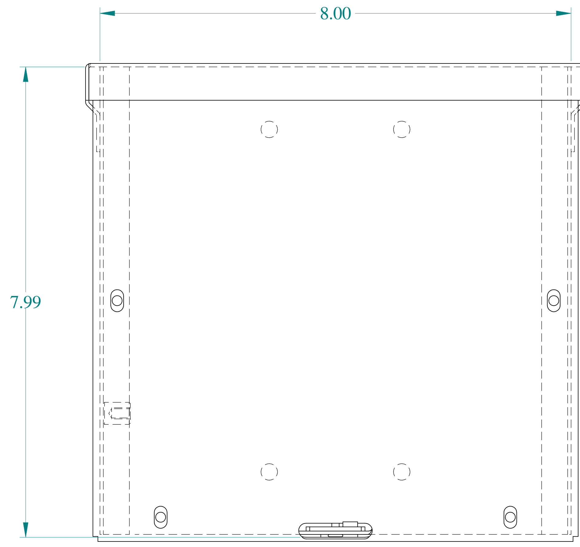
FRONT VIEW
