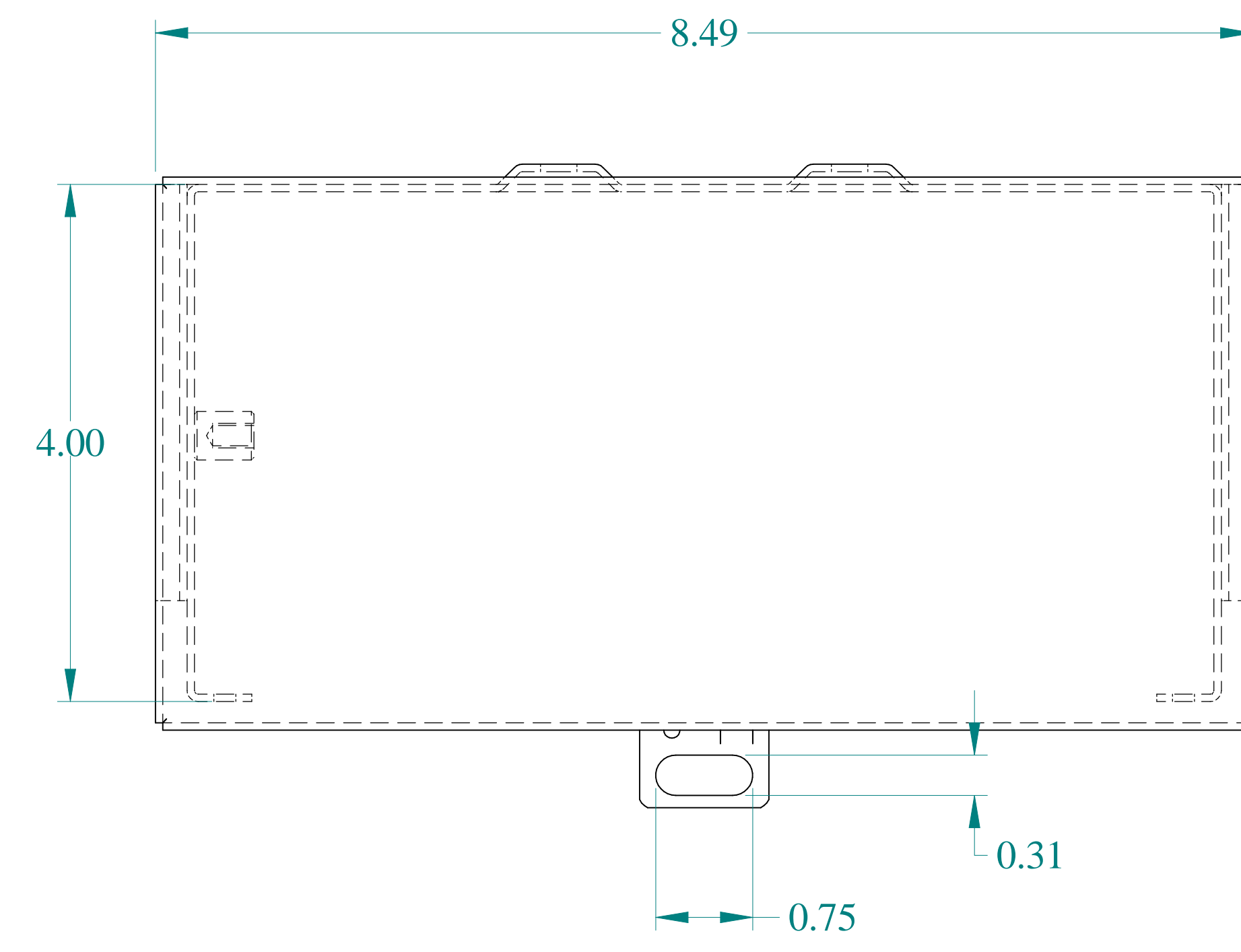
TOP VIEW
