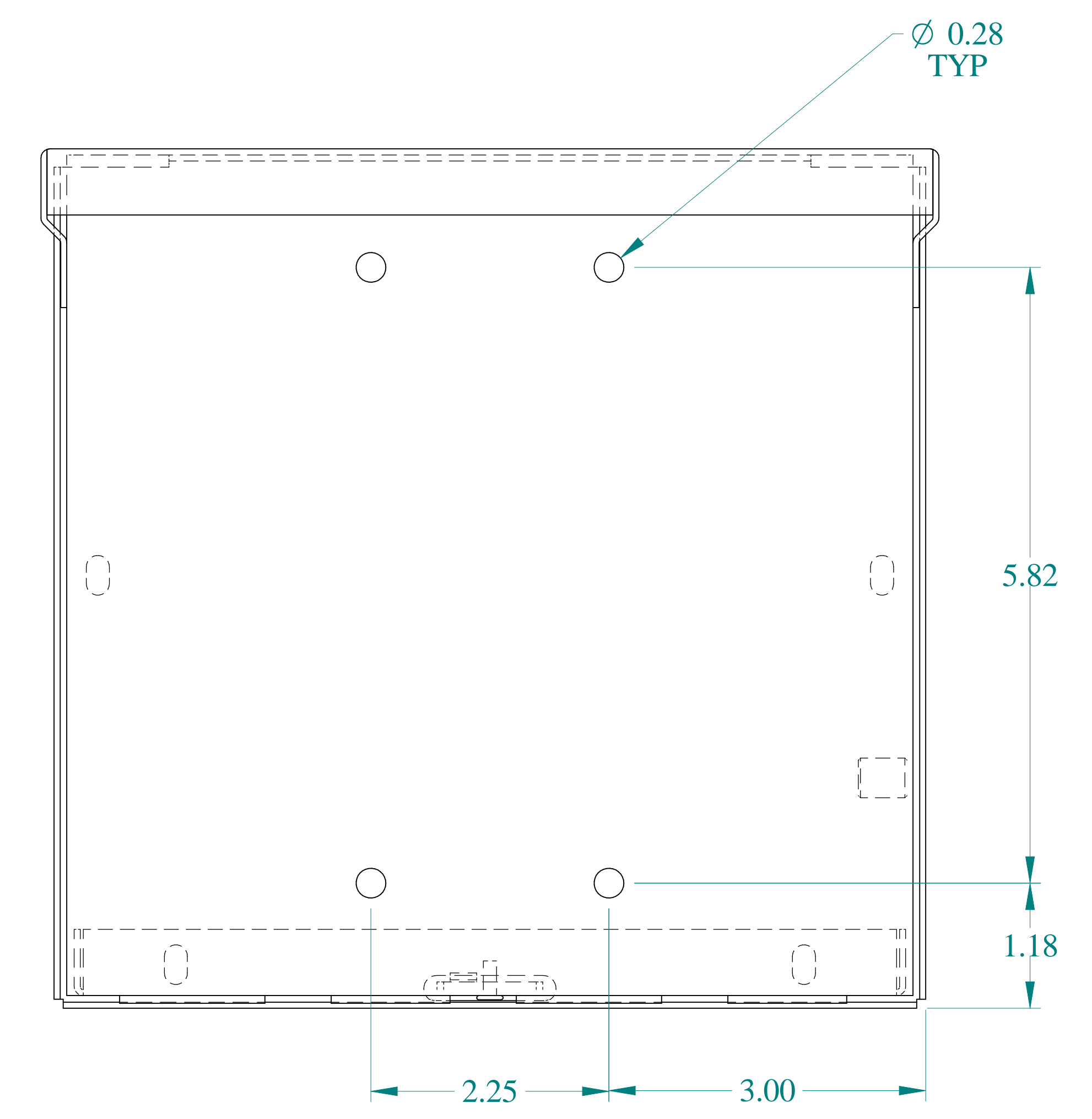
BACK VIEW
