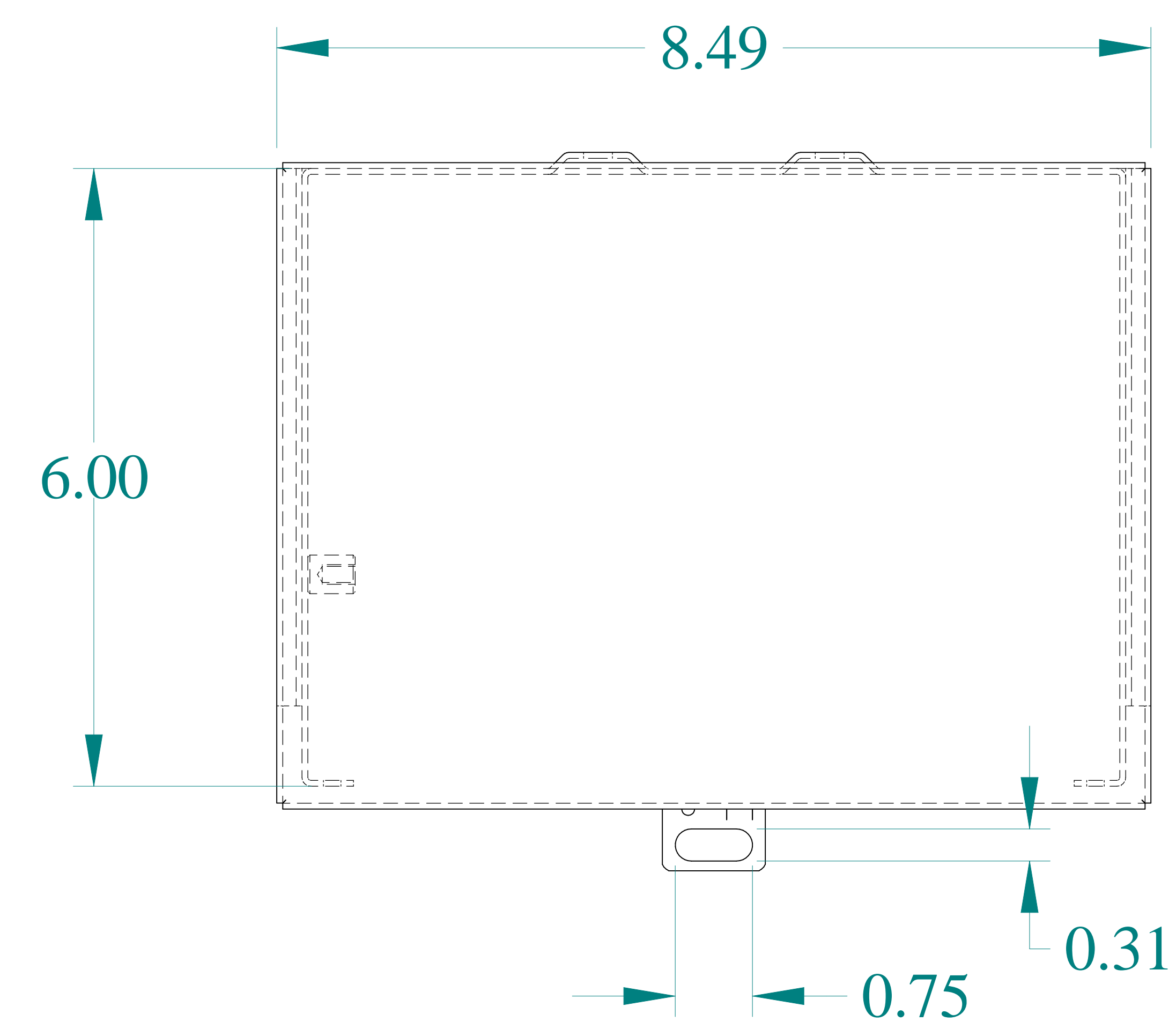
TOP VIEW
