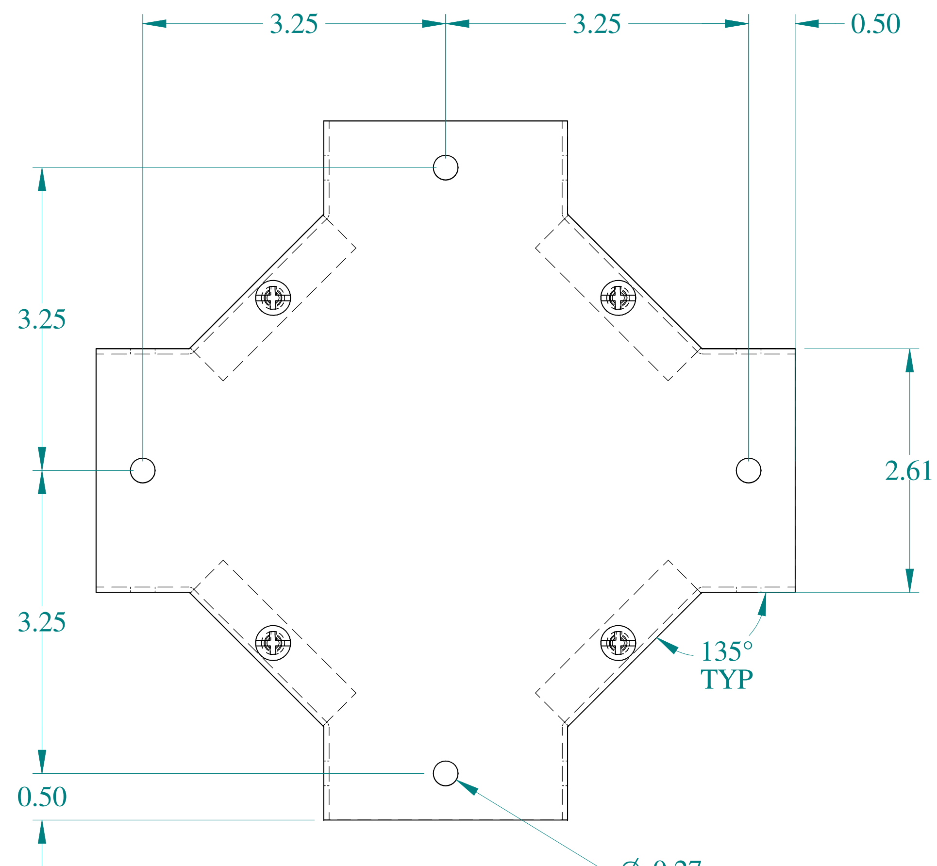
TOP VIEW
