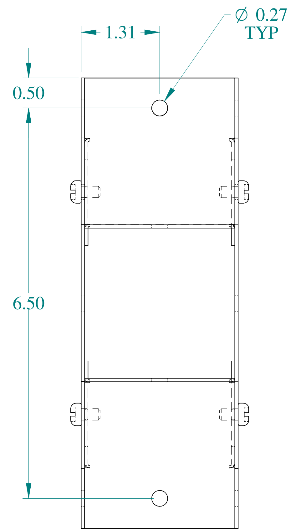
SIDE VIEW
