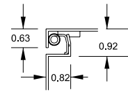
Cross Section of 14 gauge Body & Door
