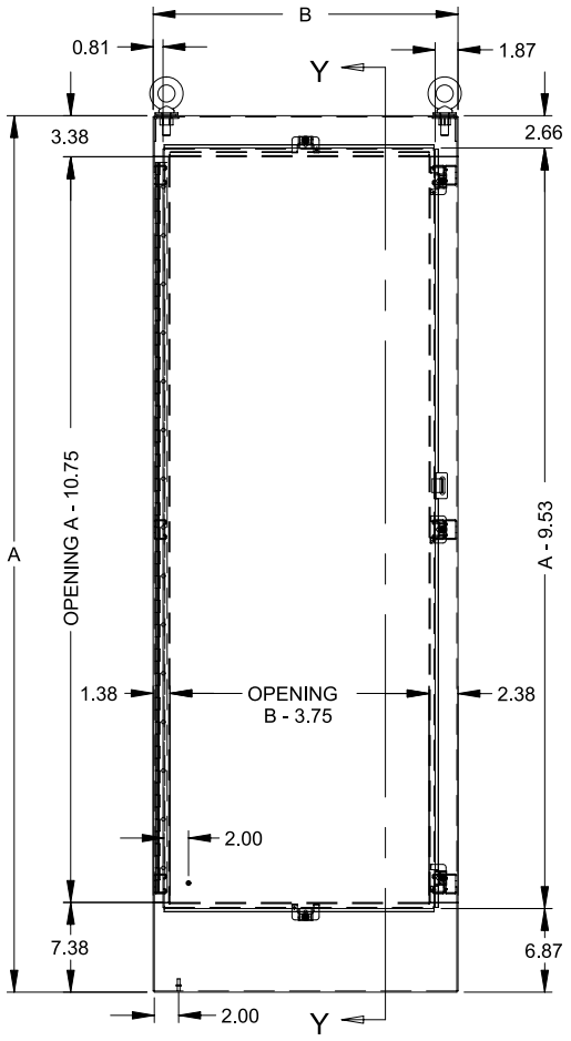
Front View
