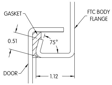
FTC Detail
