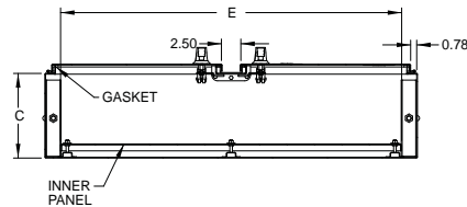
SECTION X-X
