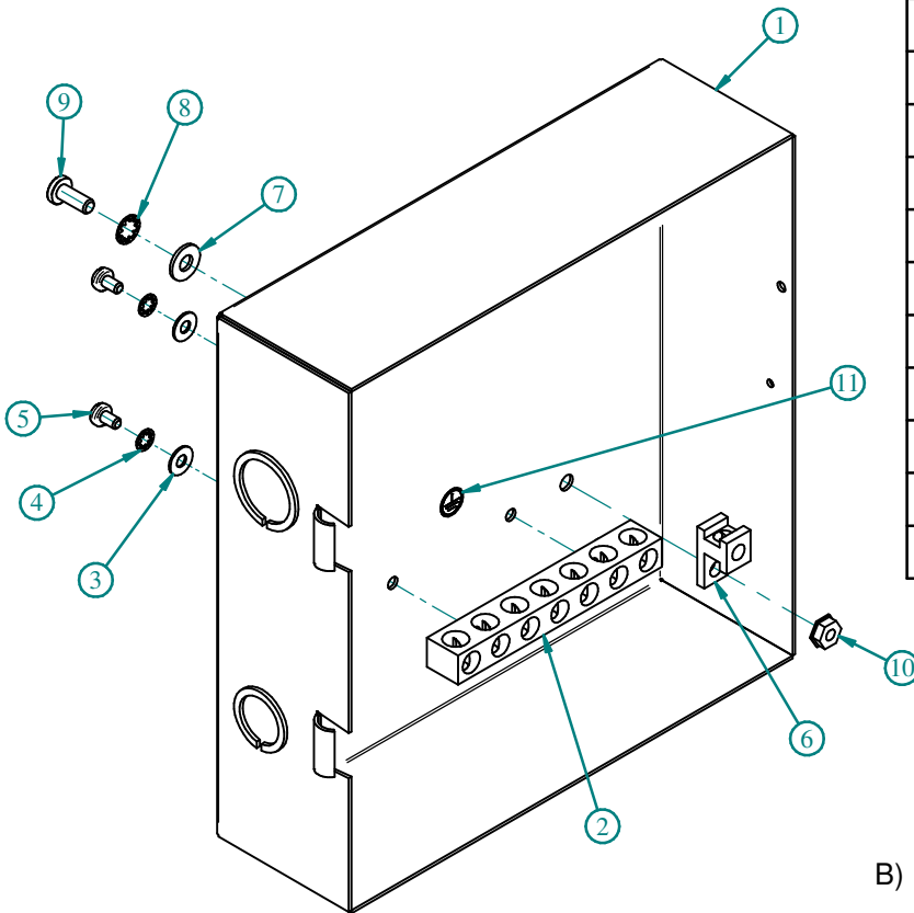
EXPLODED - ISOMETRIC VIEW
