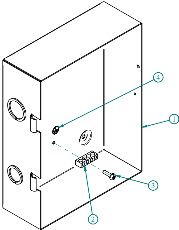
EXPLODED - ISOMETRIC VIEW
