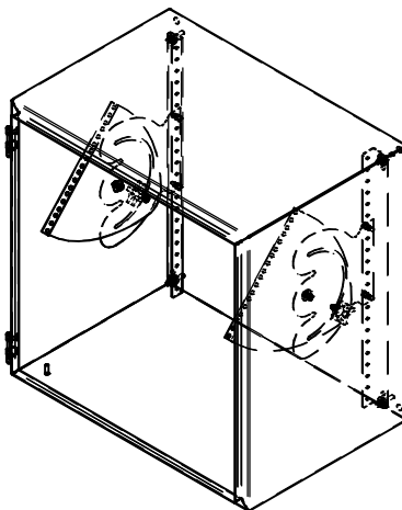
ERP MOUNTED INSIDE ECLIPSE (SHOWN WITH HLP6UR RAILS)
