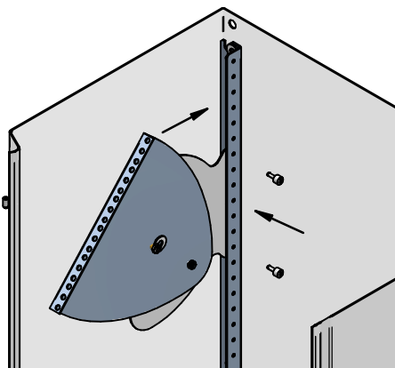
SHOWN MOUNTING TO ECLIPSE SERIES
