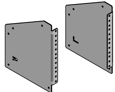
FIXED RAILS 1:6
