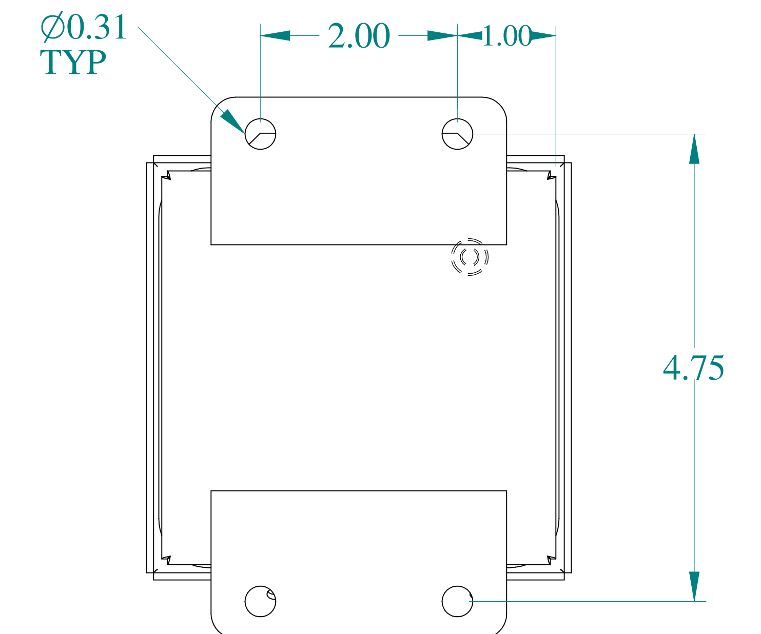
BACK VIEW
