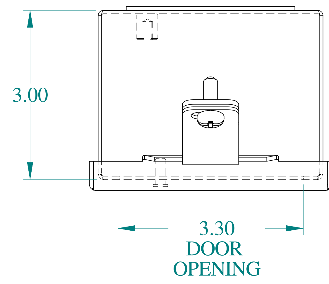
TOP VIEW
