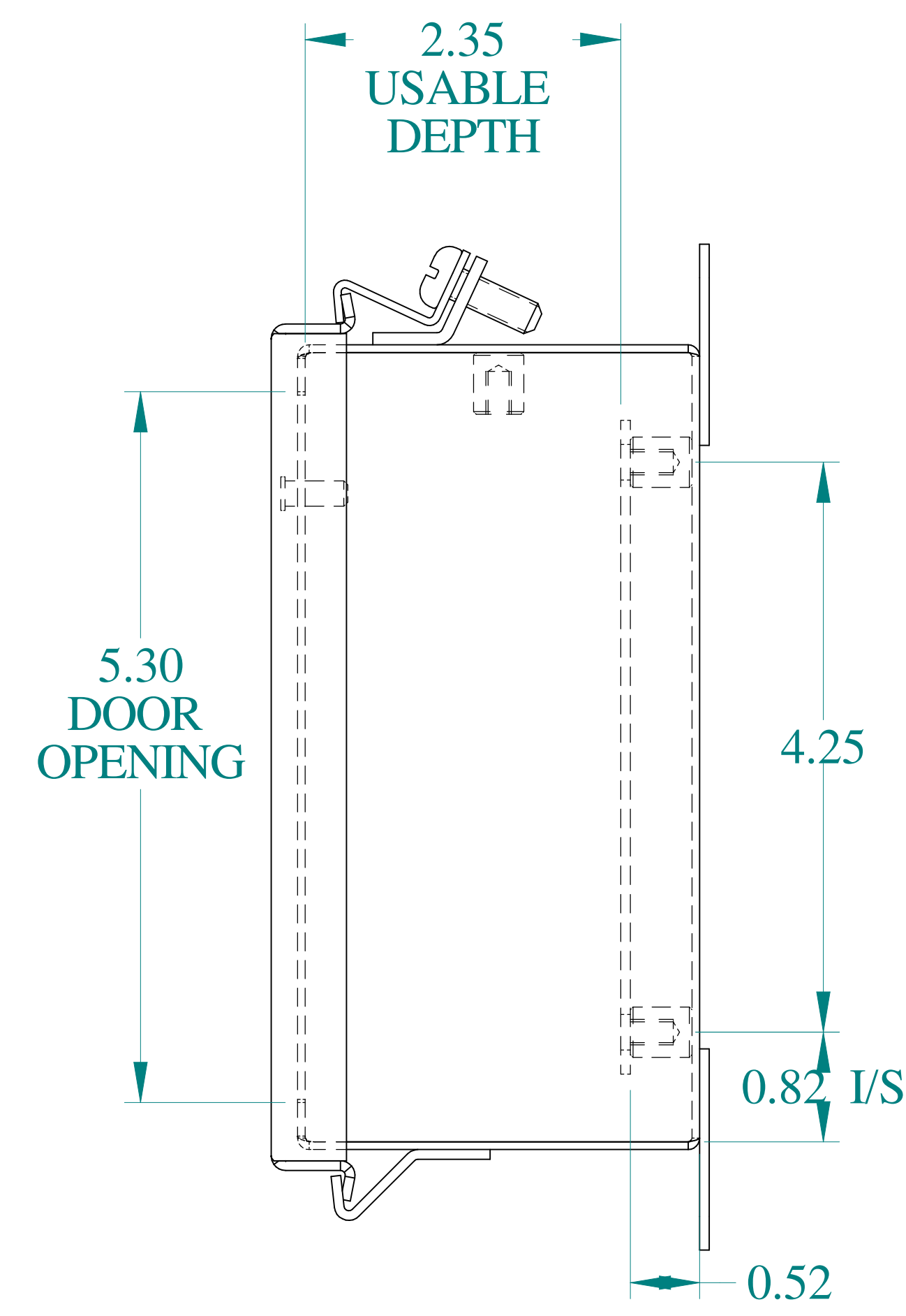
SIDE VIEW
