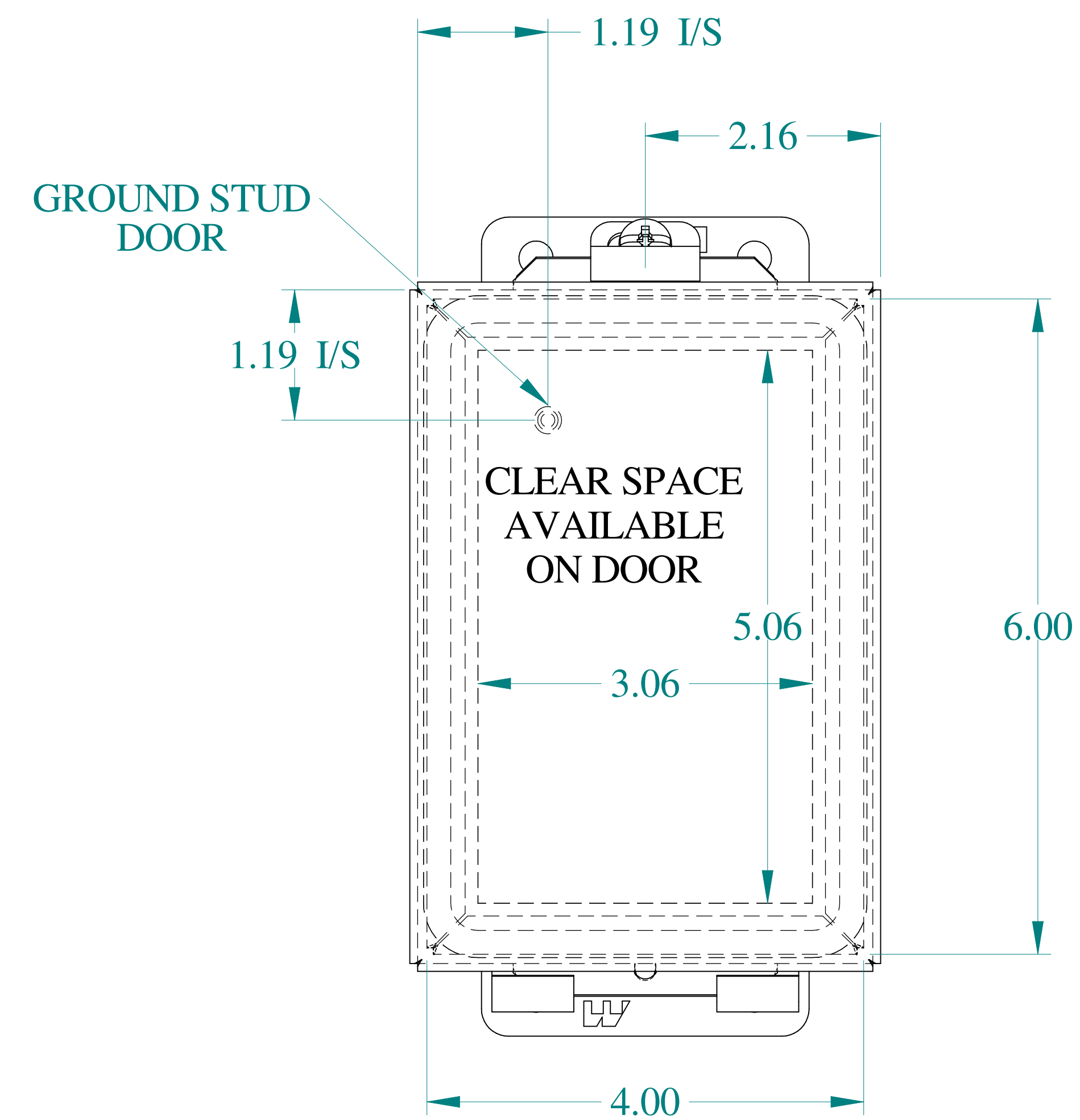
FRONT VIEW
