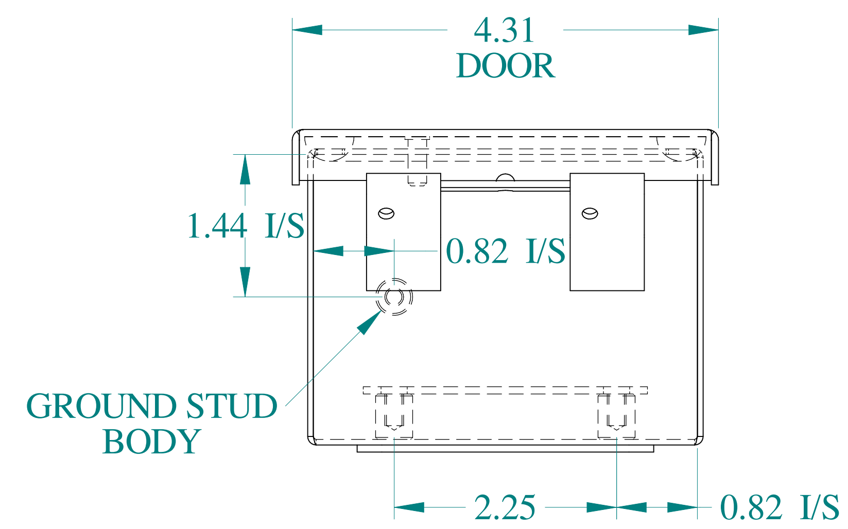
BOTTOM VIEW
