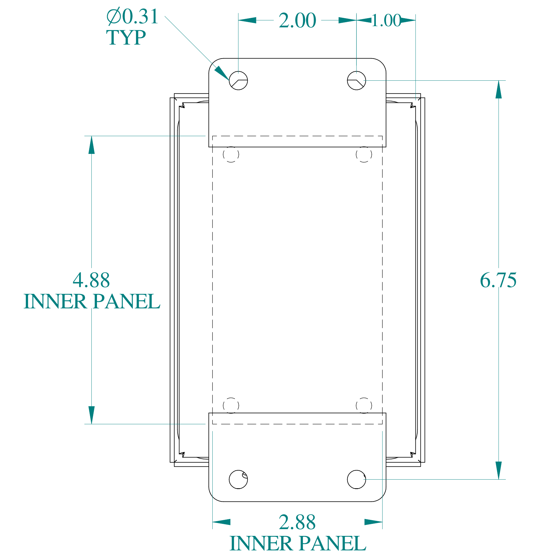
BACK VIEW
