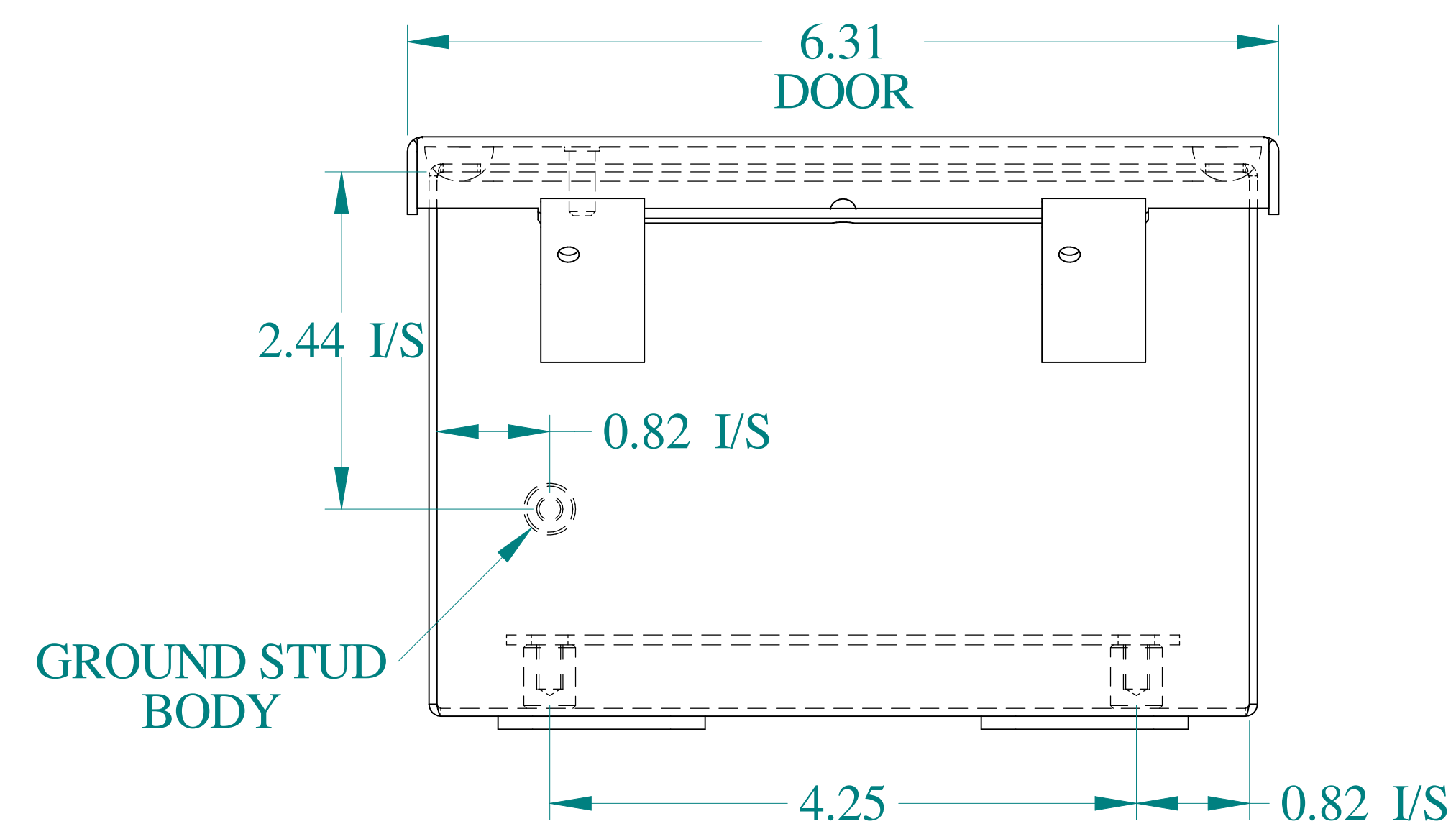
BOTTOM VIEW
