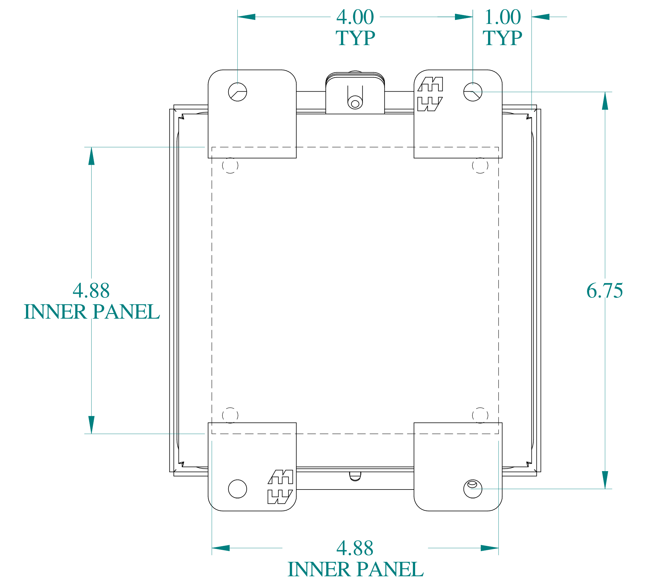
BACK VIEW
