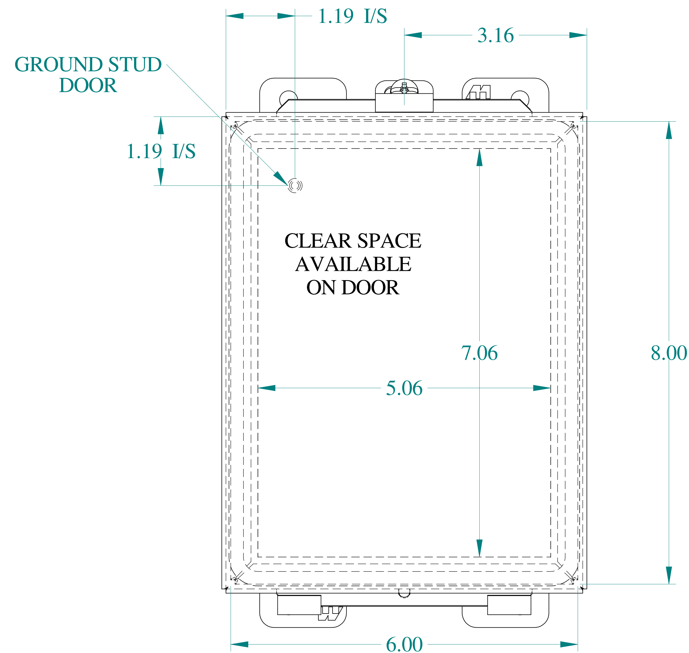
FRONT VIEW
