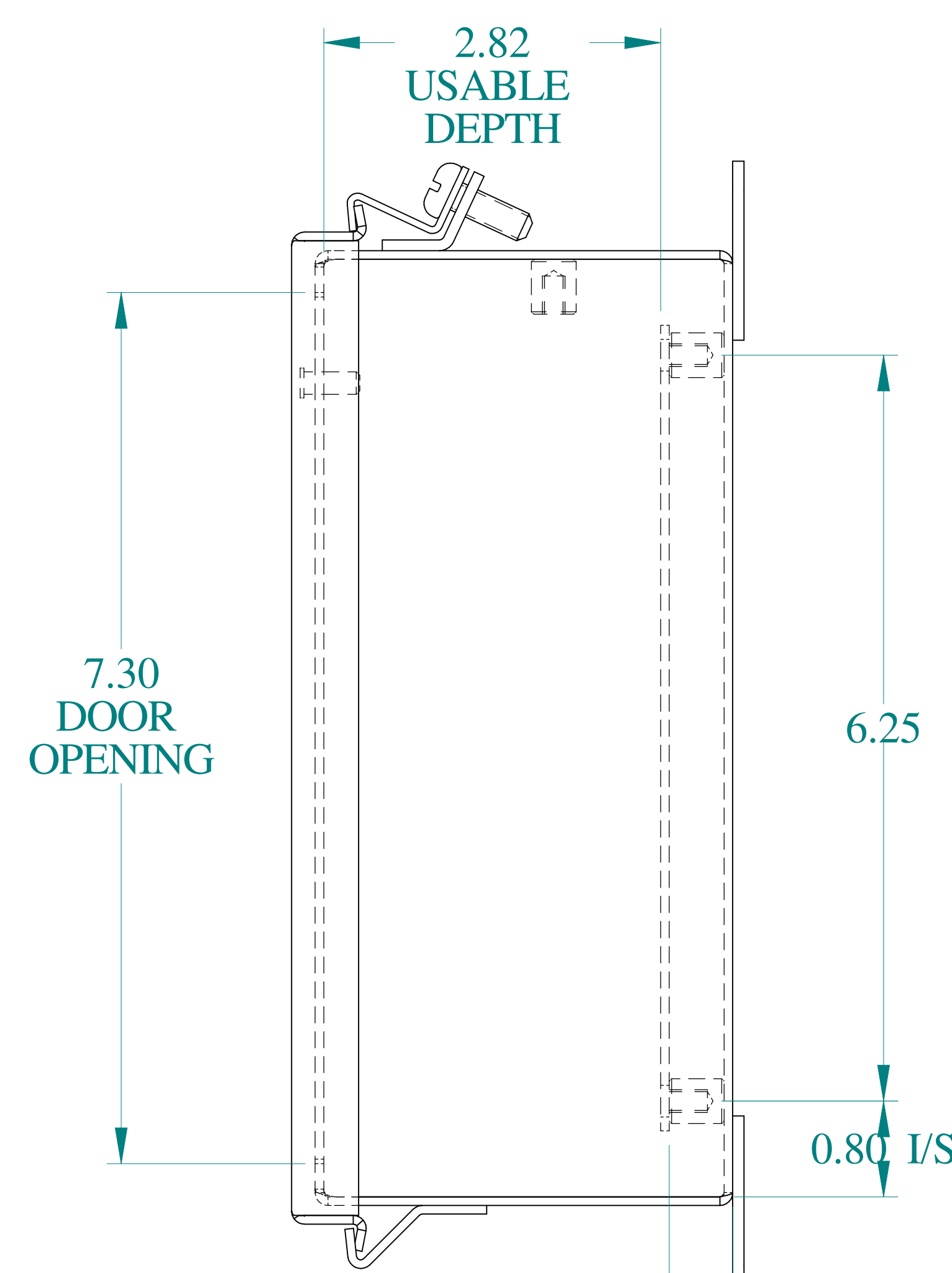
SIDE VIEW
