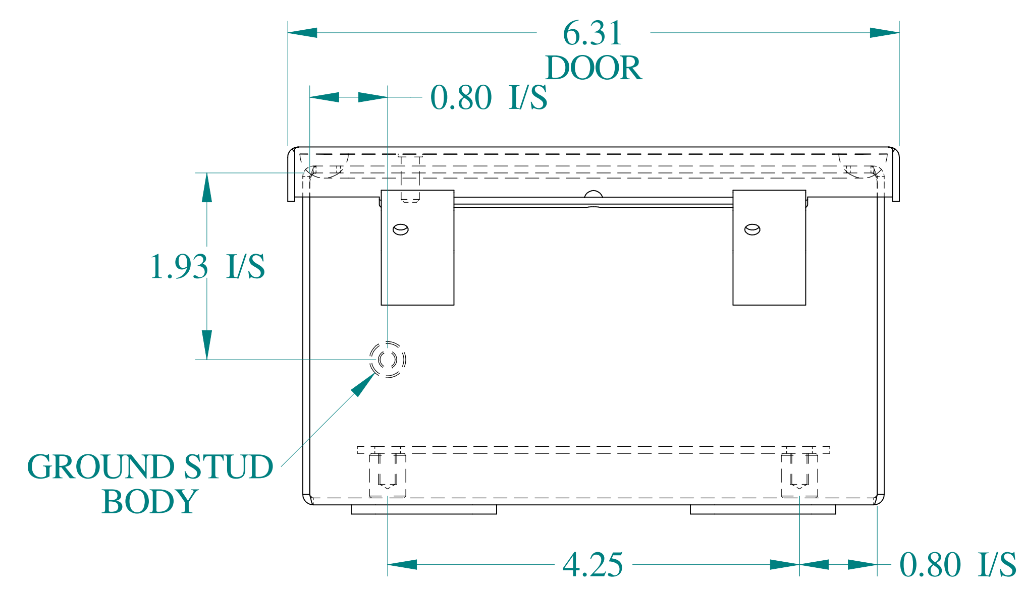
BOTTOM VIEW
