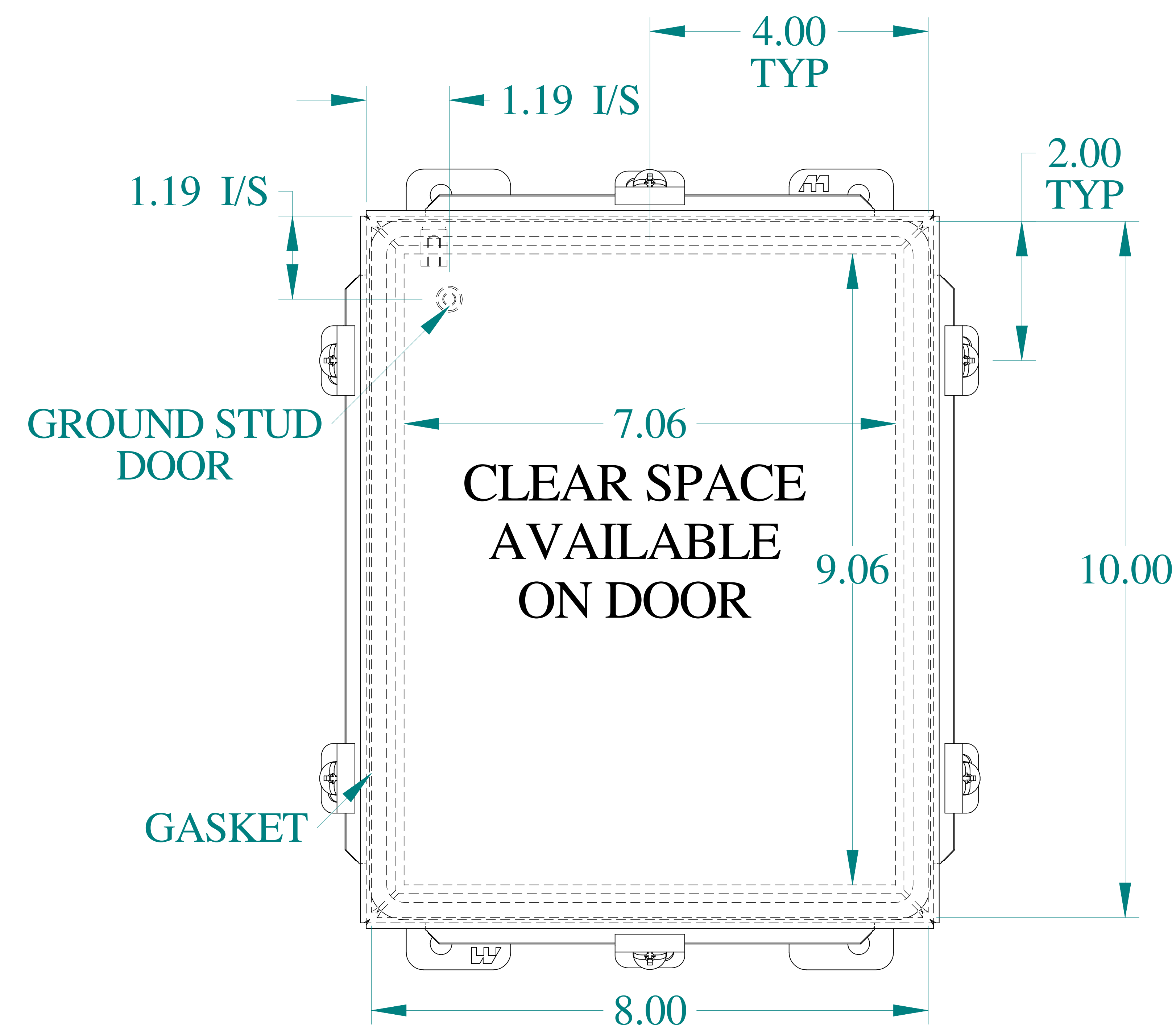
FRONT VIEW
