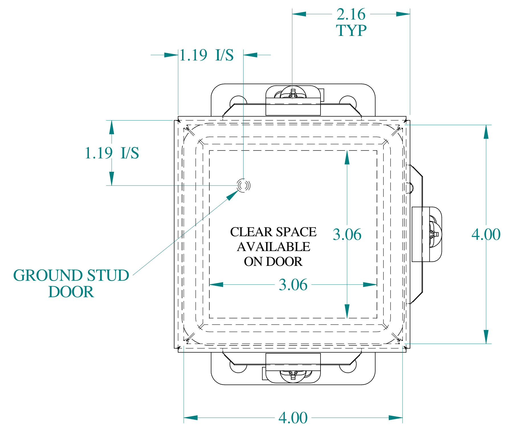
FRONT VIEW
