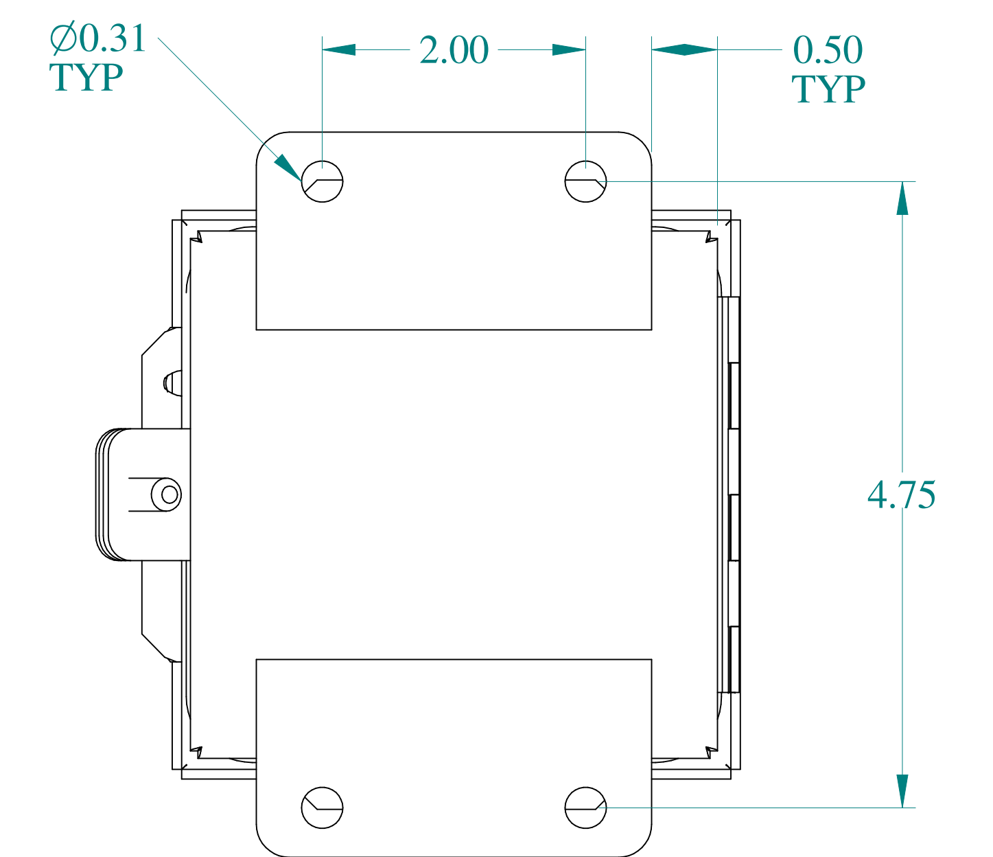
BACK VIEW
