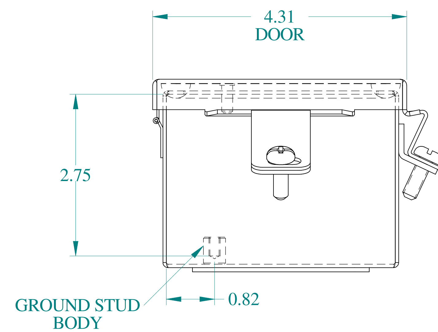
BOTTOM VIEW
