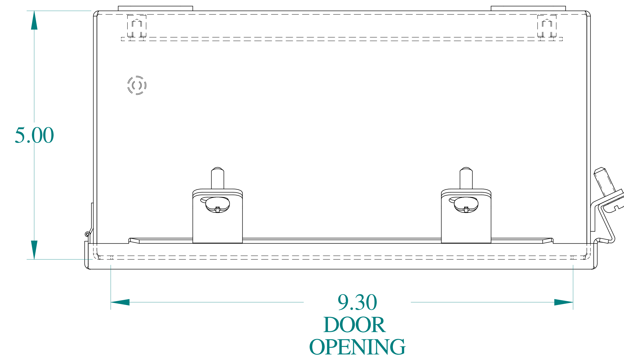
TOP VIEW
