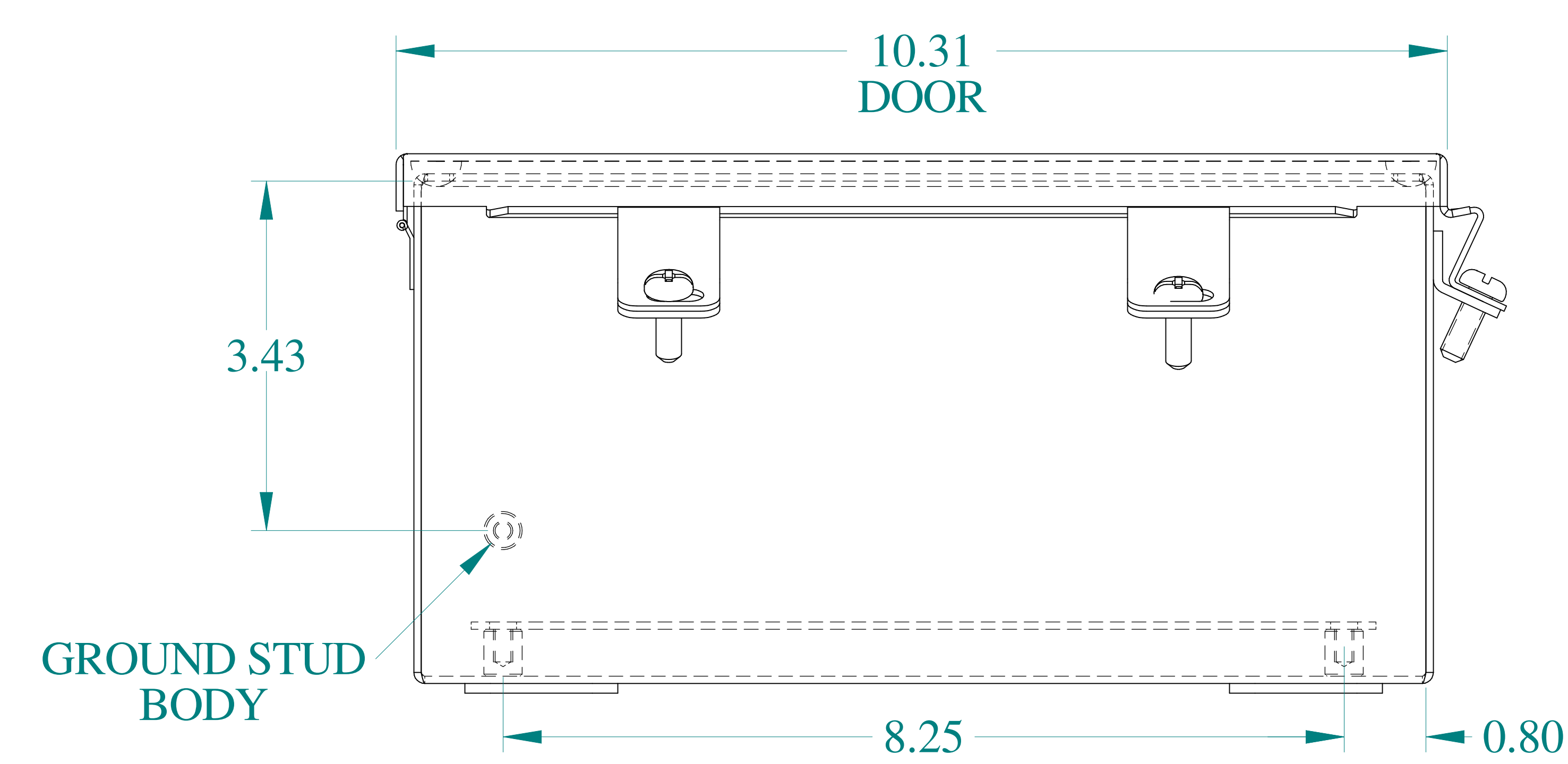
BOTTOM VIEW
