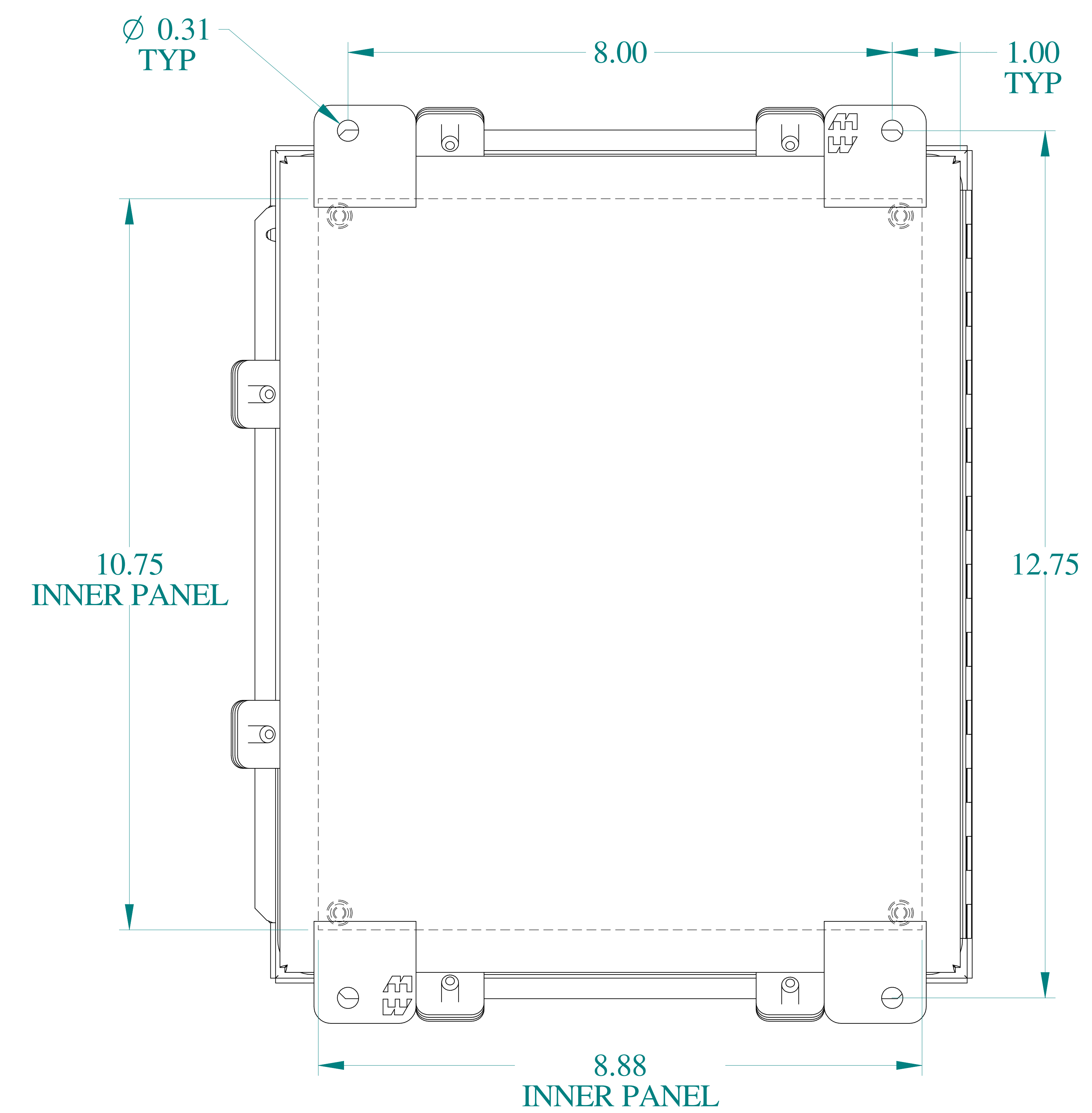
BACK VIEW
