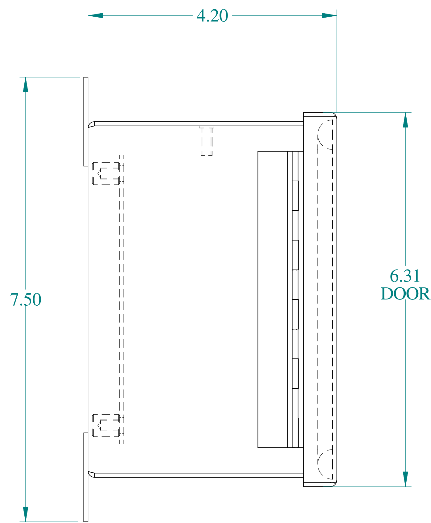
SIDE VIEW
