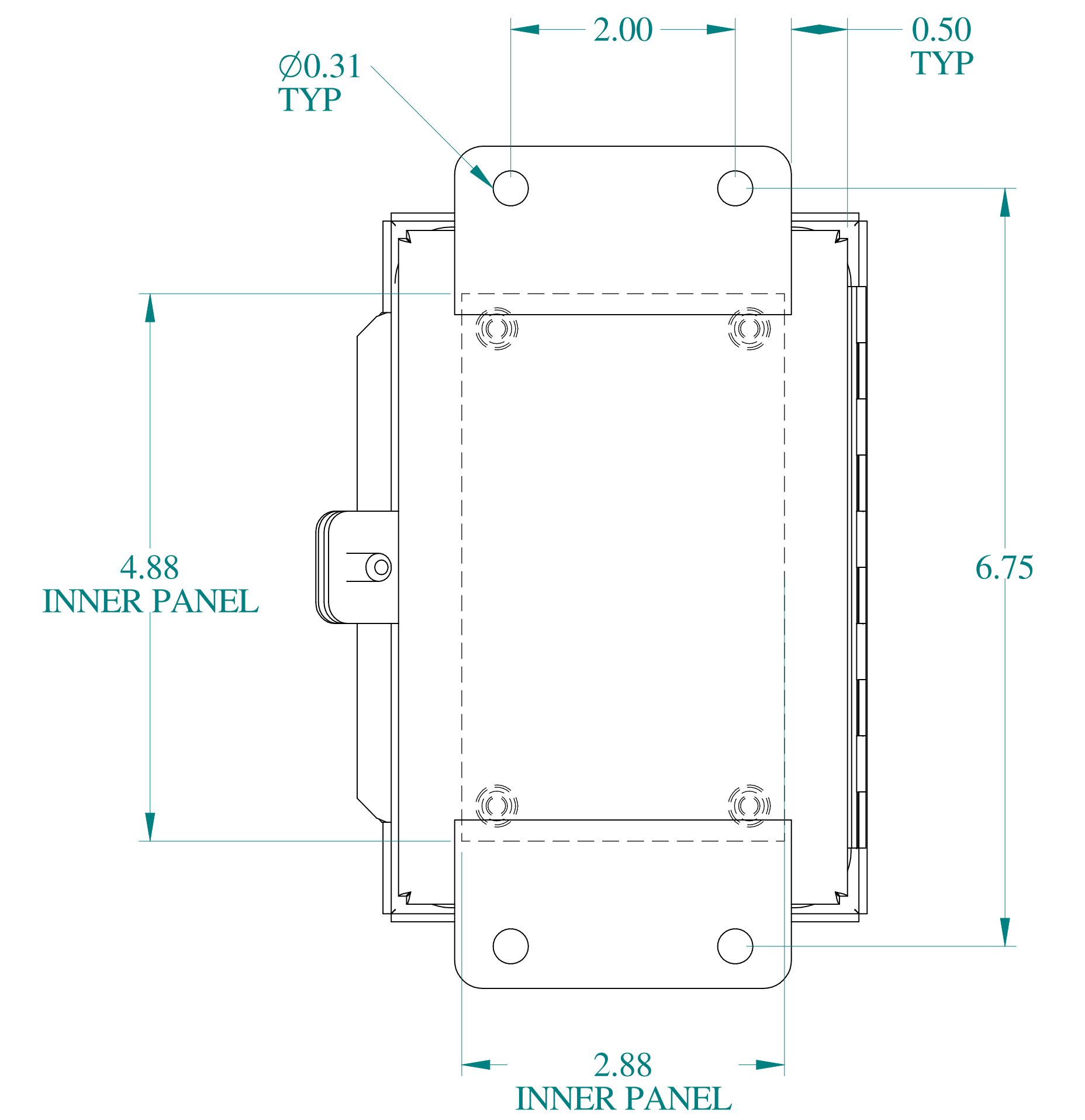
BACK VIEW
