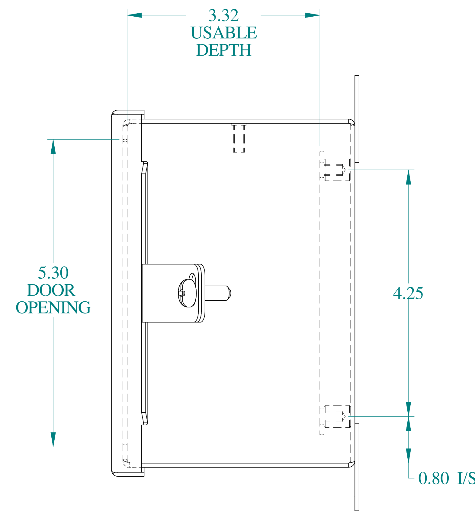
SIDE VIEW
