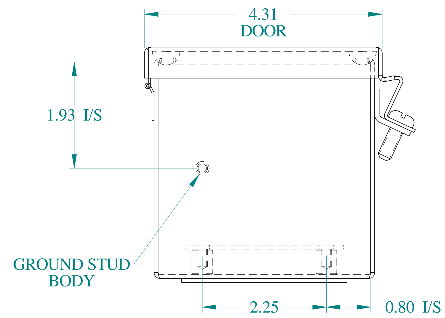
BOTTOM VIEW
