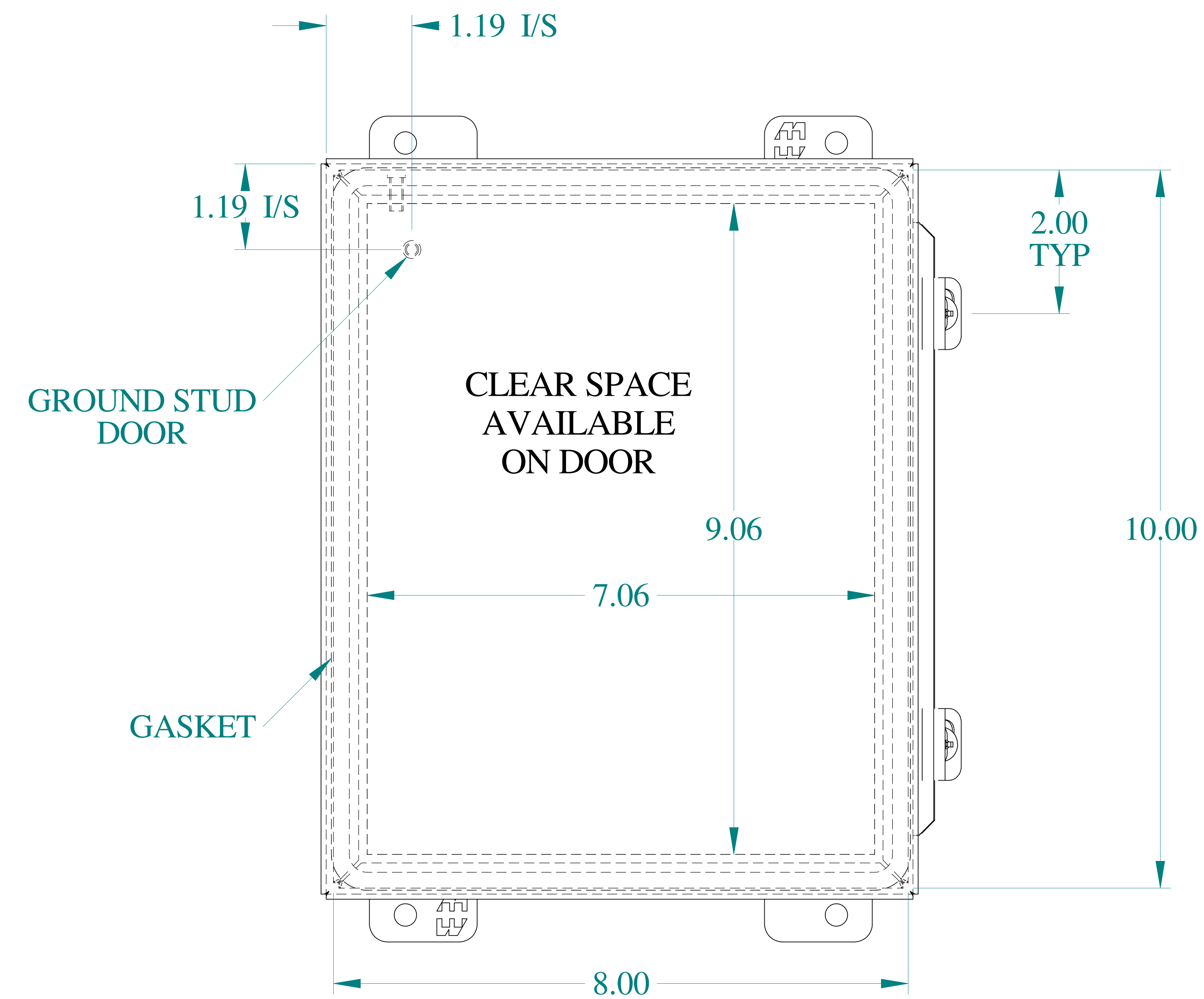
FRONT VIEW
