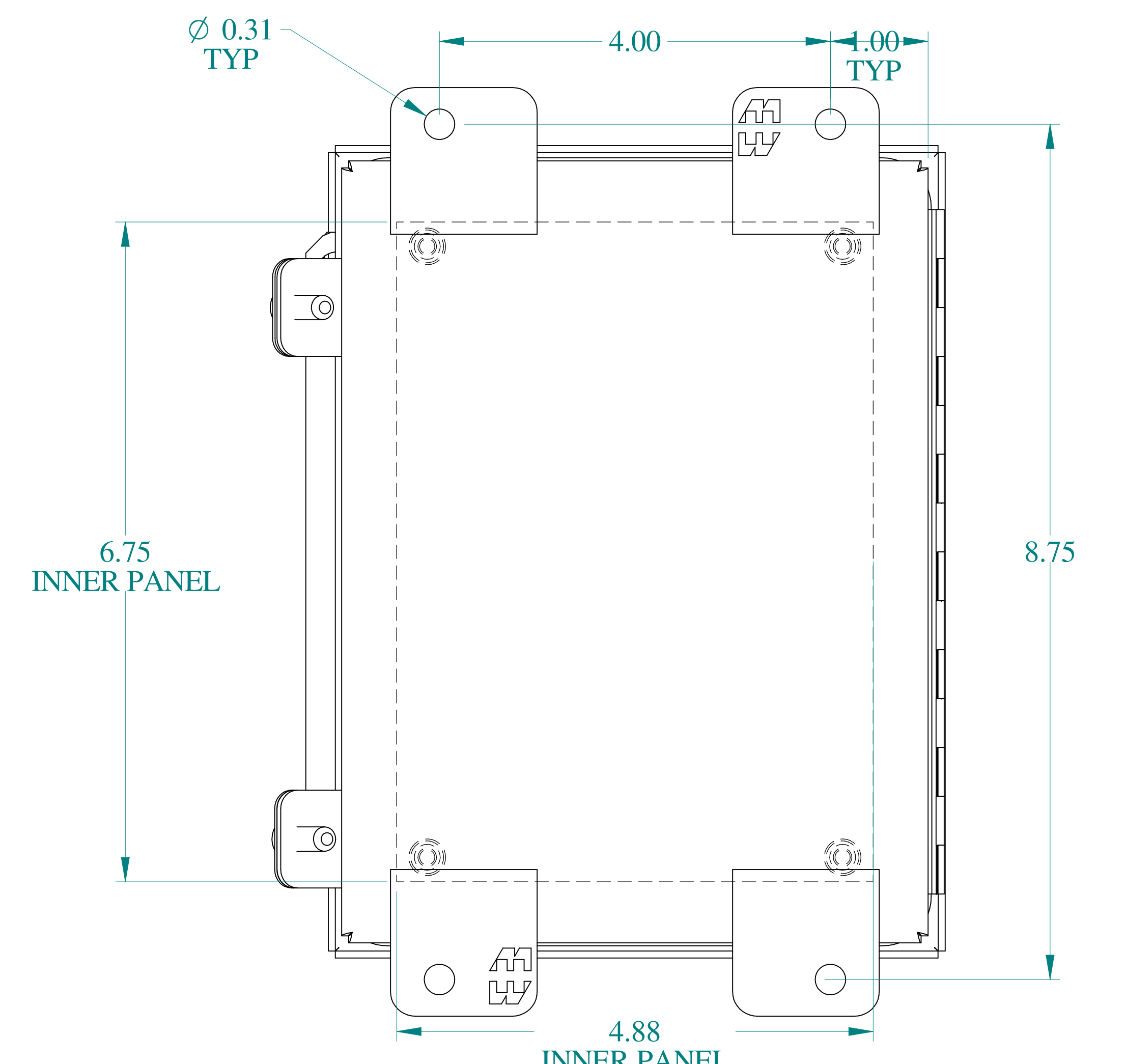
BACK VIEW
