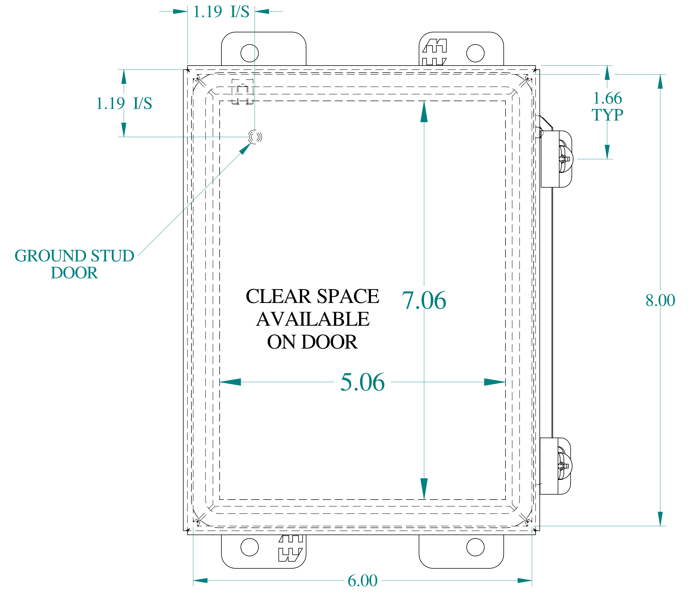
FRONT VIEW
