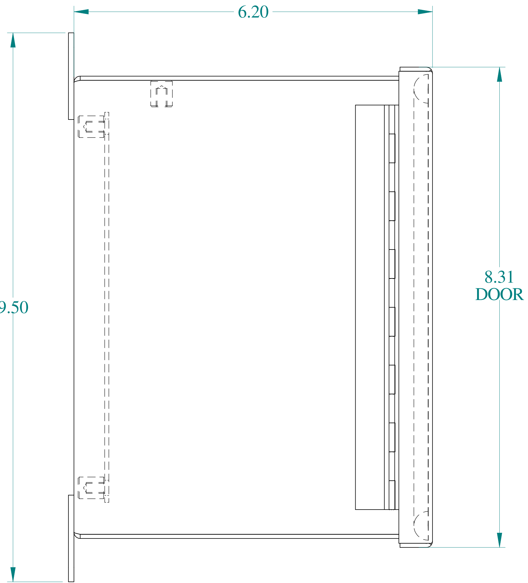
SIDE VIEW
