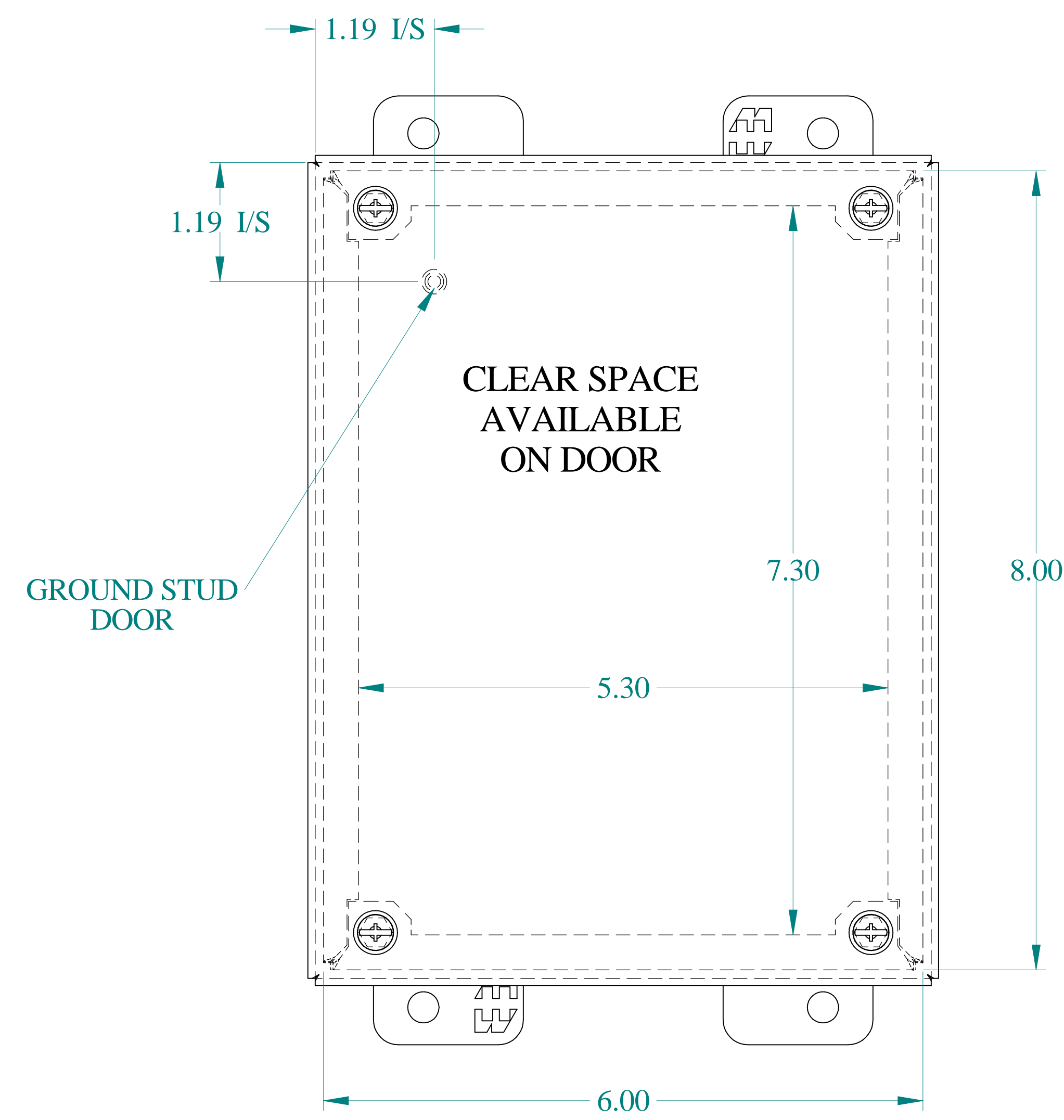
FRONT VIEW
