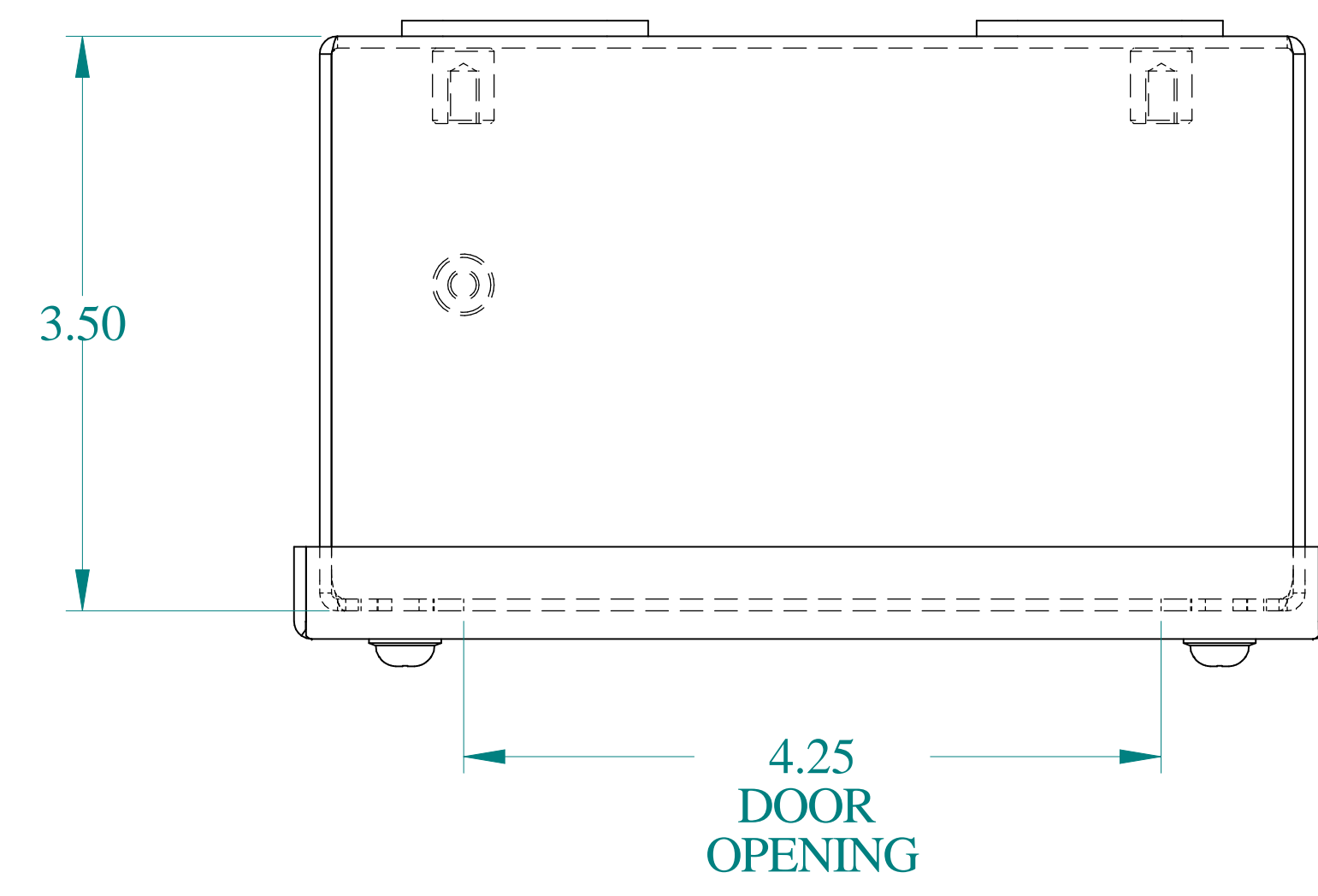
TOP VIEW
