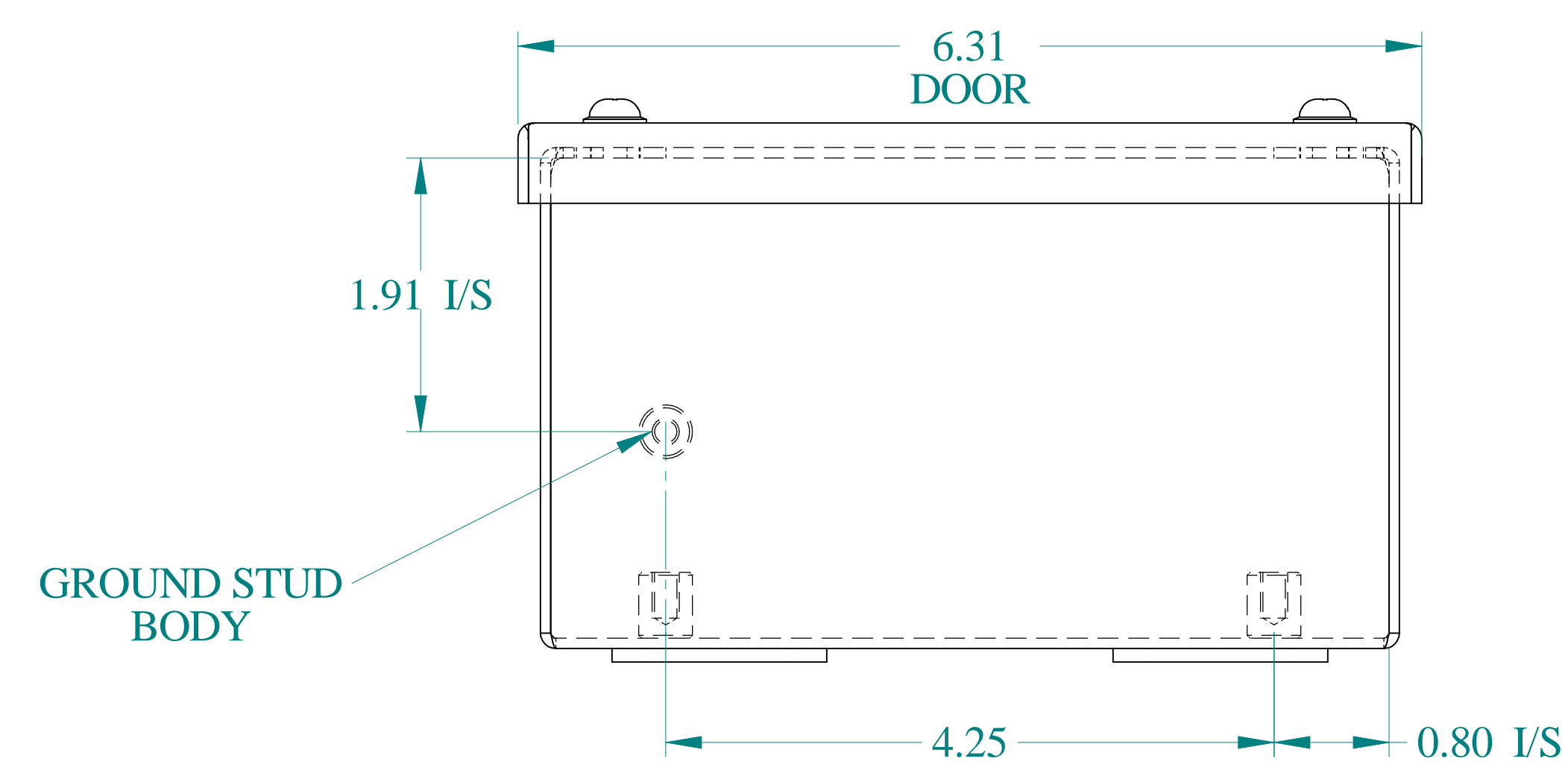
BOTTOM VIEW
