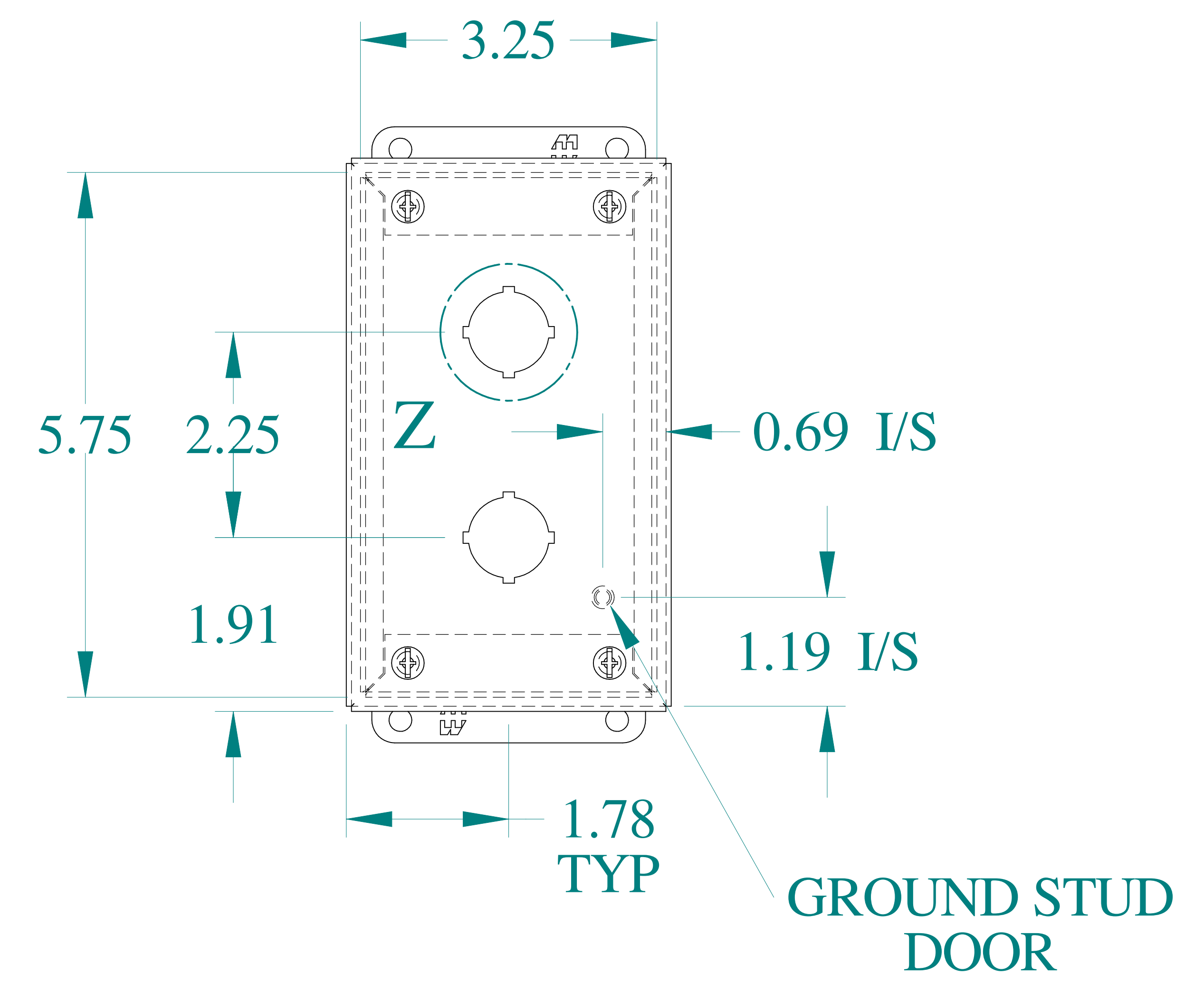
FRONT VIEW
