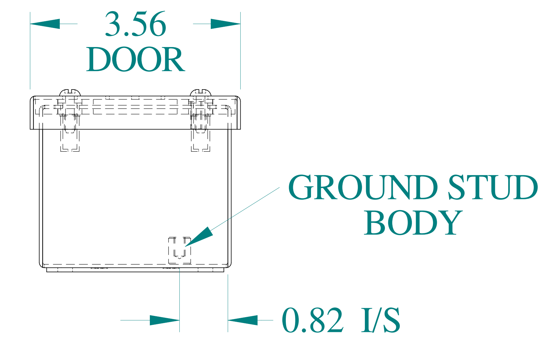
BOTTOM VIEW
