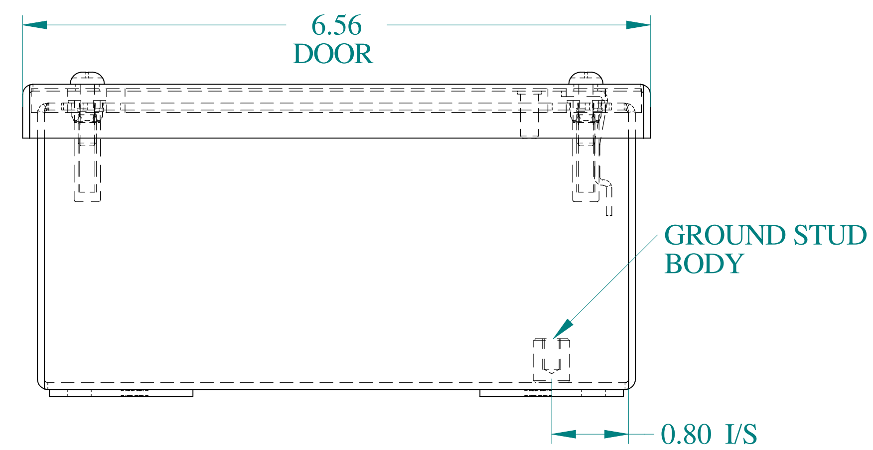
BOTTOM VIEW
