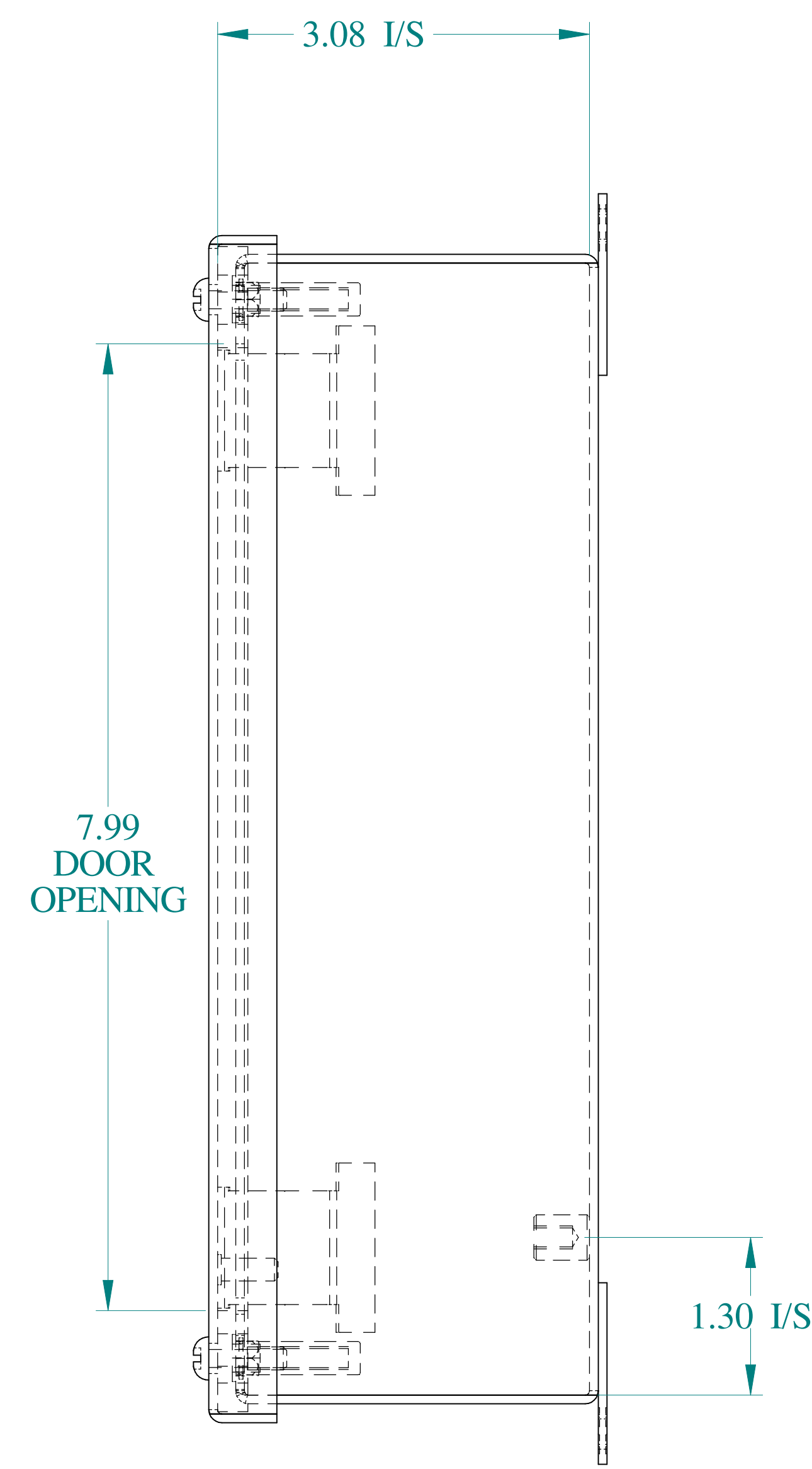
SIDE VIEW
