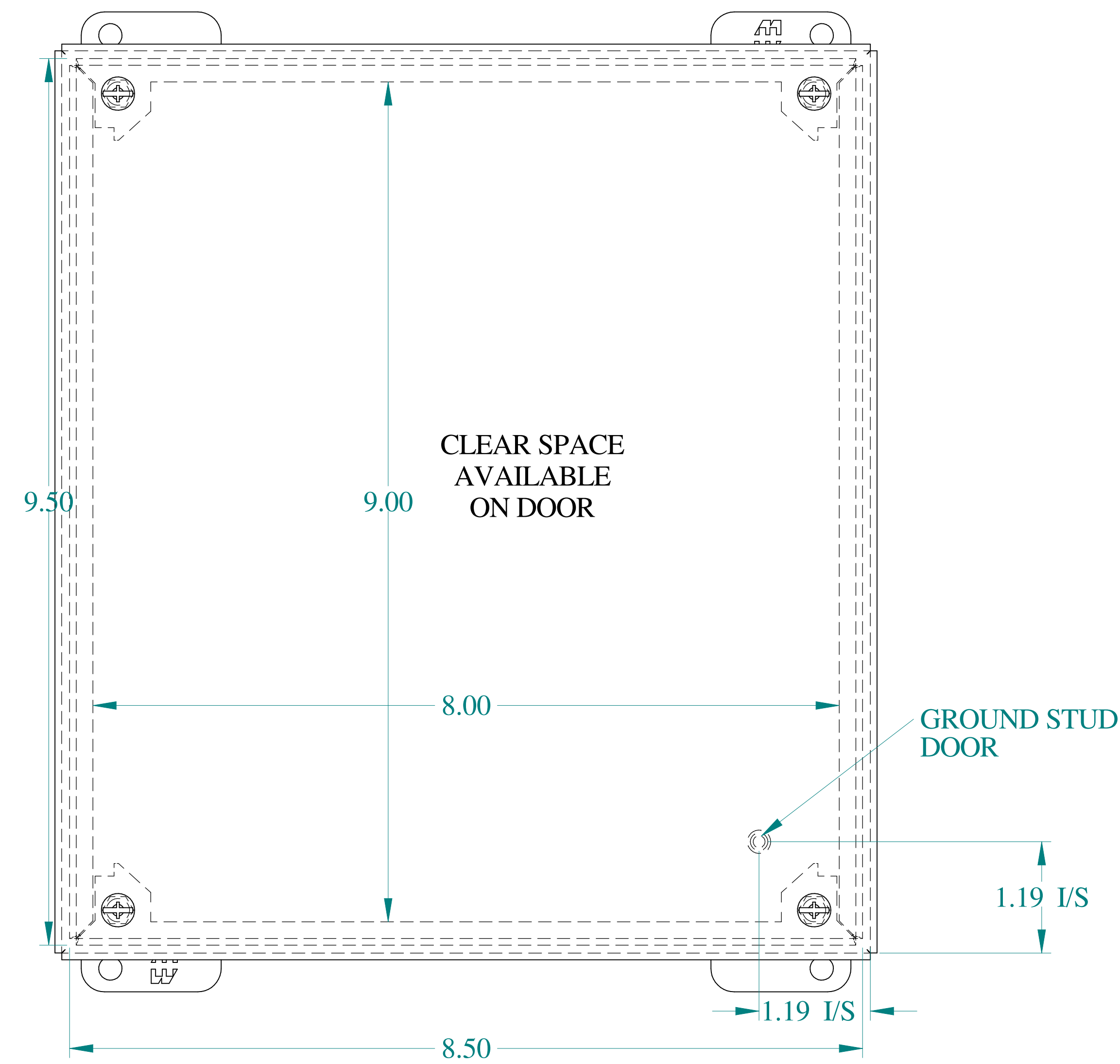
FRONT VIEW
