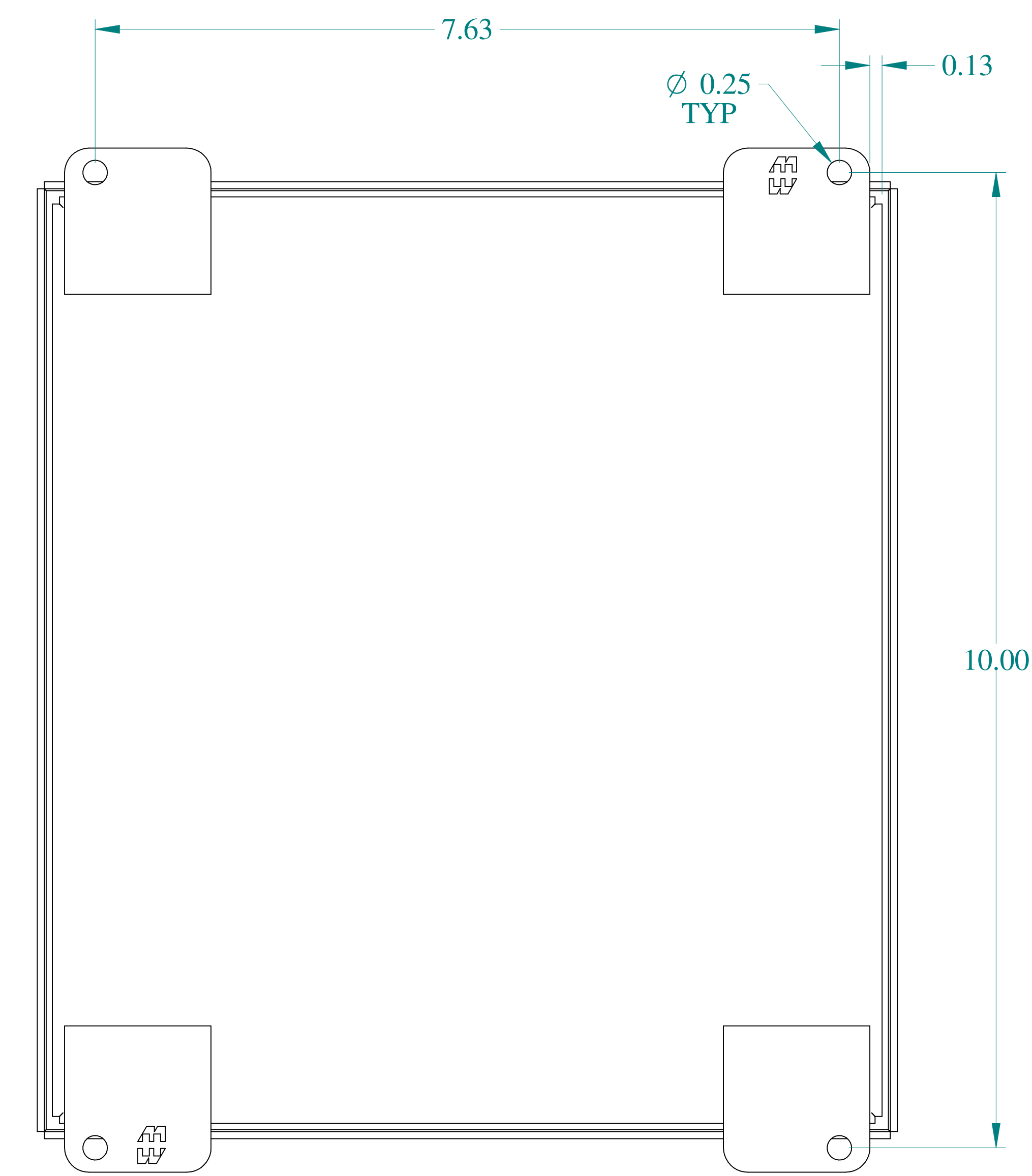
BACK VIEW
