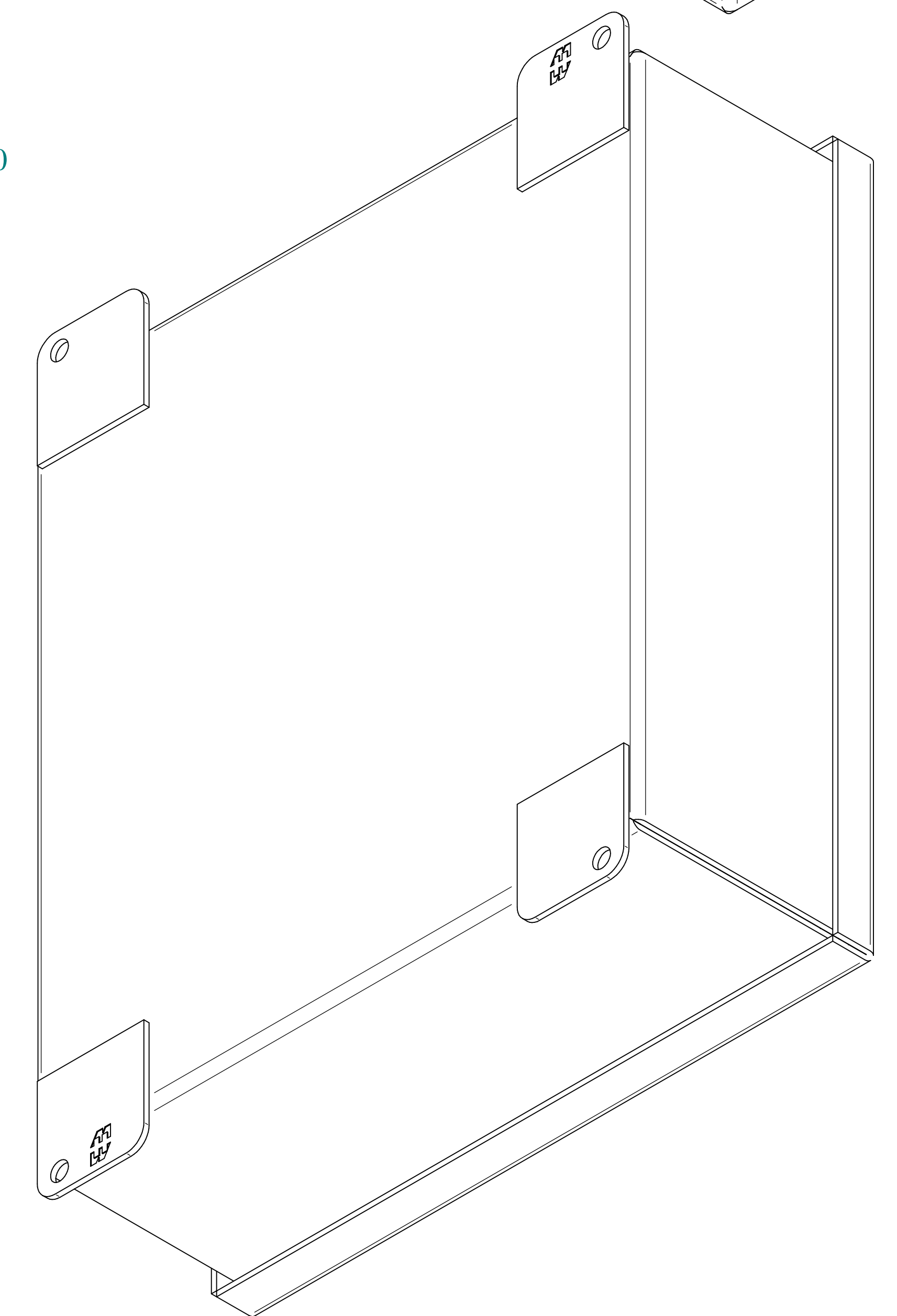
ISOMETRIC VIEWS
