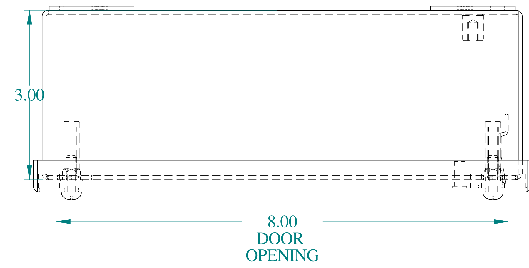
TOP VIEW
