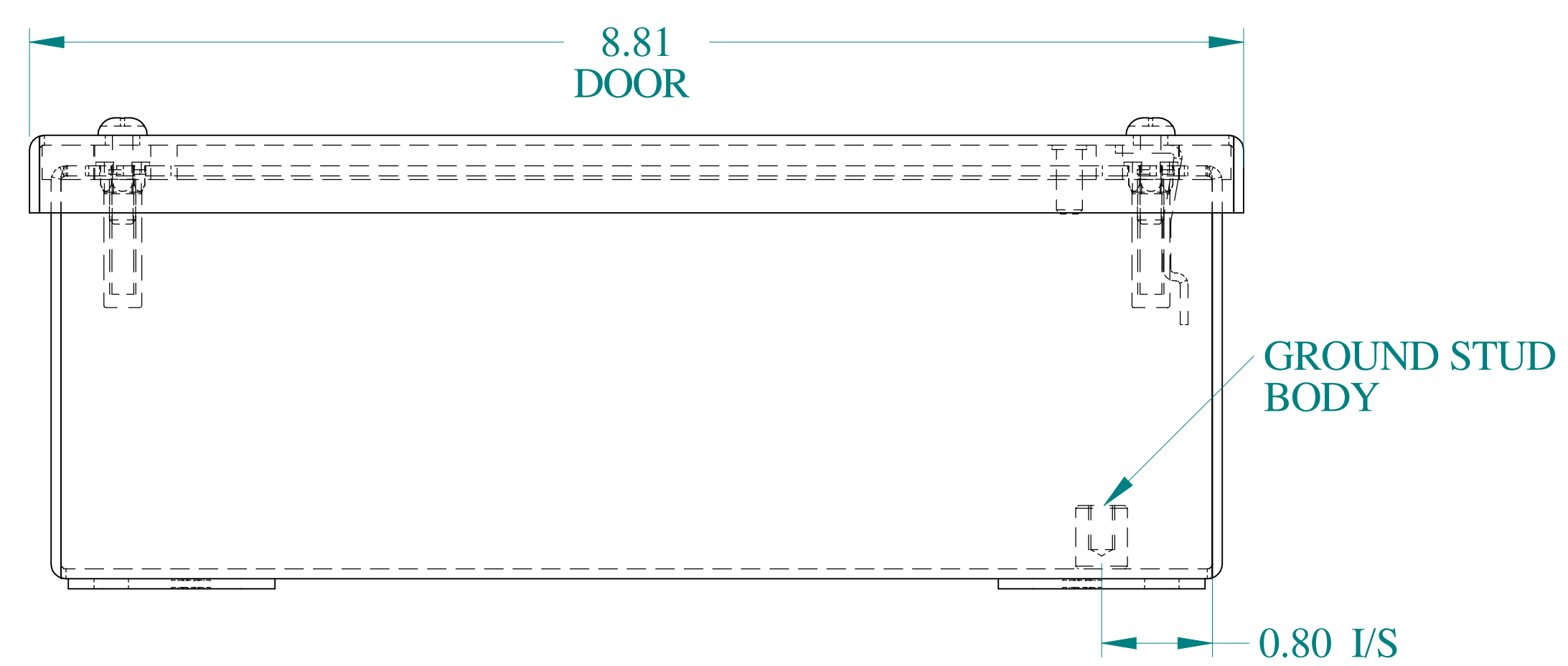
BOTTOM VIEW
