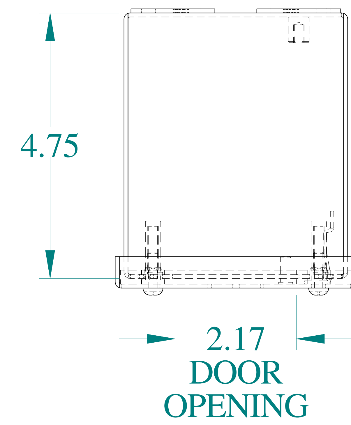
TOP VIEW
