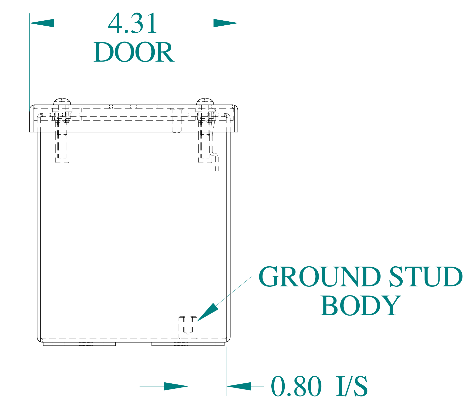
BOTTOM VIEW
