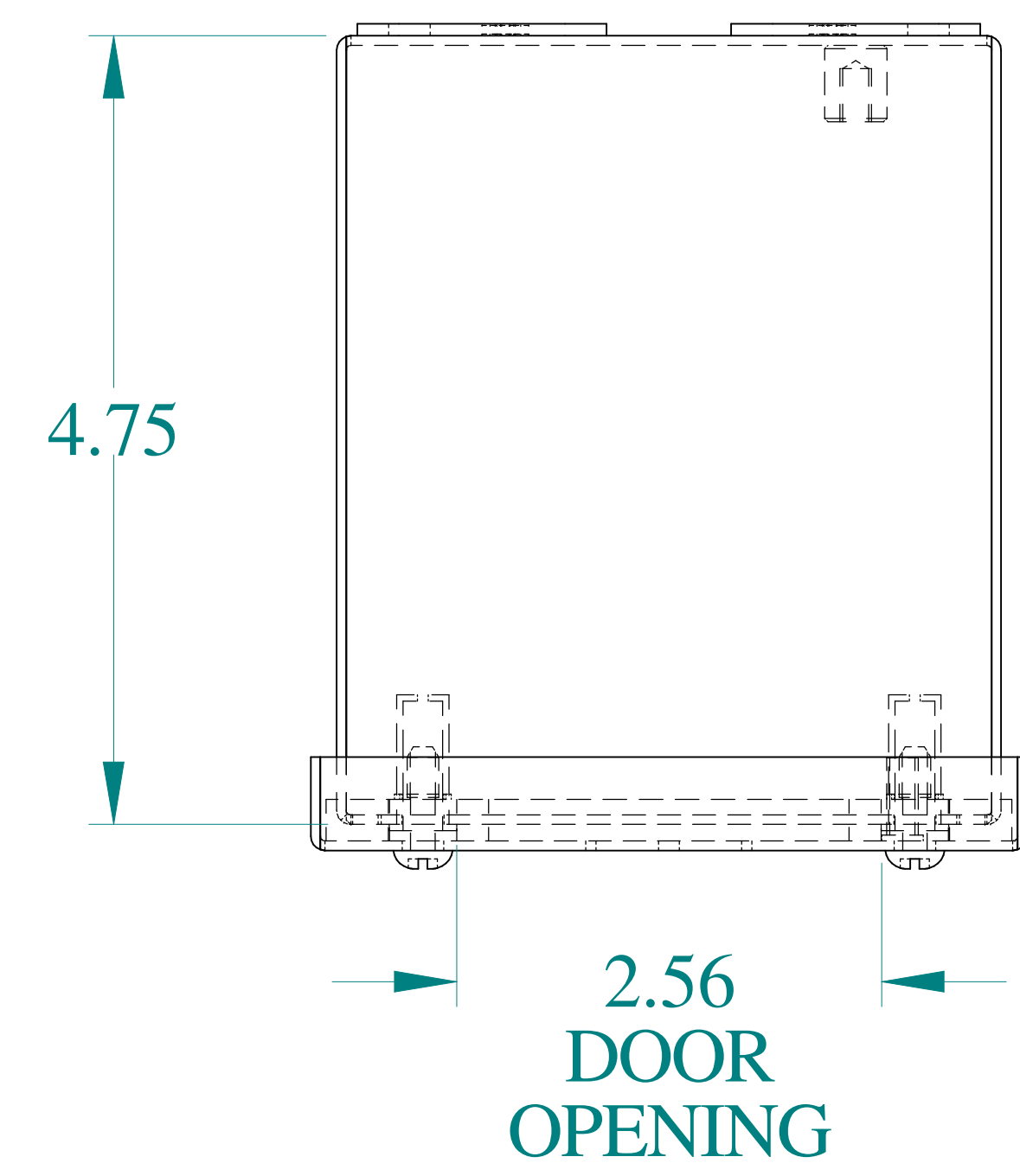
TOP VIEW
