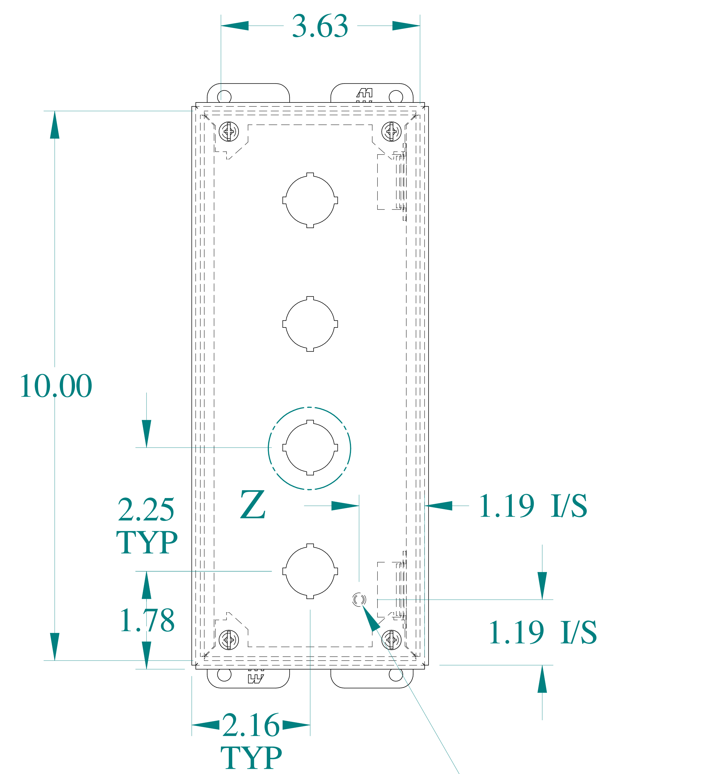
FRONT VIEW
