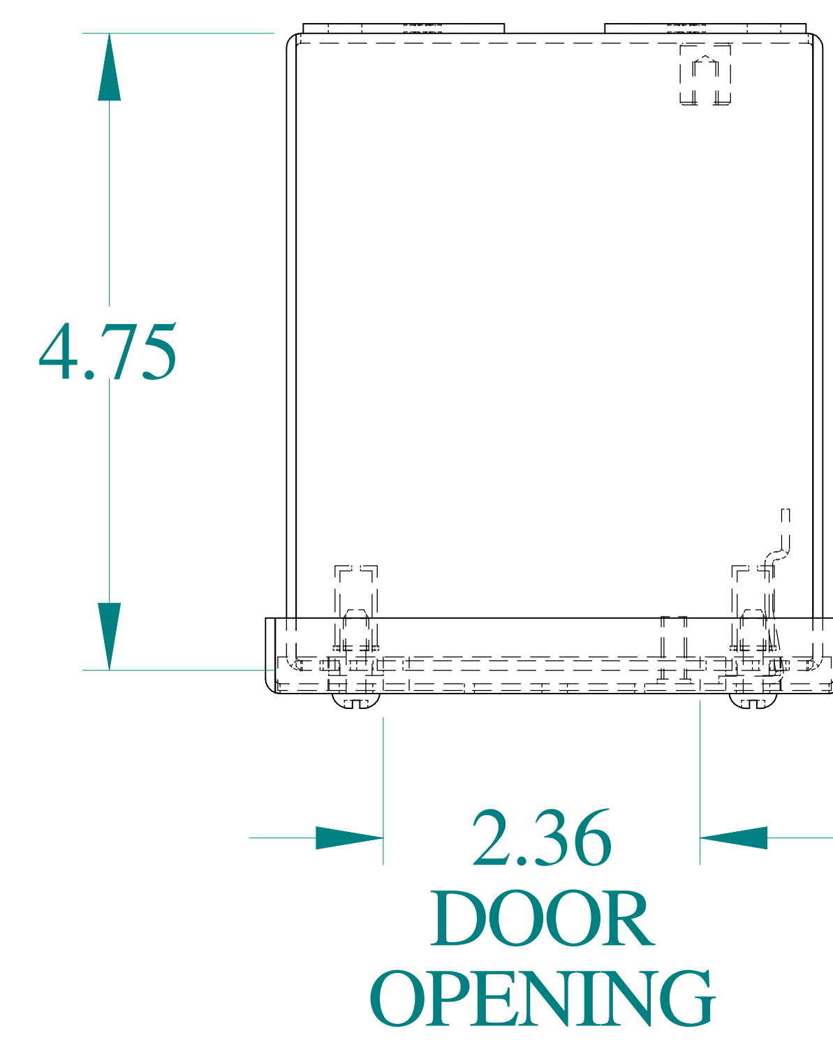
TOP VIEW
