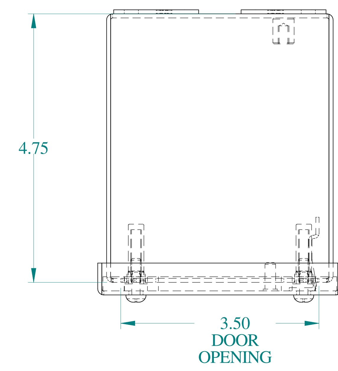
TOP VIEW
