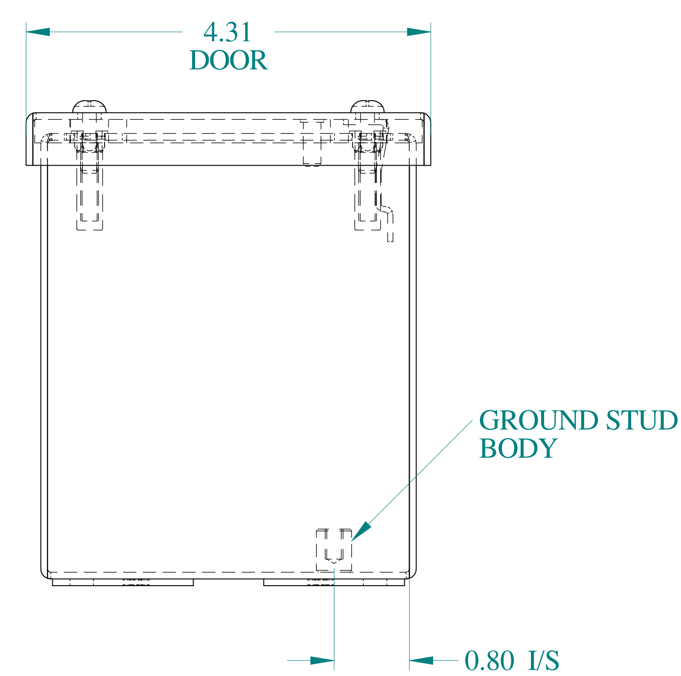
BOTTOM VIEW
