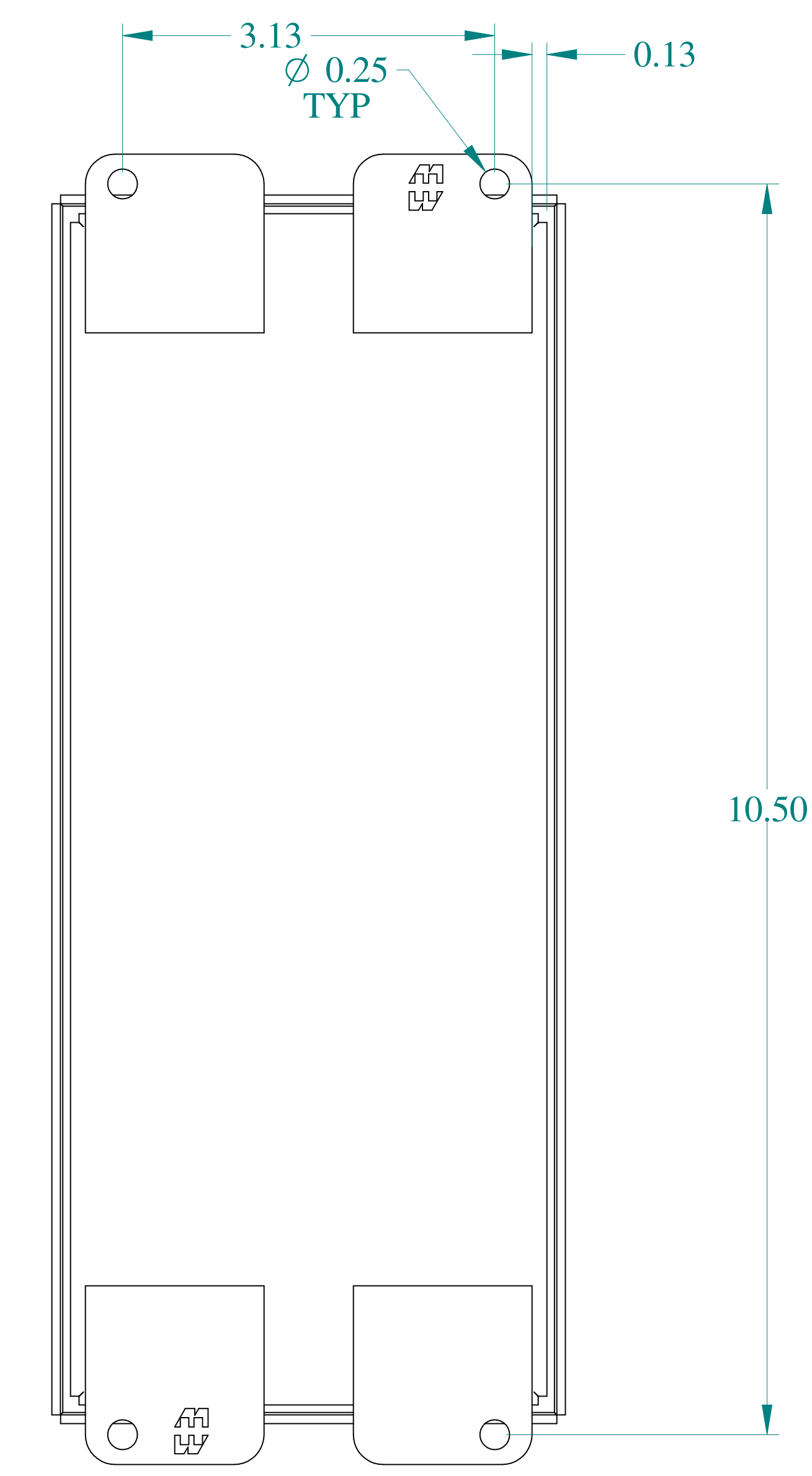
BACK VIEW
