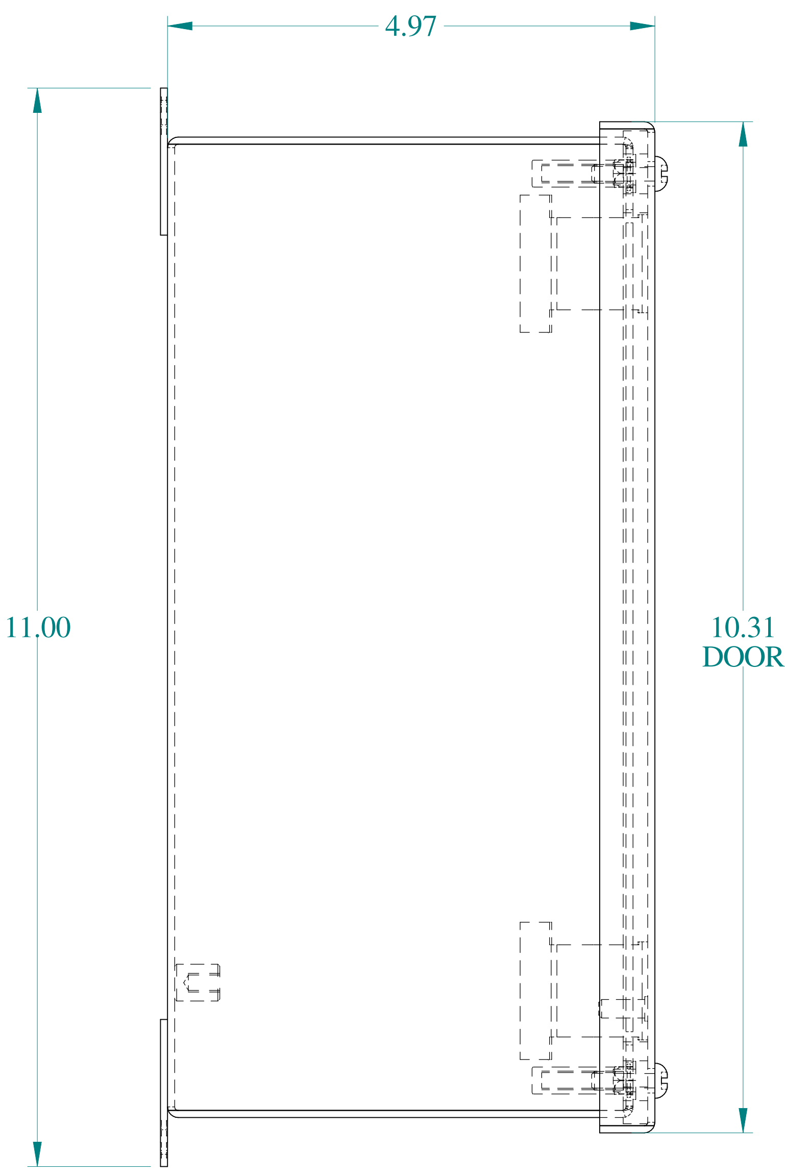
SIDE VIEW
