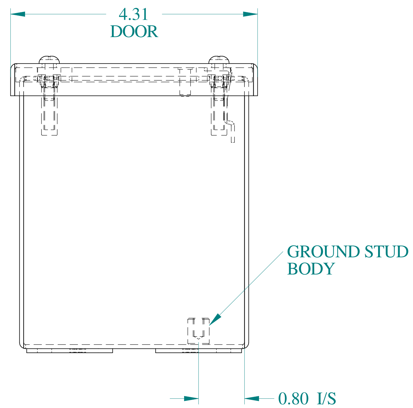
BOTTOM VIEW
