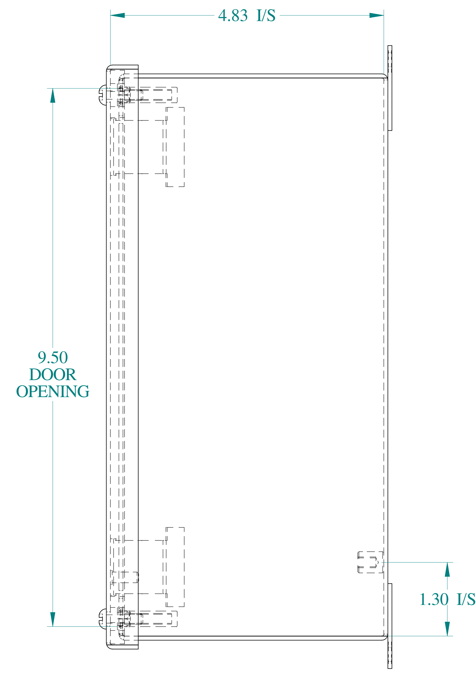
SIDE VIEW
