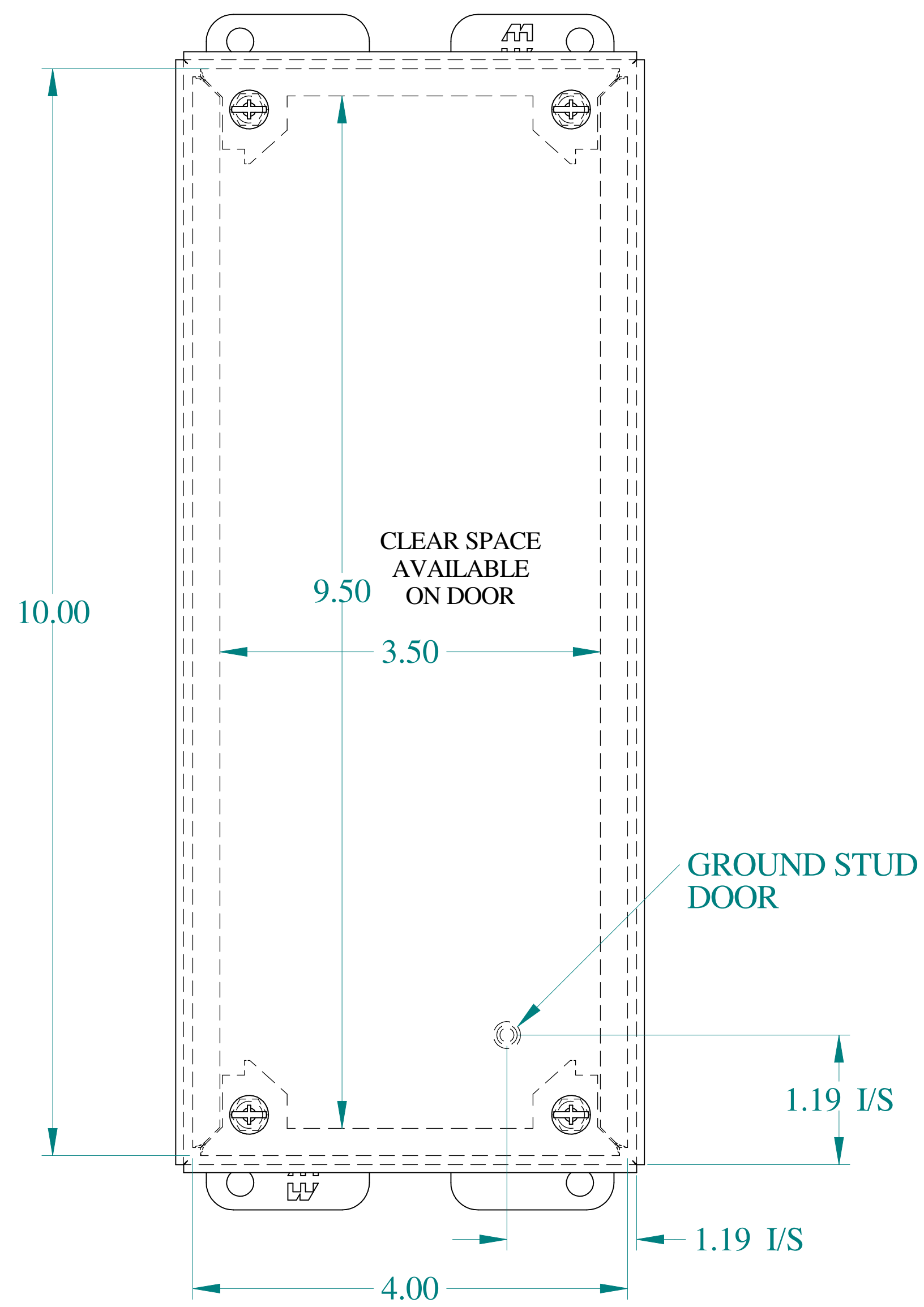
FRONT VIEW
