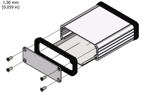
EXPLODED ISOMETRIC VIEW
