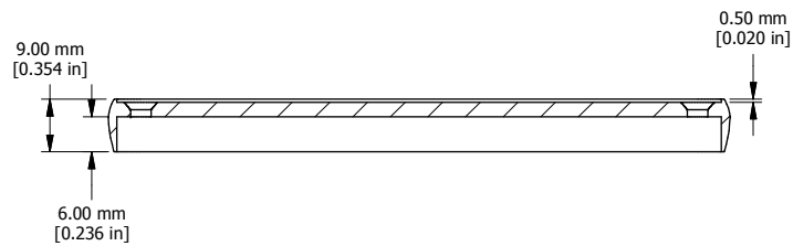
CLOSED BEZEL
