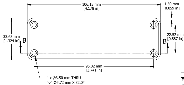
CLOSED BEZEL
