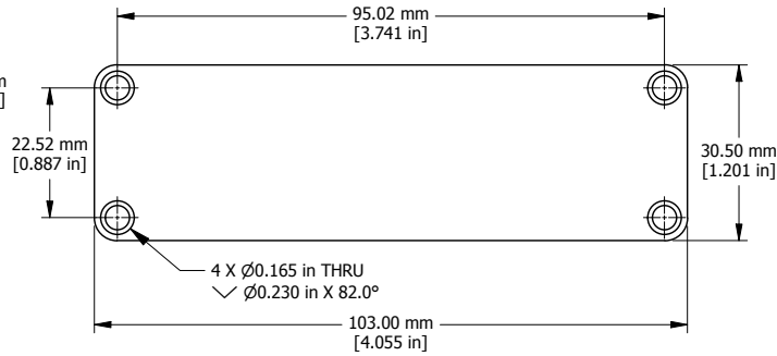
END PLATE
