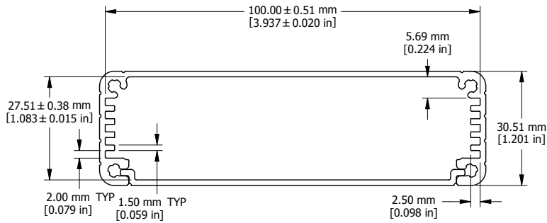
EXTRUSION
