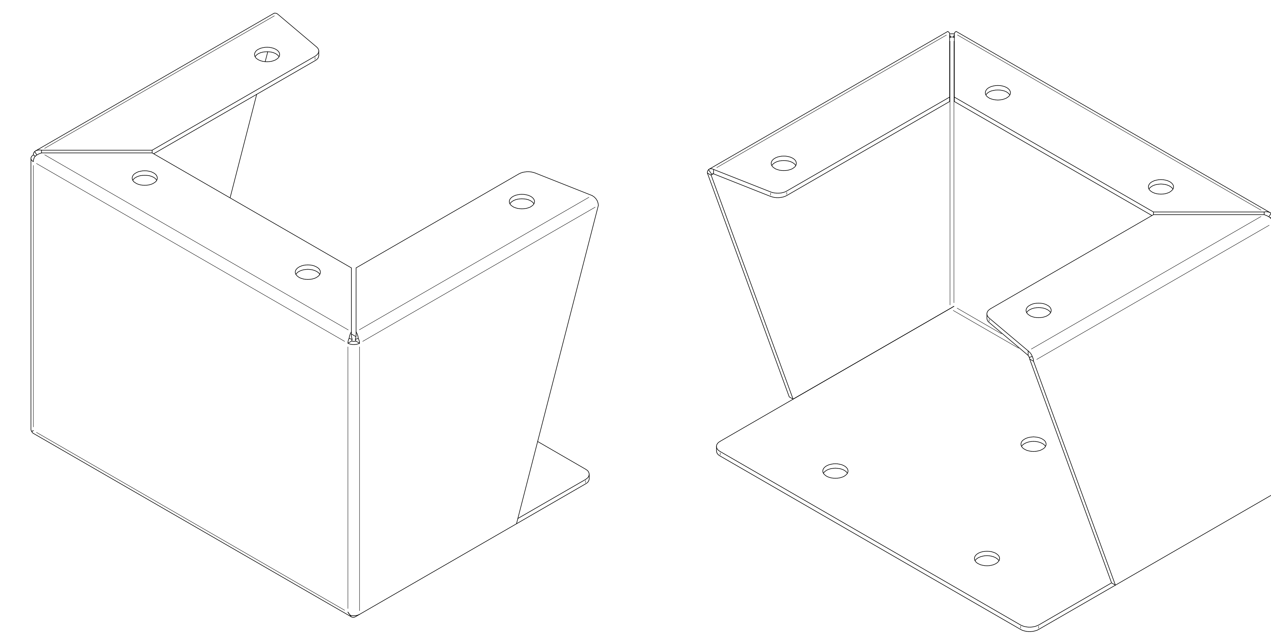
ISOMETRIC VIEWS
