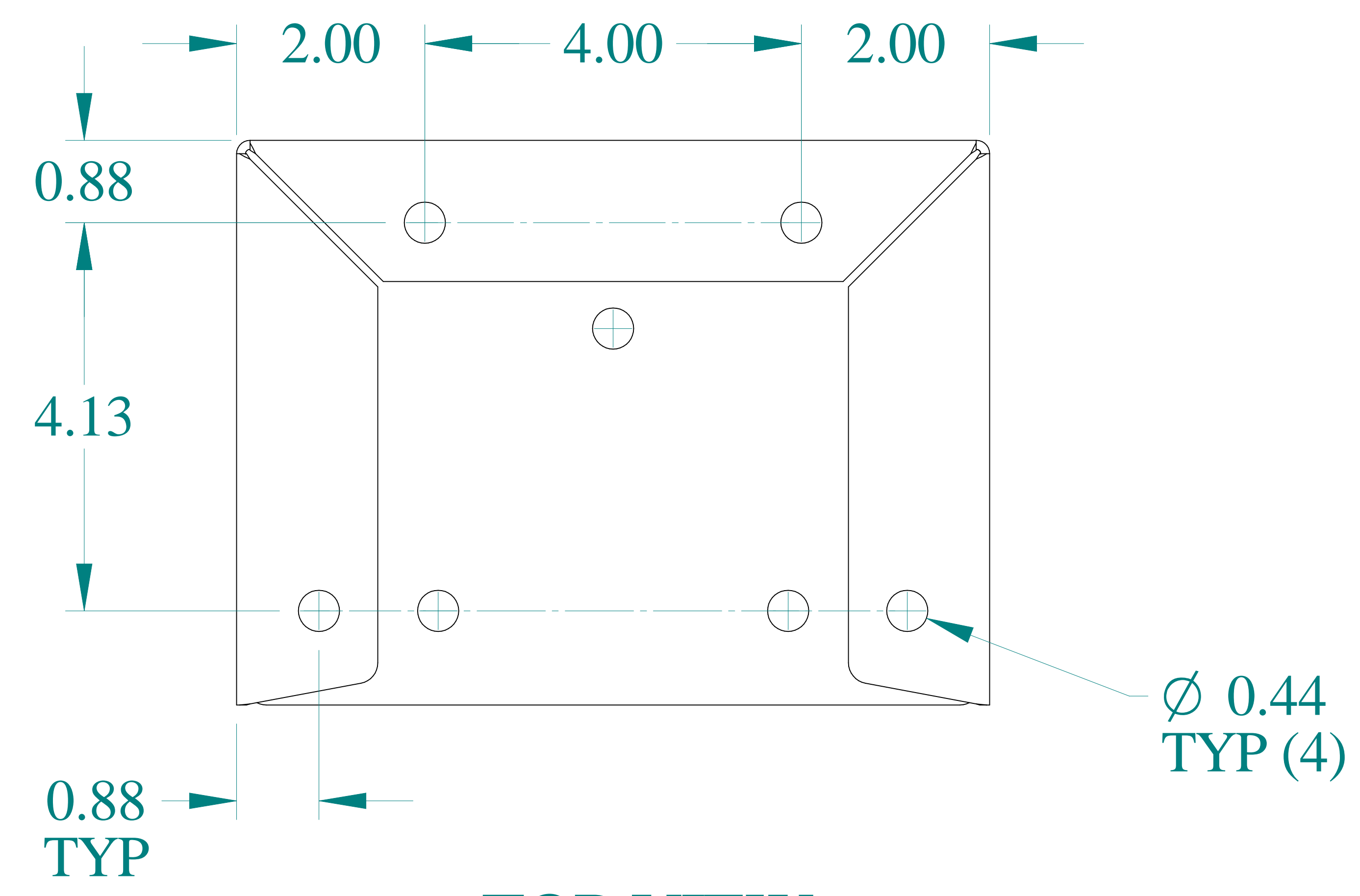
TOP VIEW
