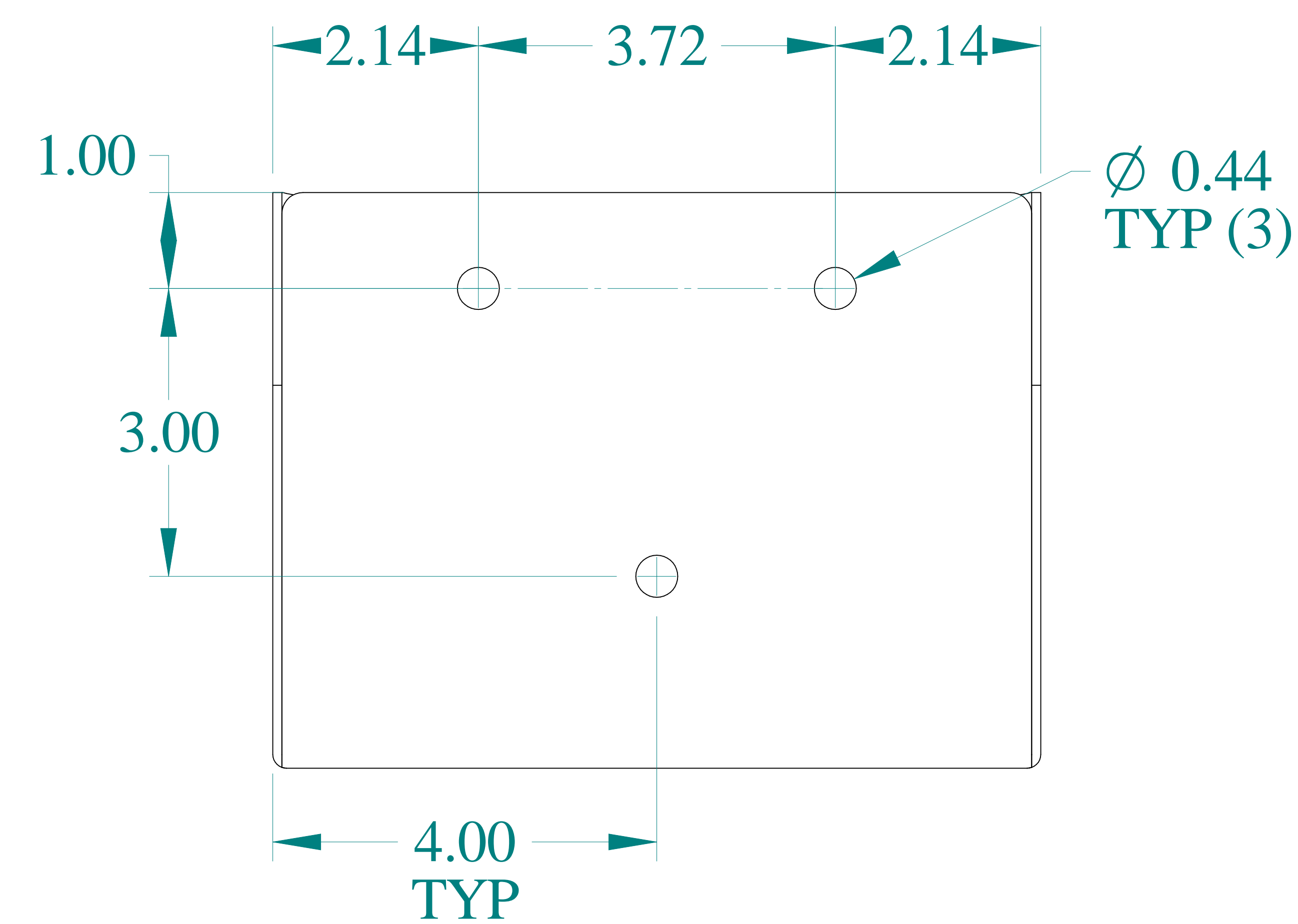
BOTTOM VIEW
