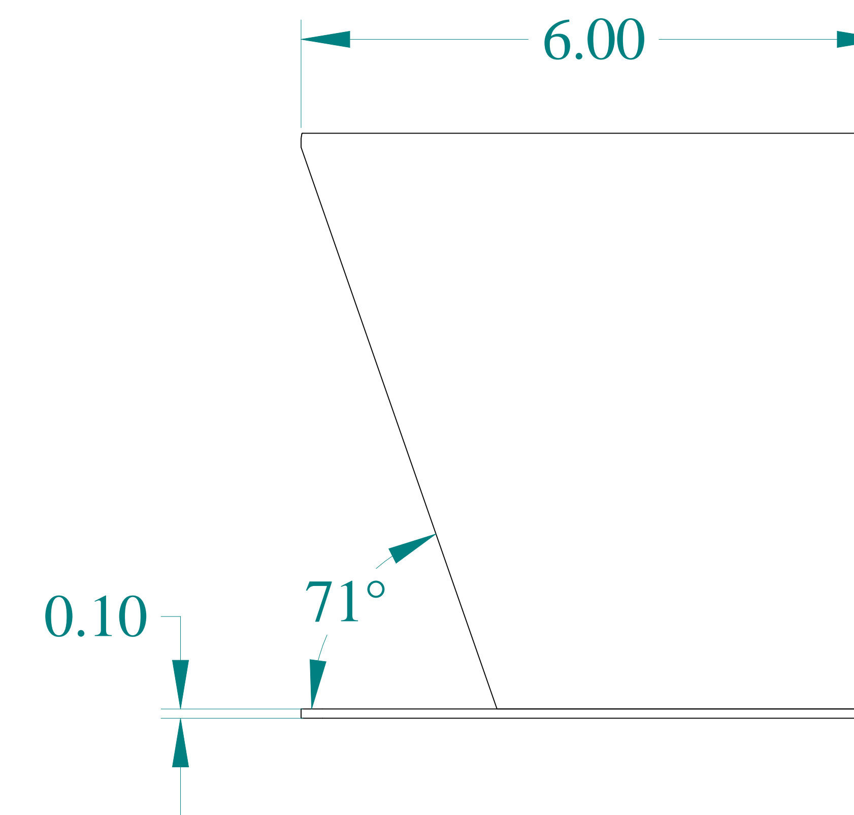
SIDE VIEW
