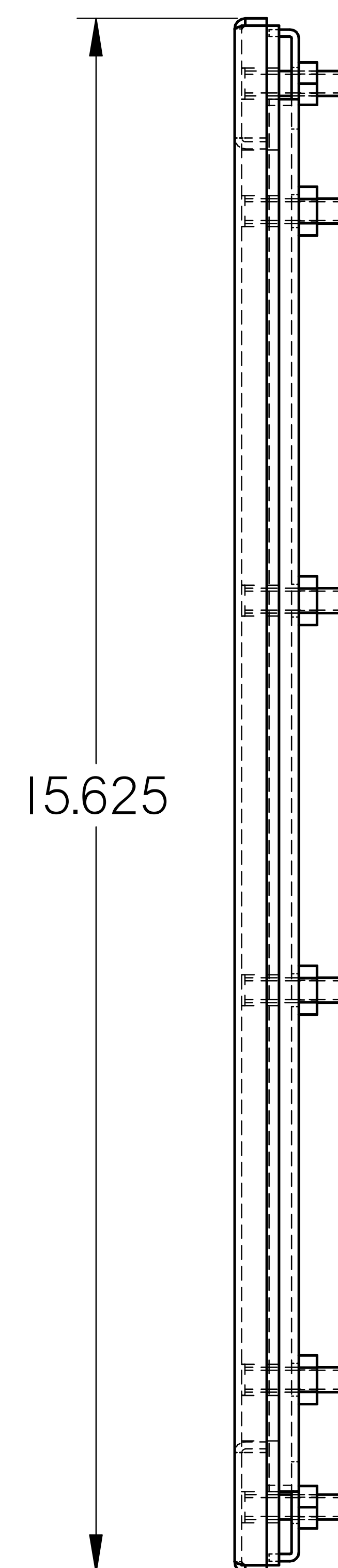
SIDE VIEW
