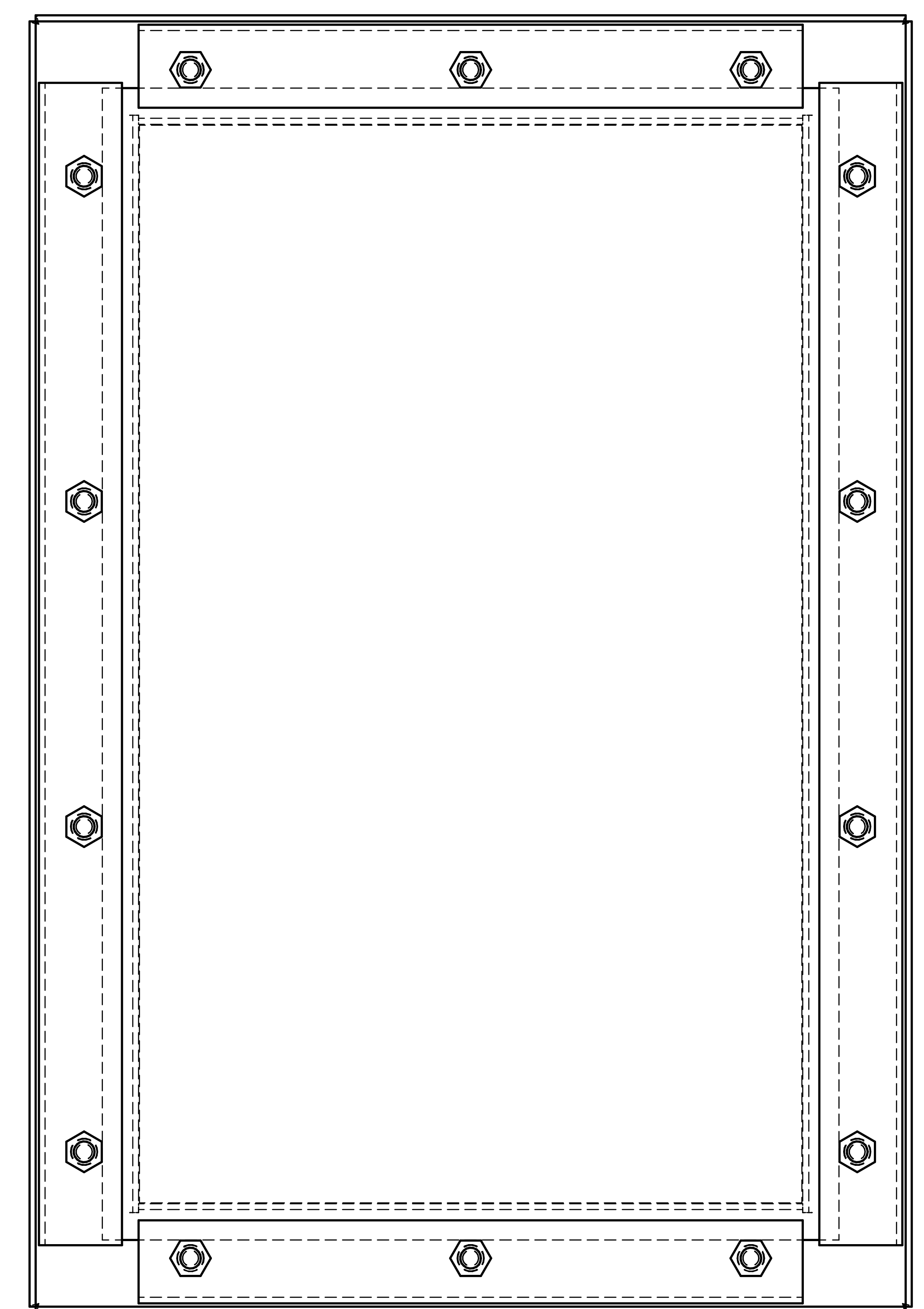
BACK VIEW
