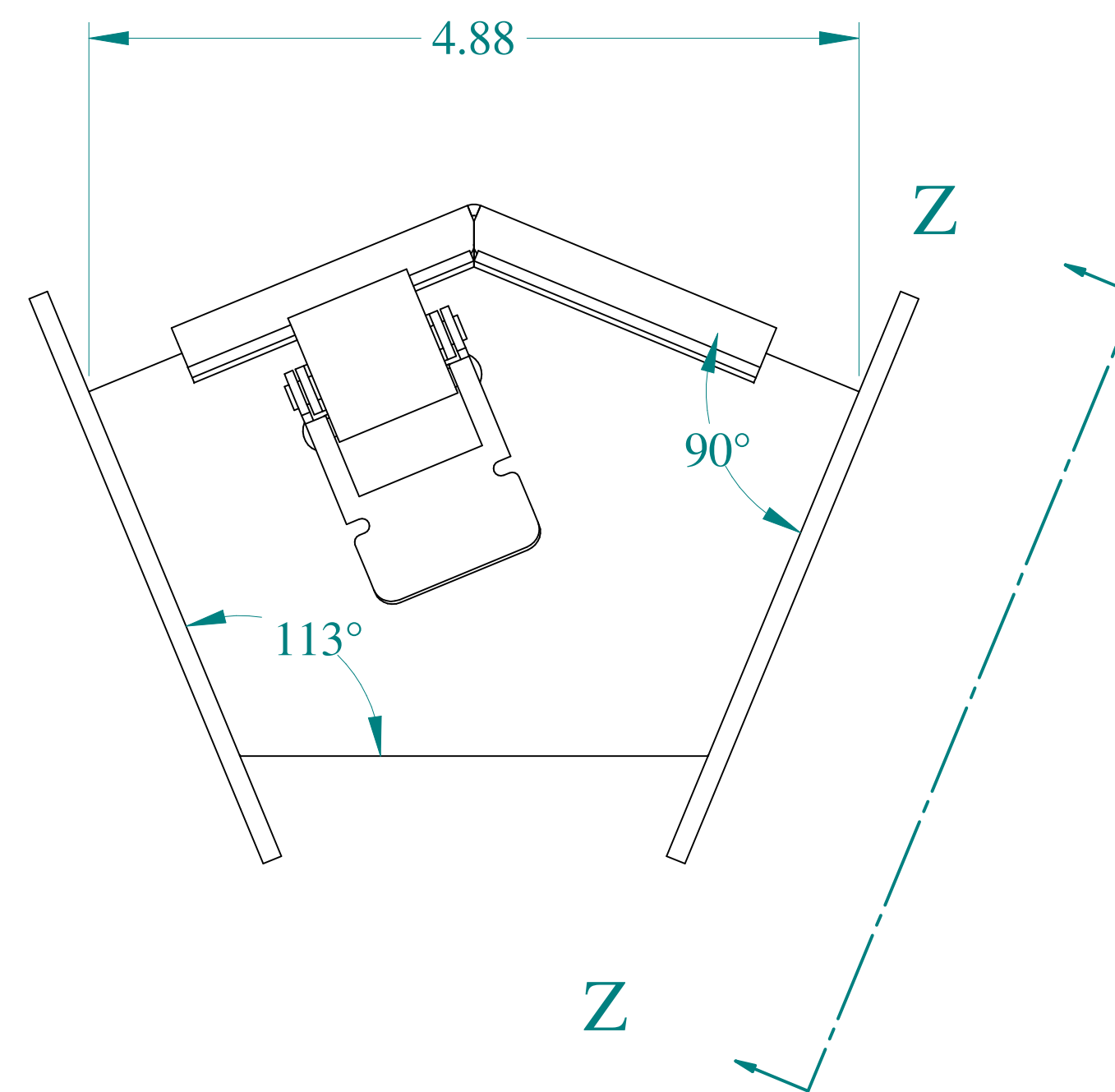
FRONT VIEW
