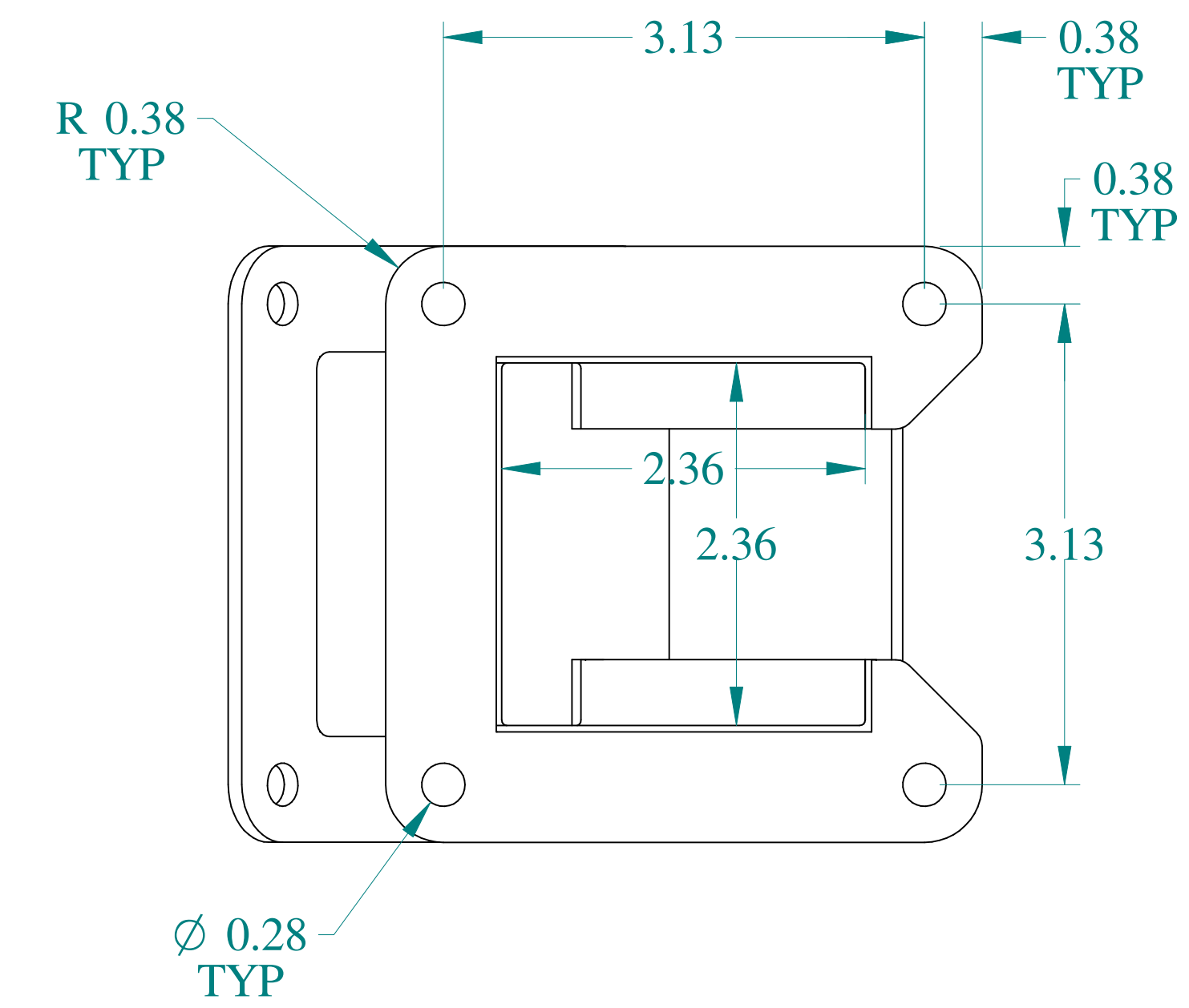
VIEW Z-Z
