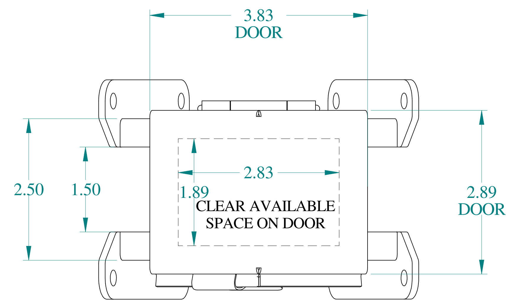
TOP VIEW
