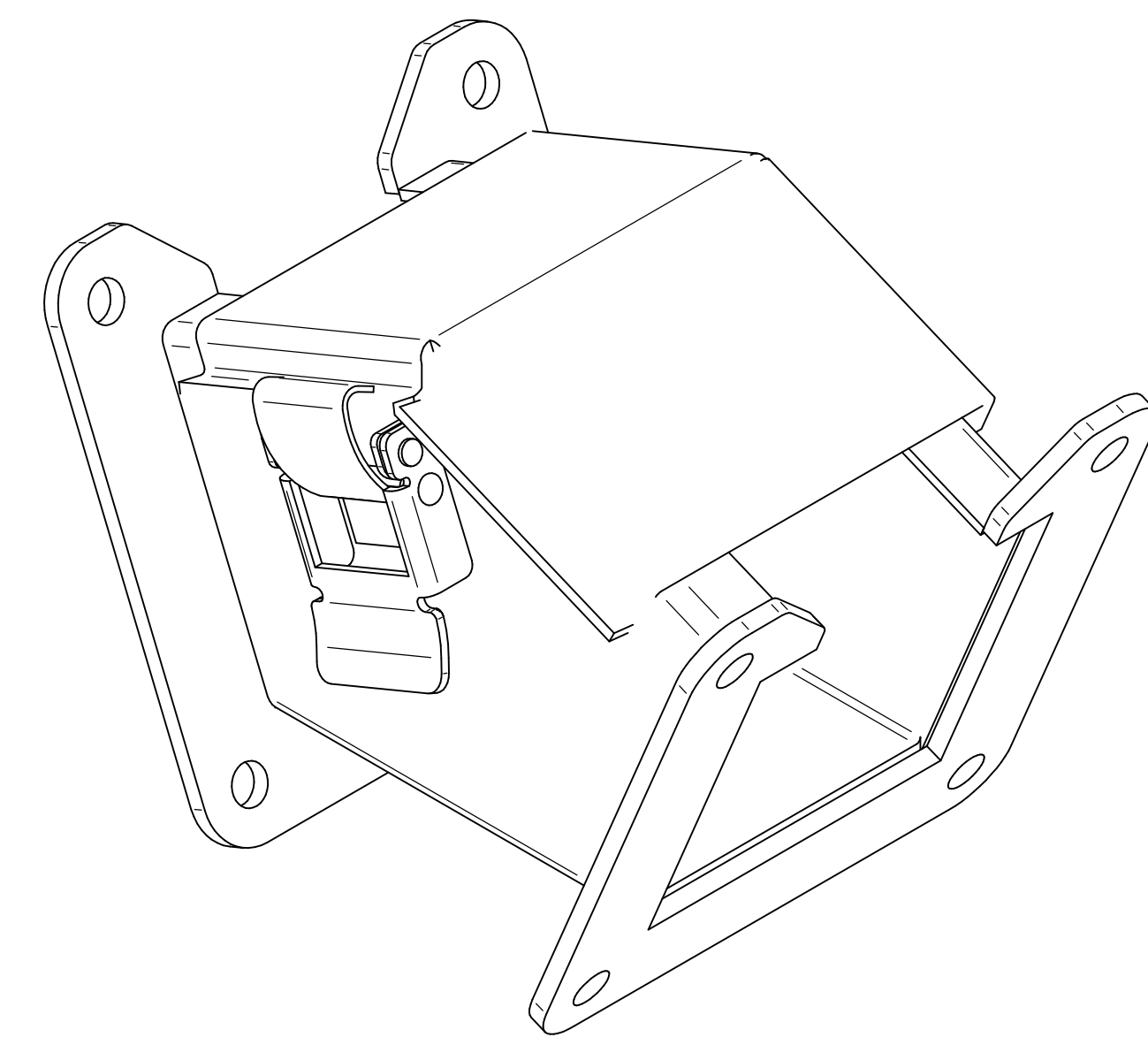
ISOMETRIC VIEWS
