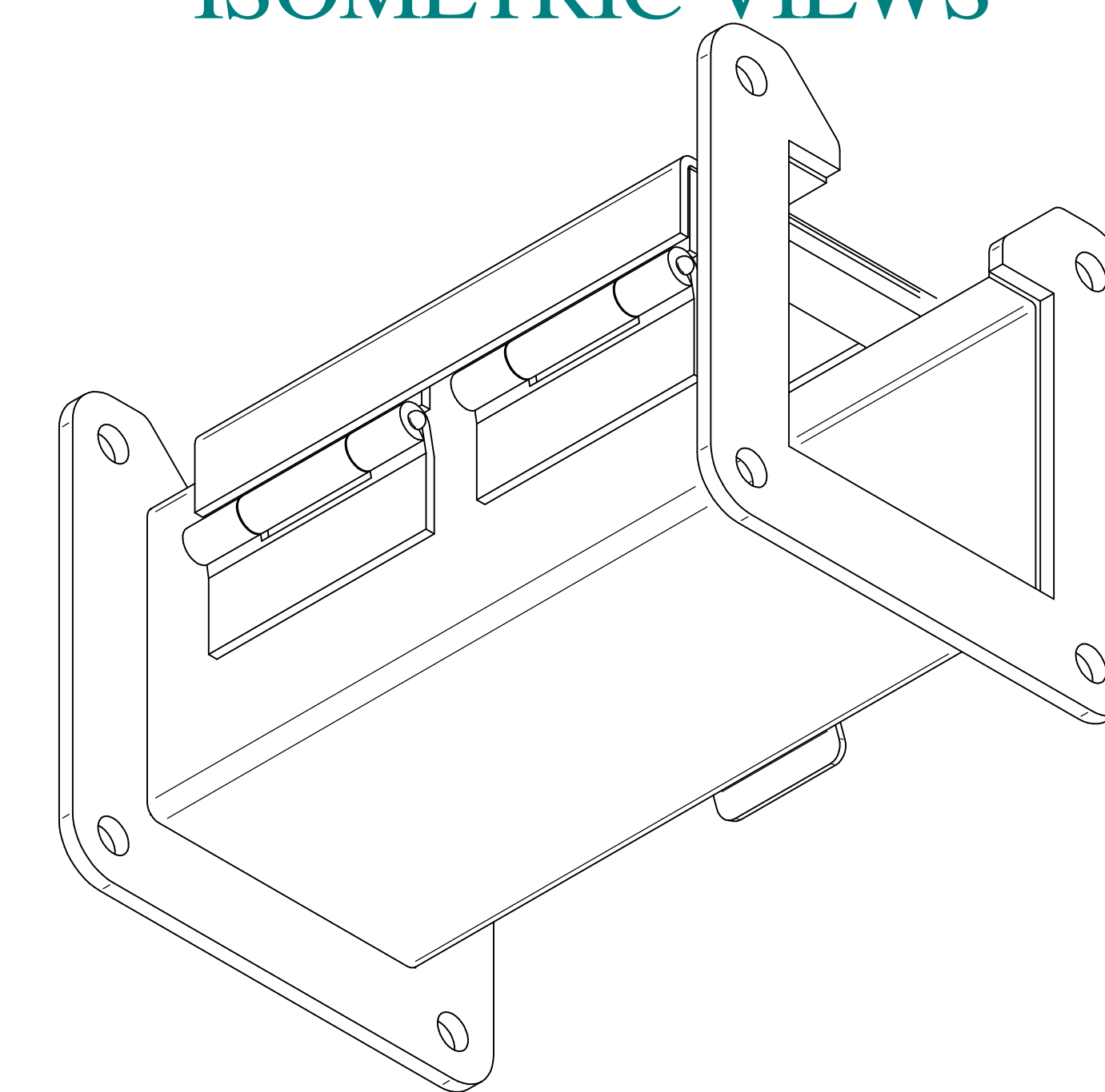
ISOMETRIC VIEWS
