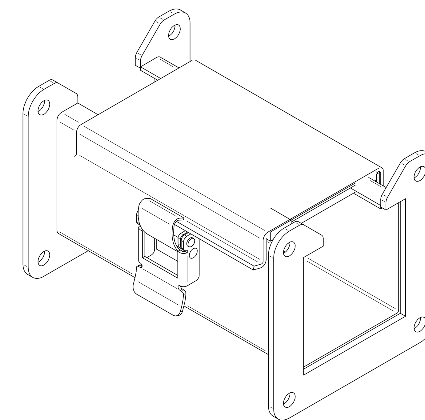
ISOMETRIC VIEWS
