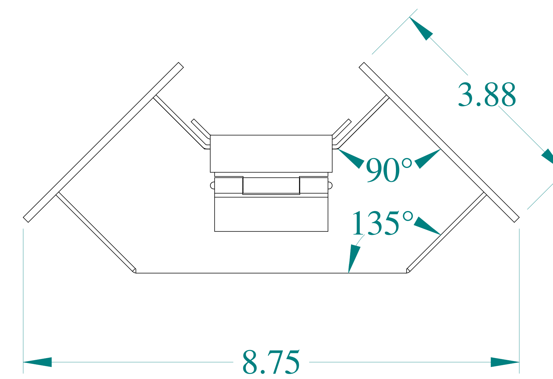
BOTTOM VIEW
