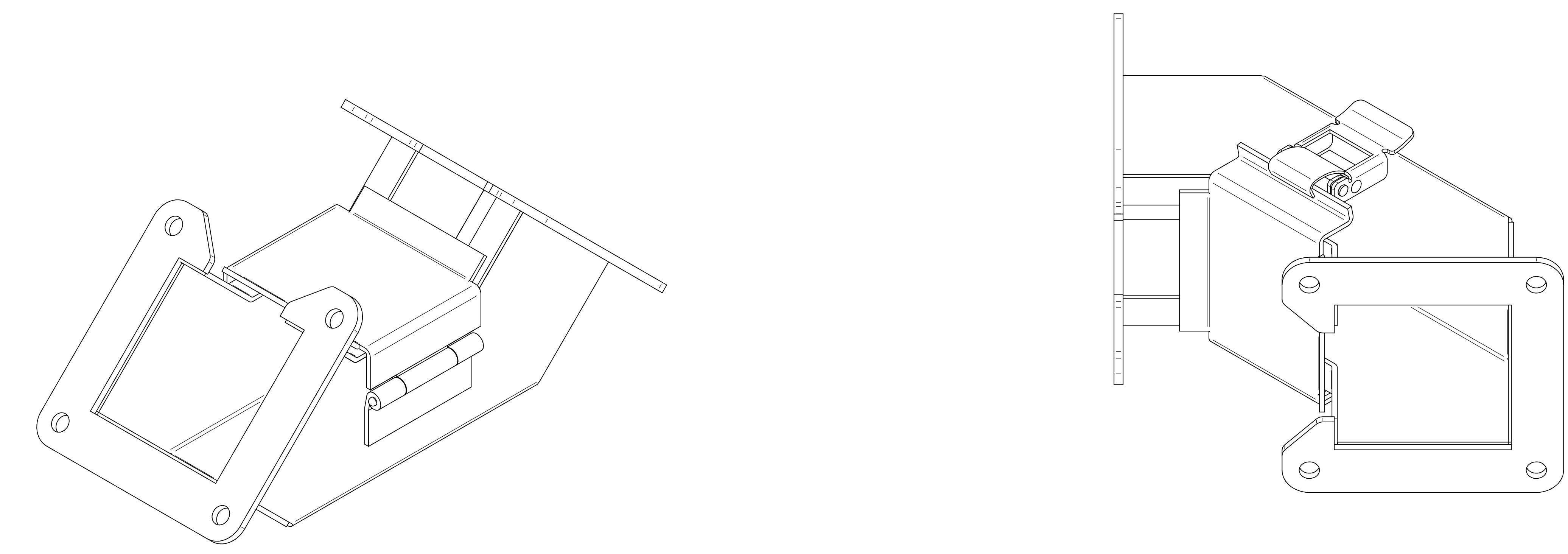
ISOMETRIC VIEWS
