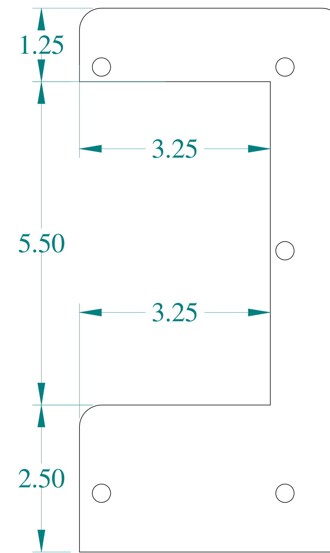
BACK VIEW
