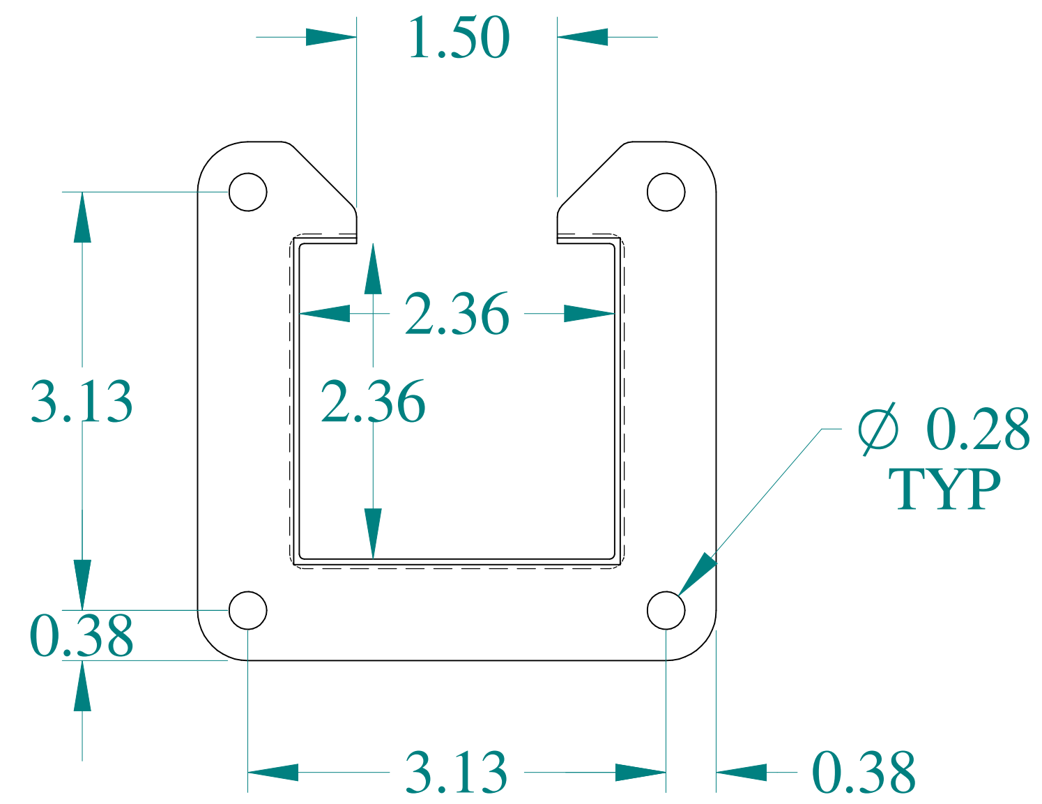
FRONT VIEW
