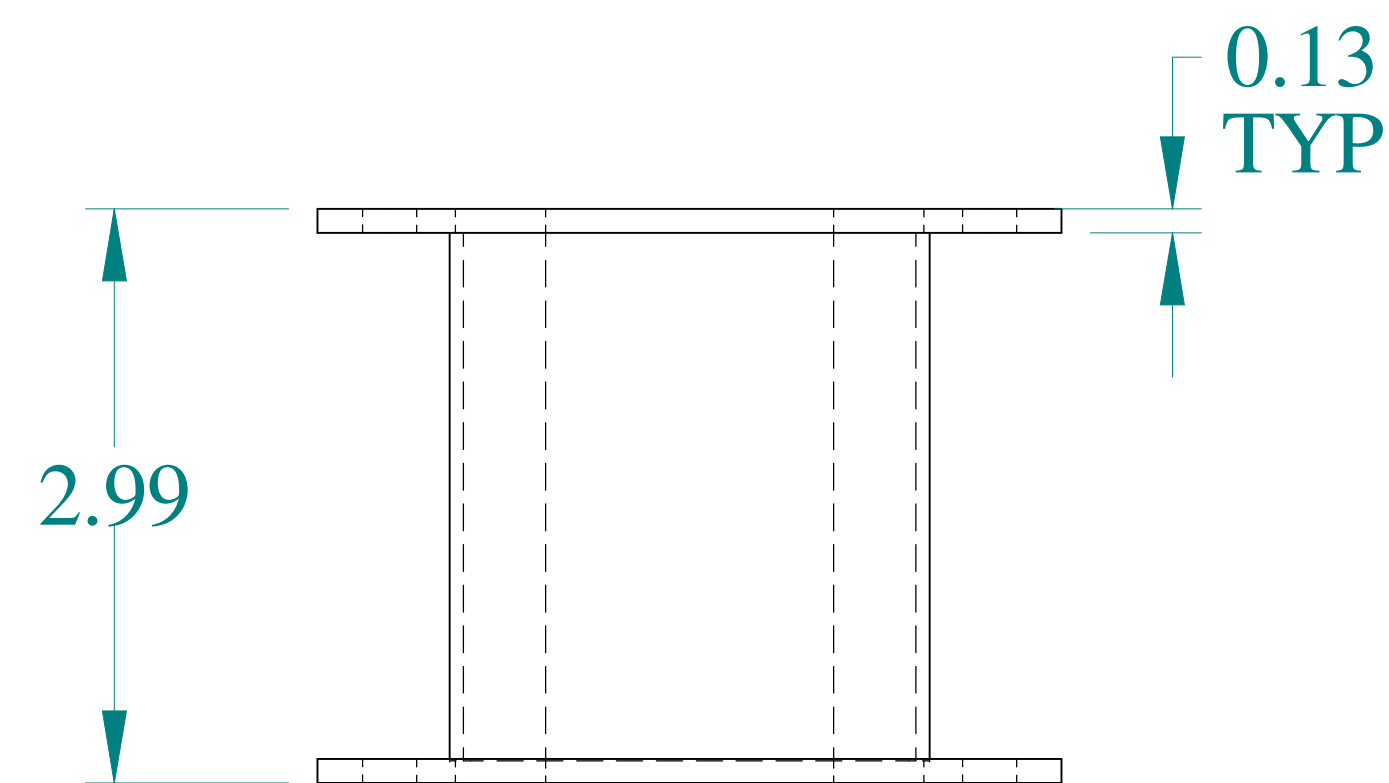
BOTTOM VIEW
