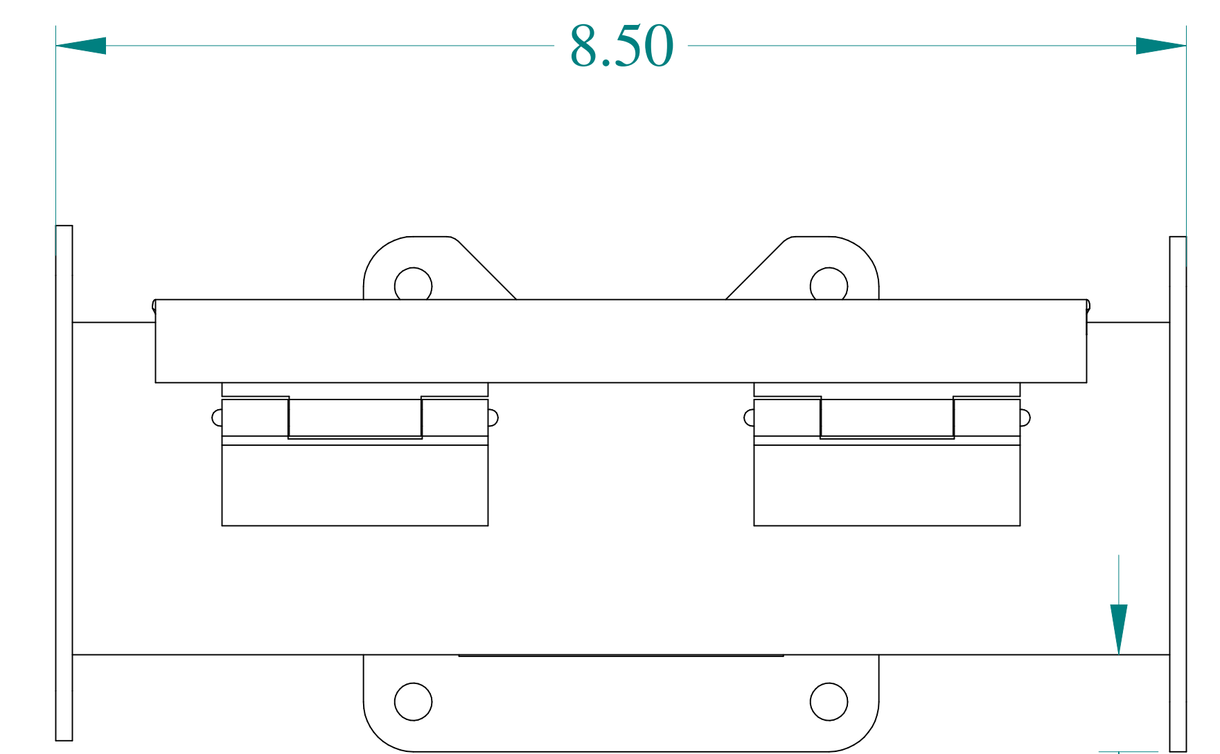
BACK VIEW
