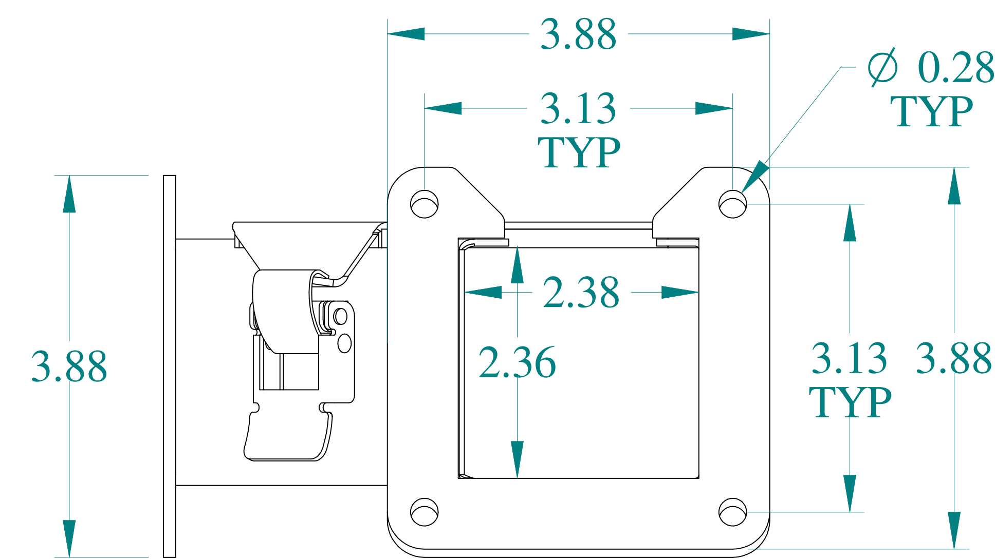
SIDE VIEW
