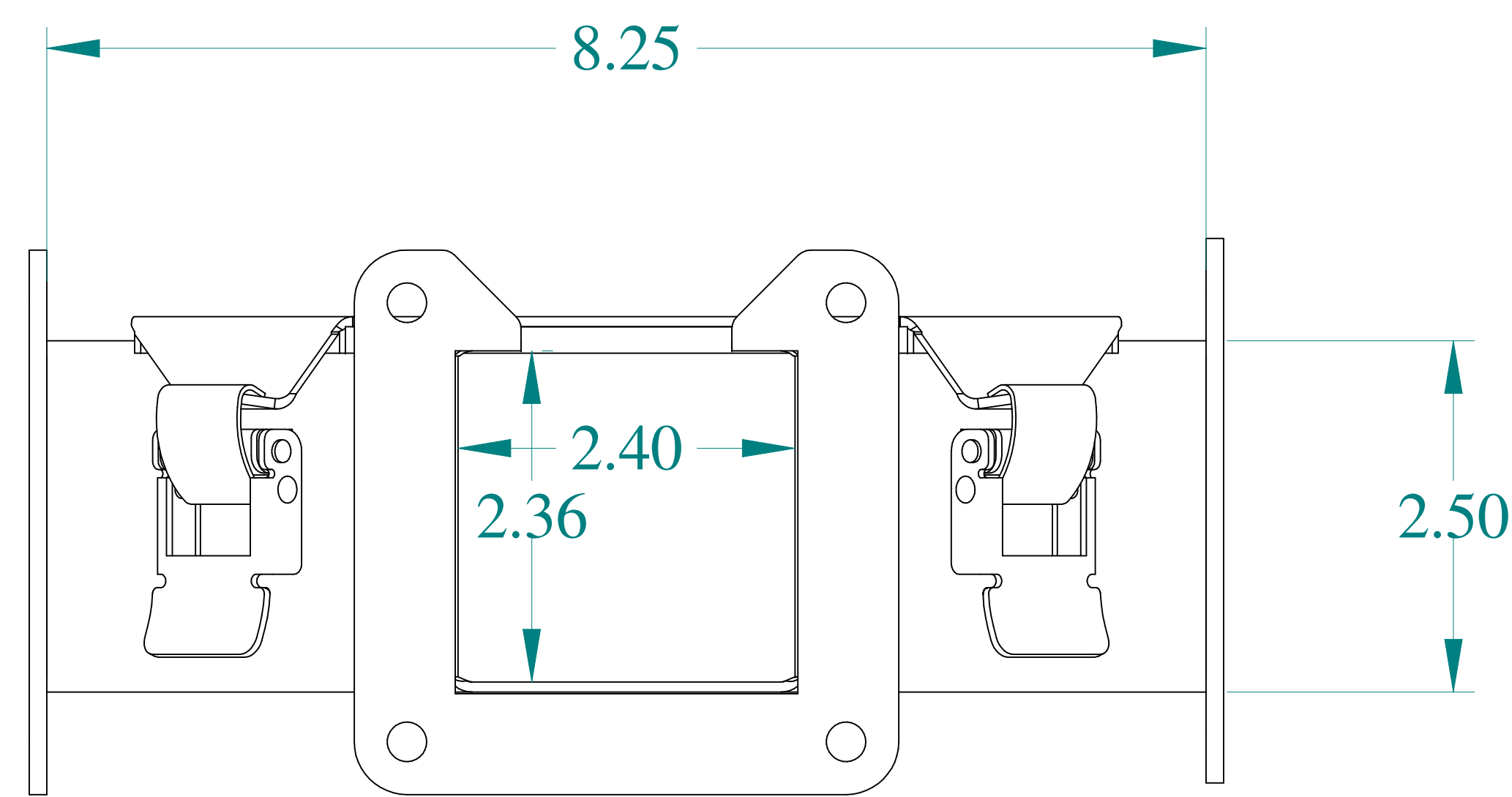
FRONT VIEW
