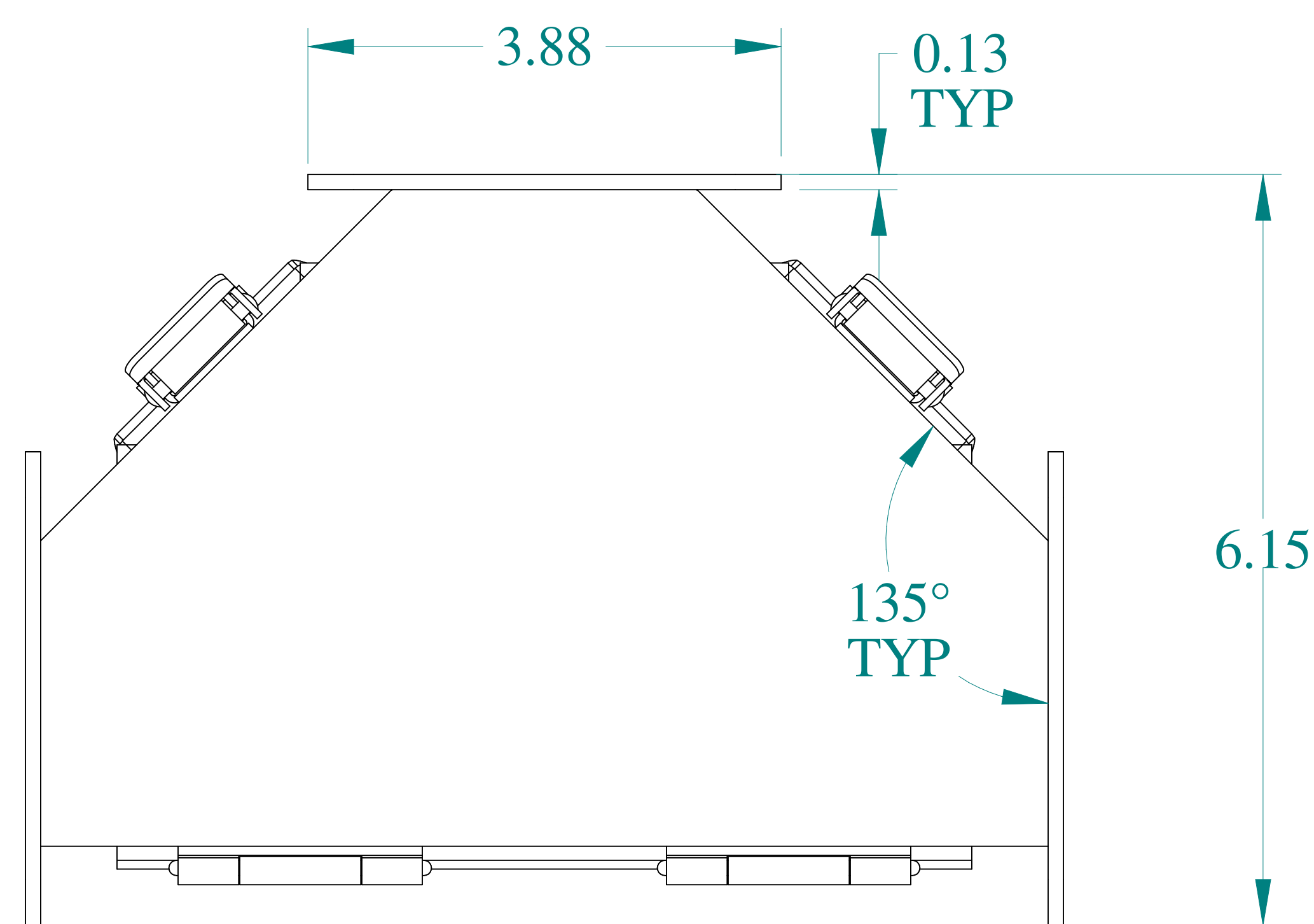
BOTTOM VIEW
