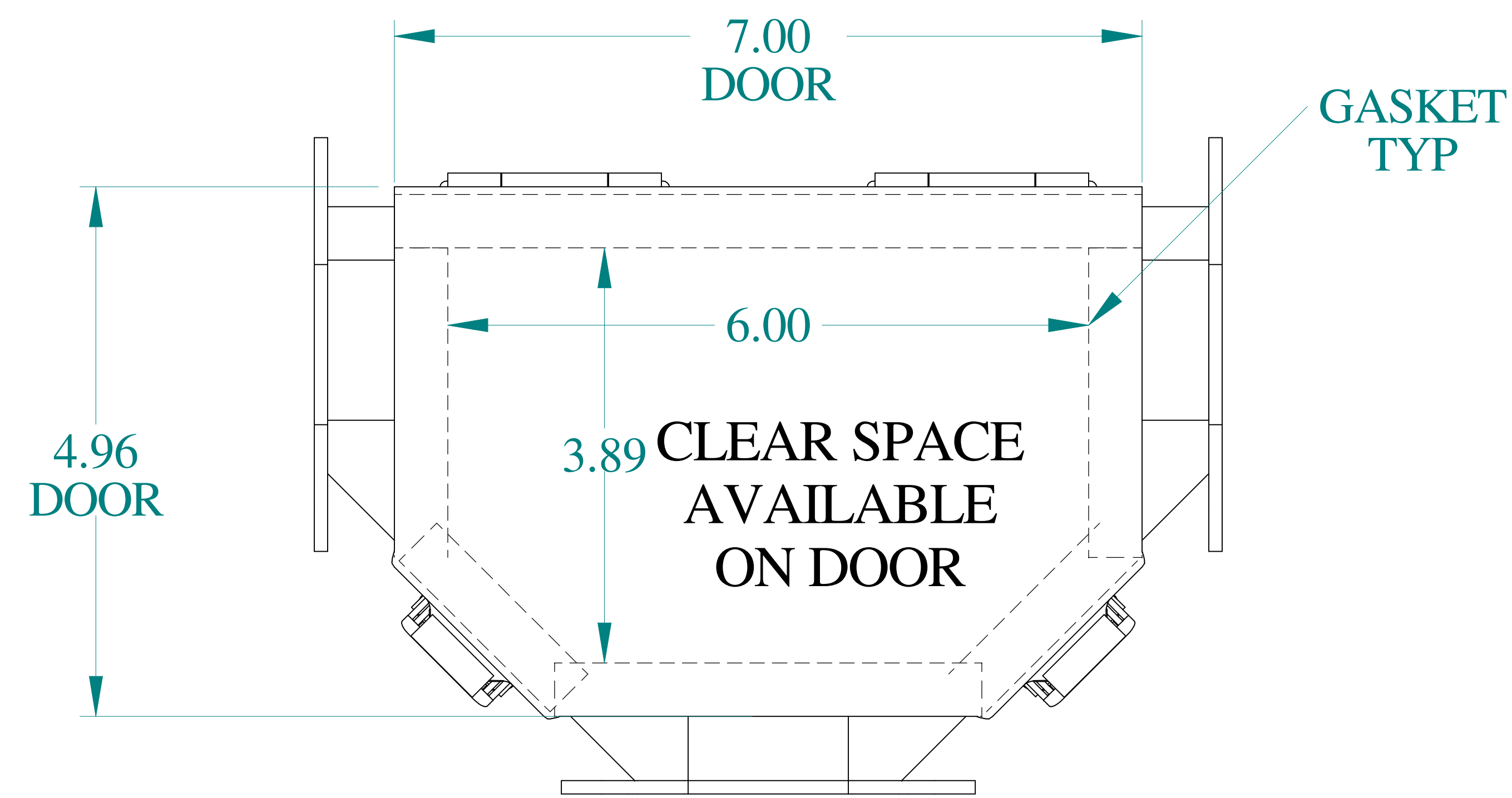
TOP VIEW
