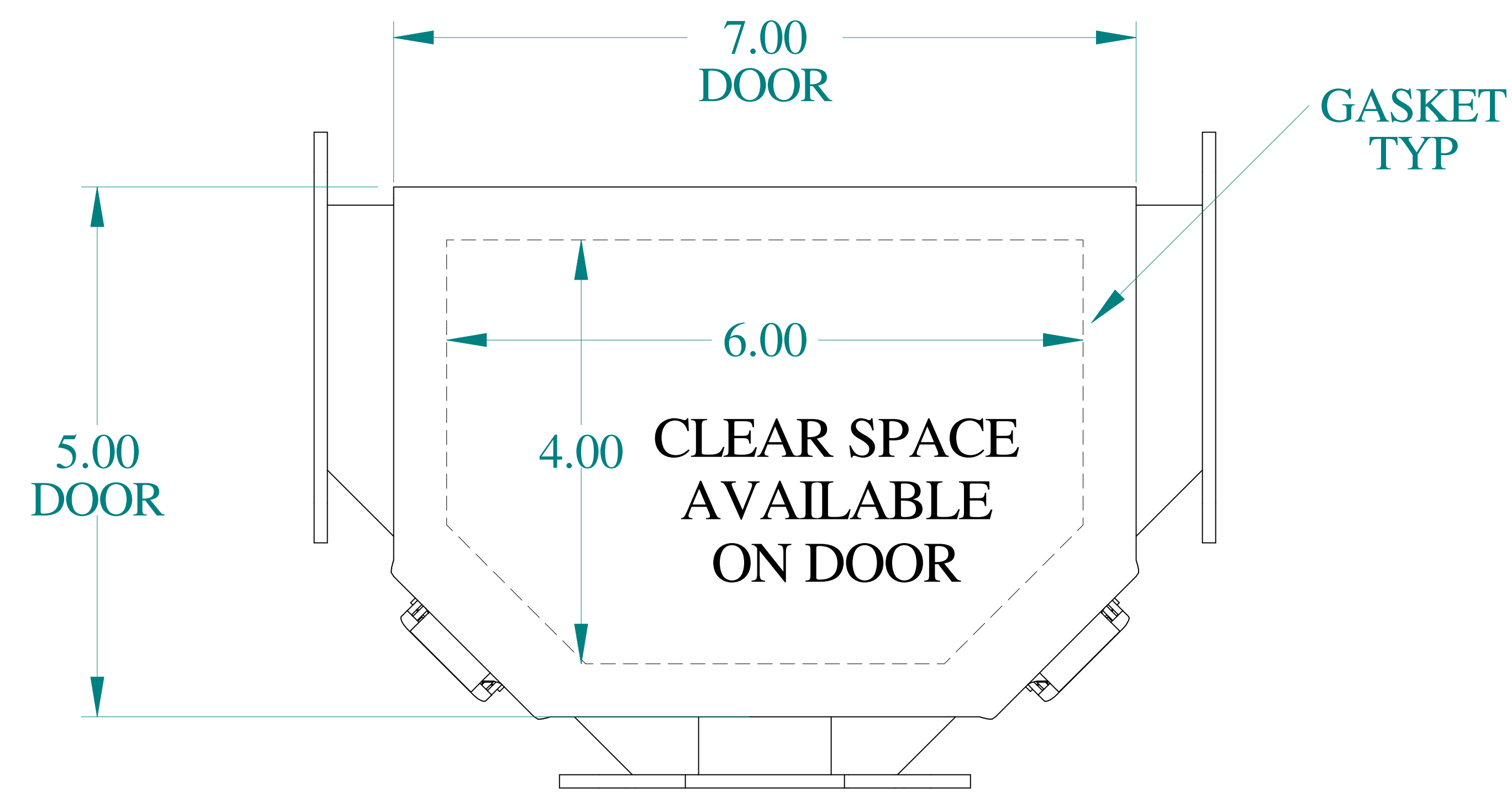
TOP VIEW
