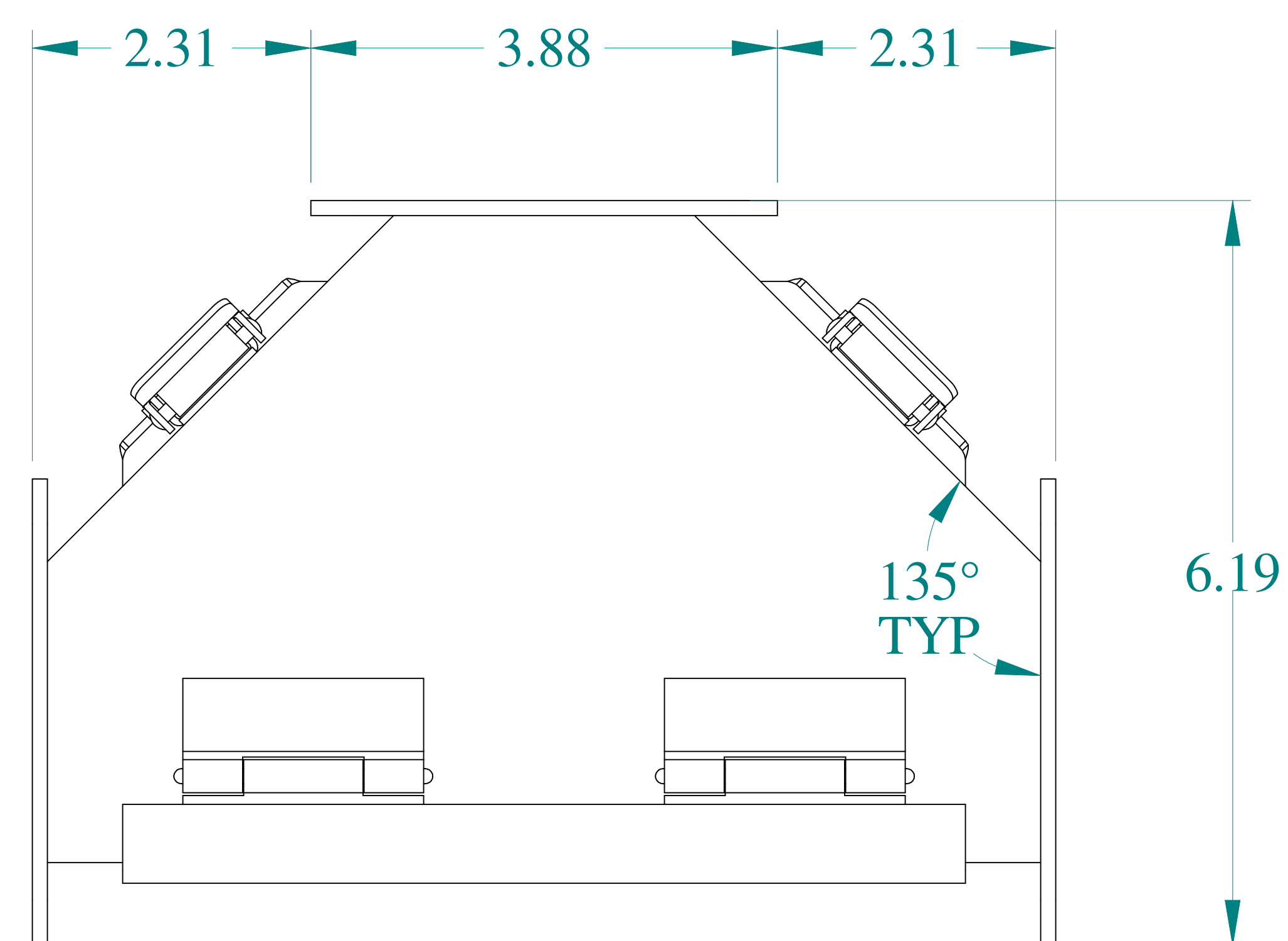
BOTTOM VIEW
