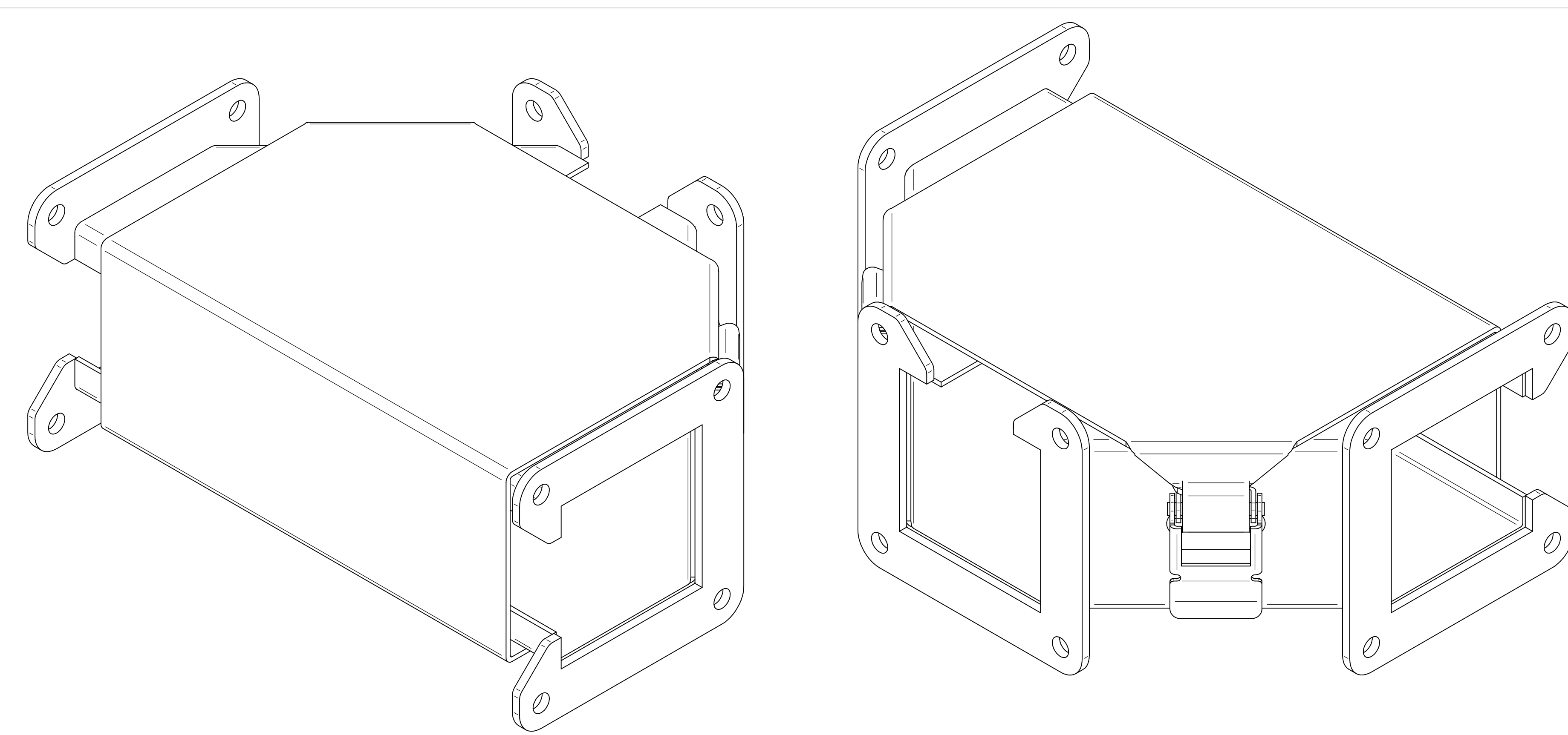
ISOMETRIC VIEWS
