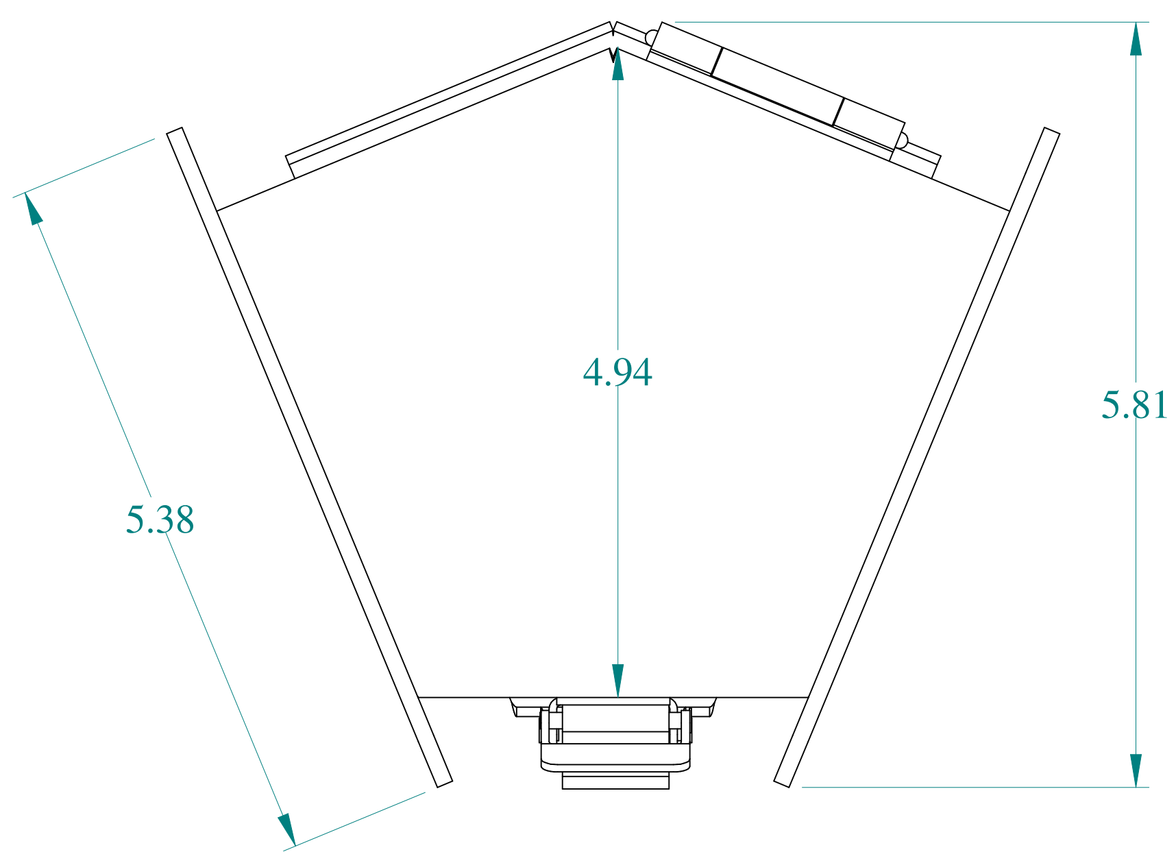
BACK VIEW
