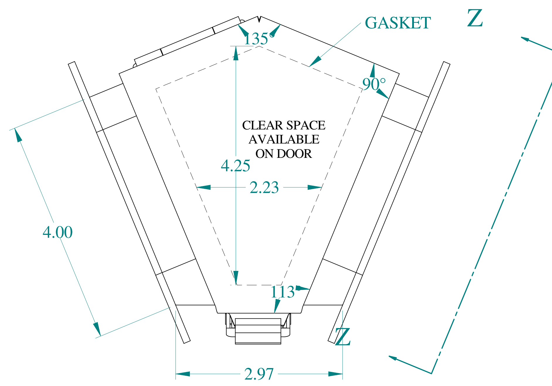
FRONT VIEW
