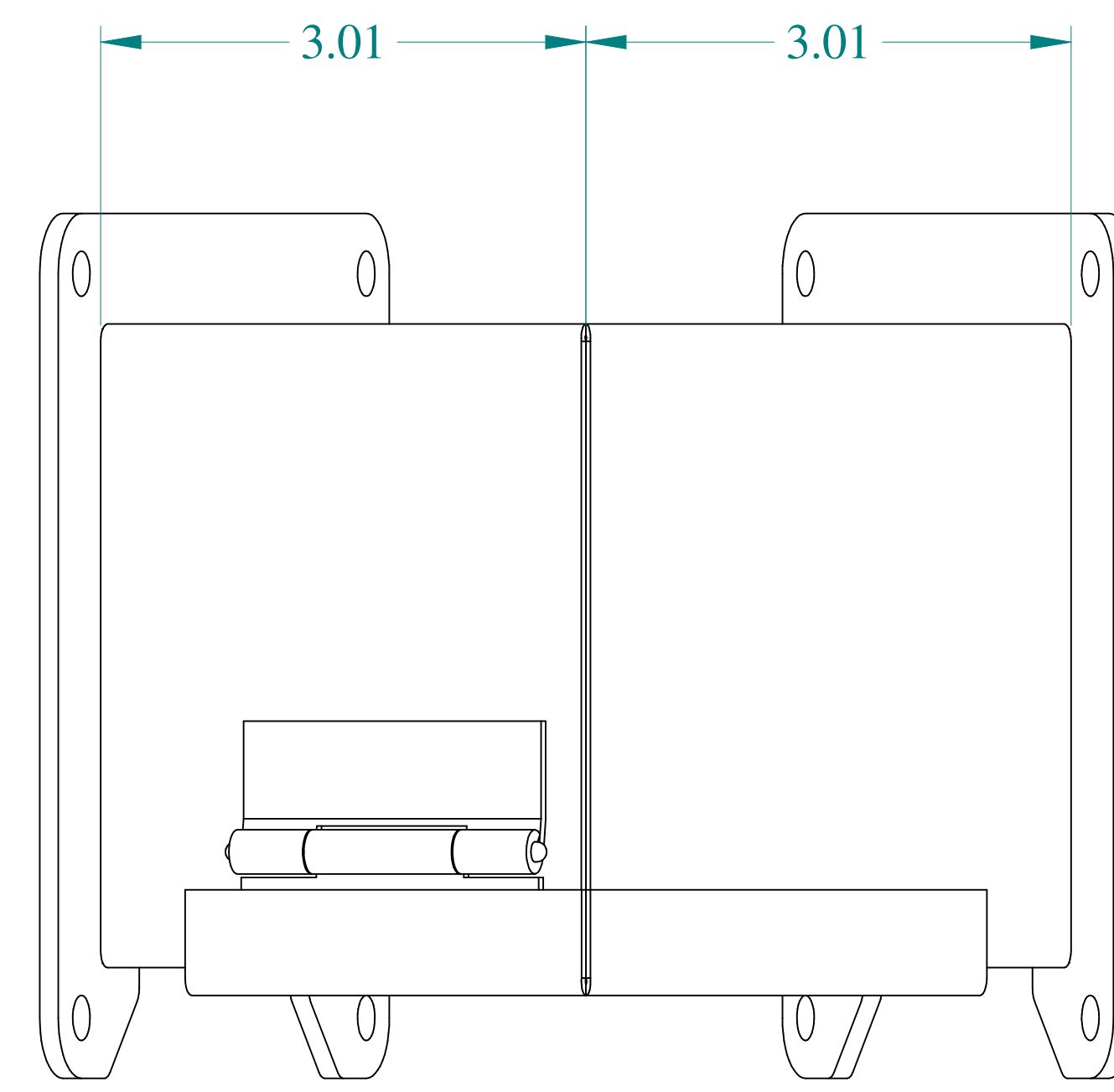
TOP VIEW
