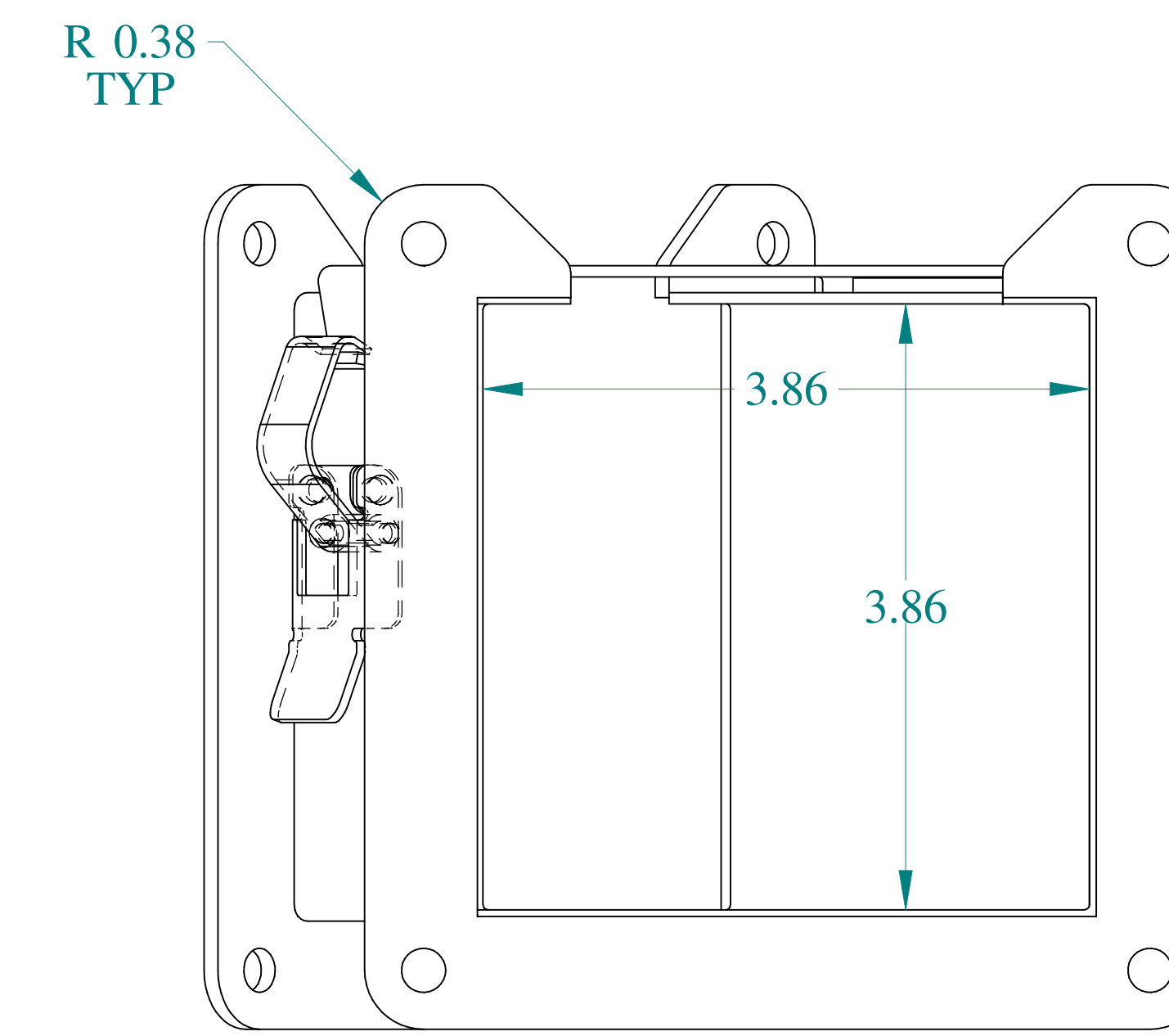
VIEW Z-Z
