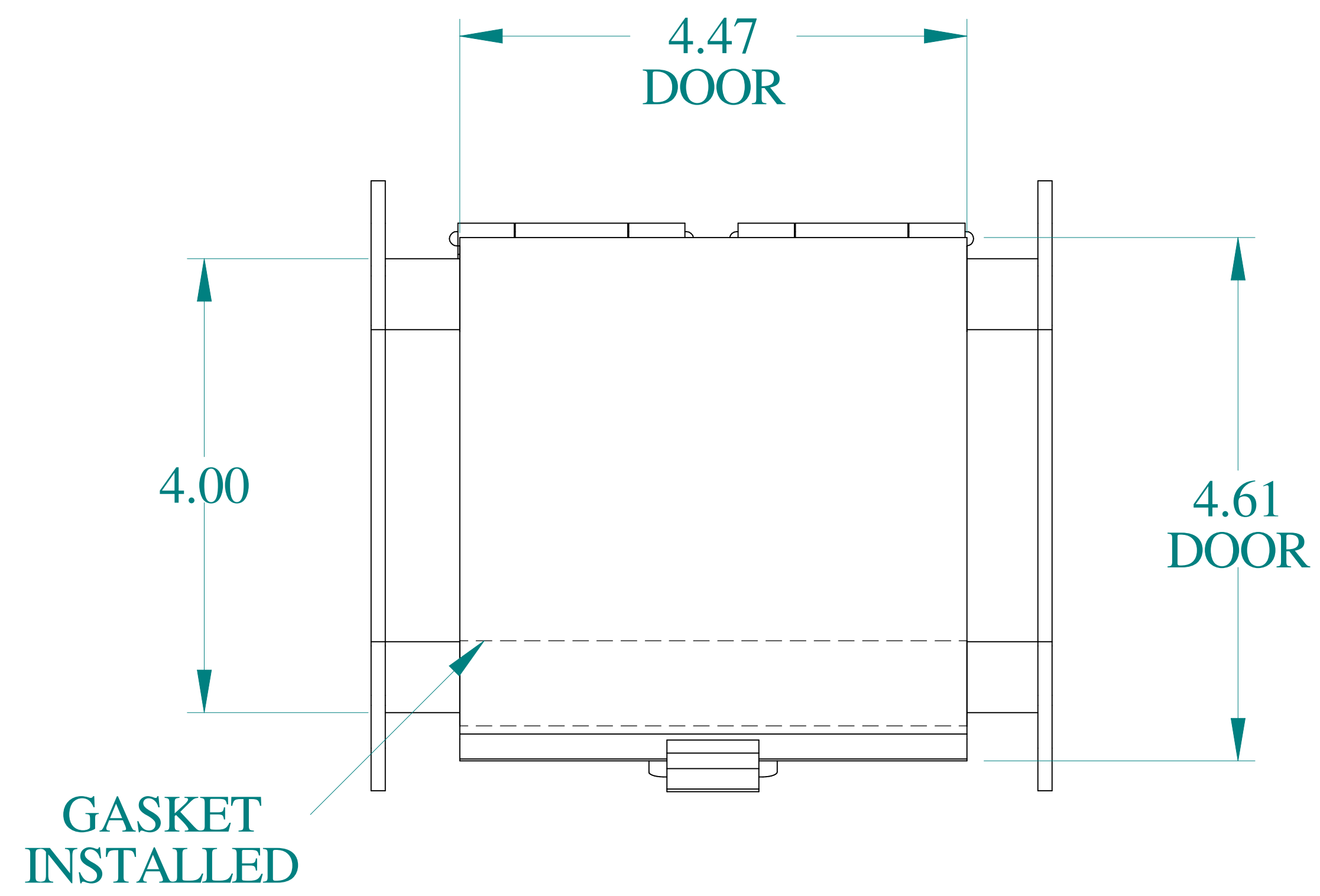
TOP VIEW
