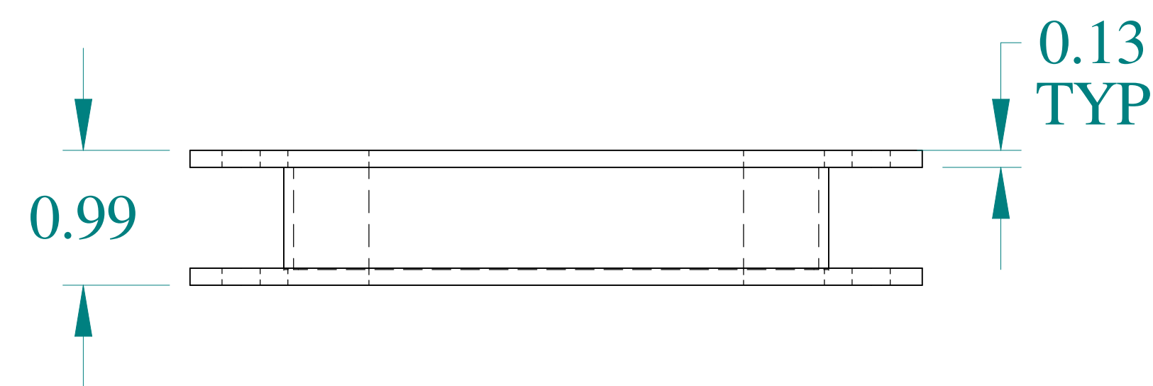
BOTTOM VIEW
