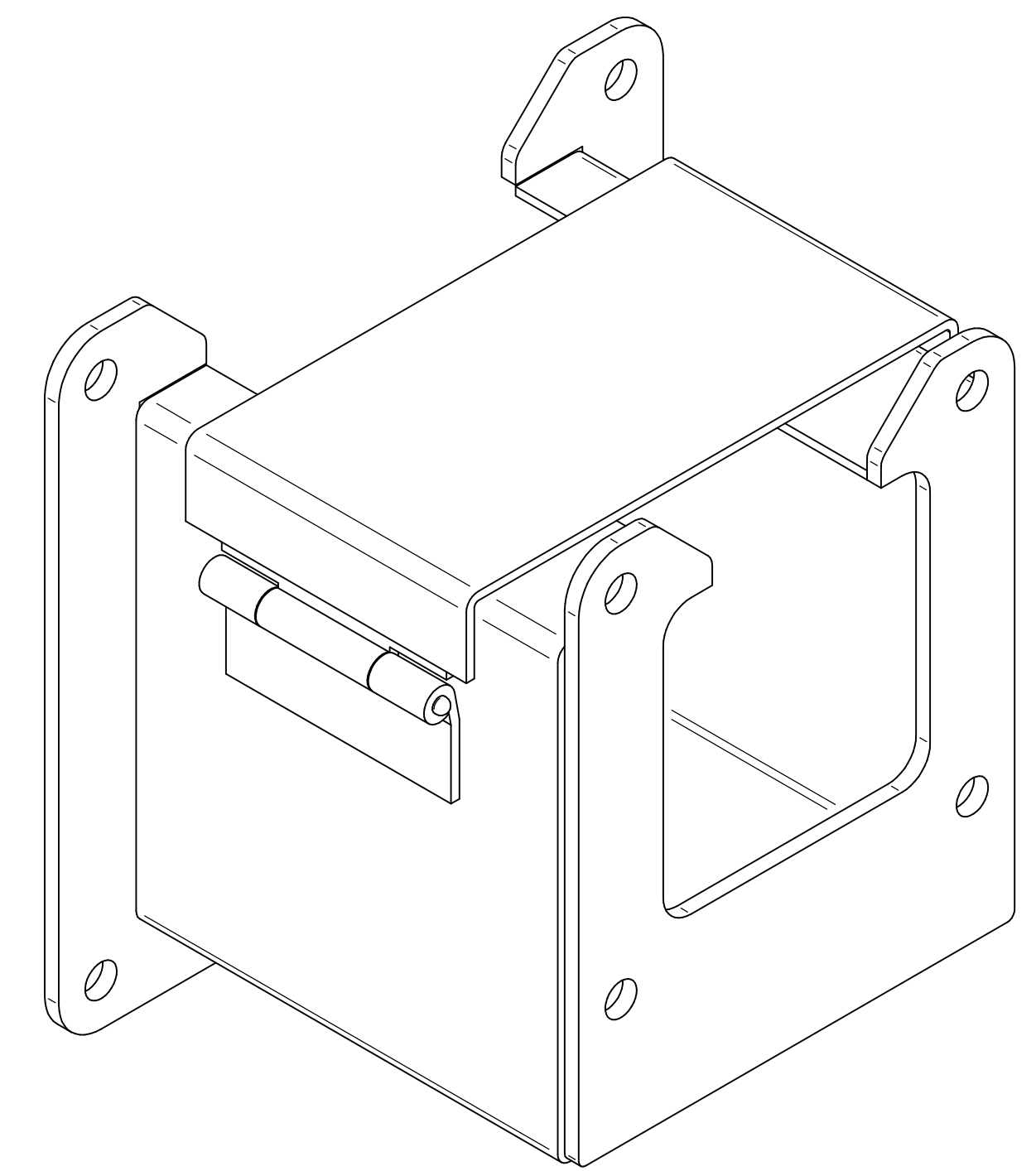
ISOMETRIC VIEWS
