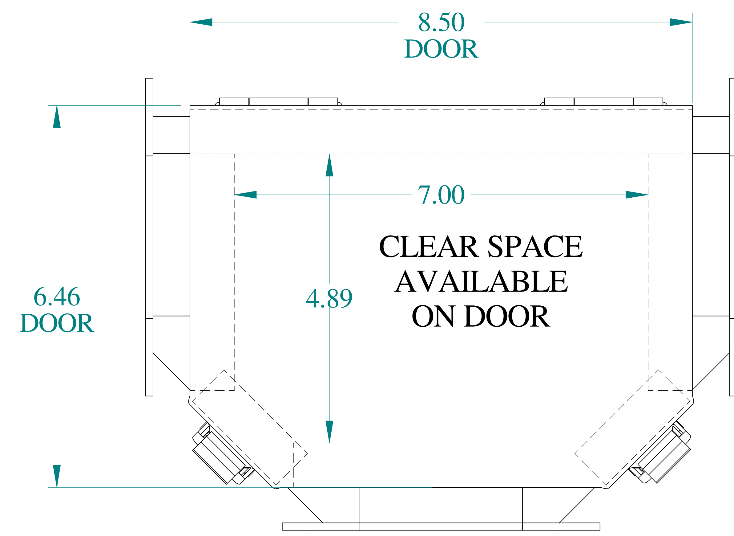
TOP VIEW
