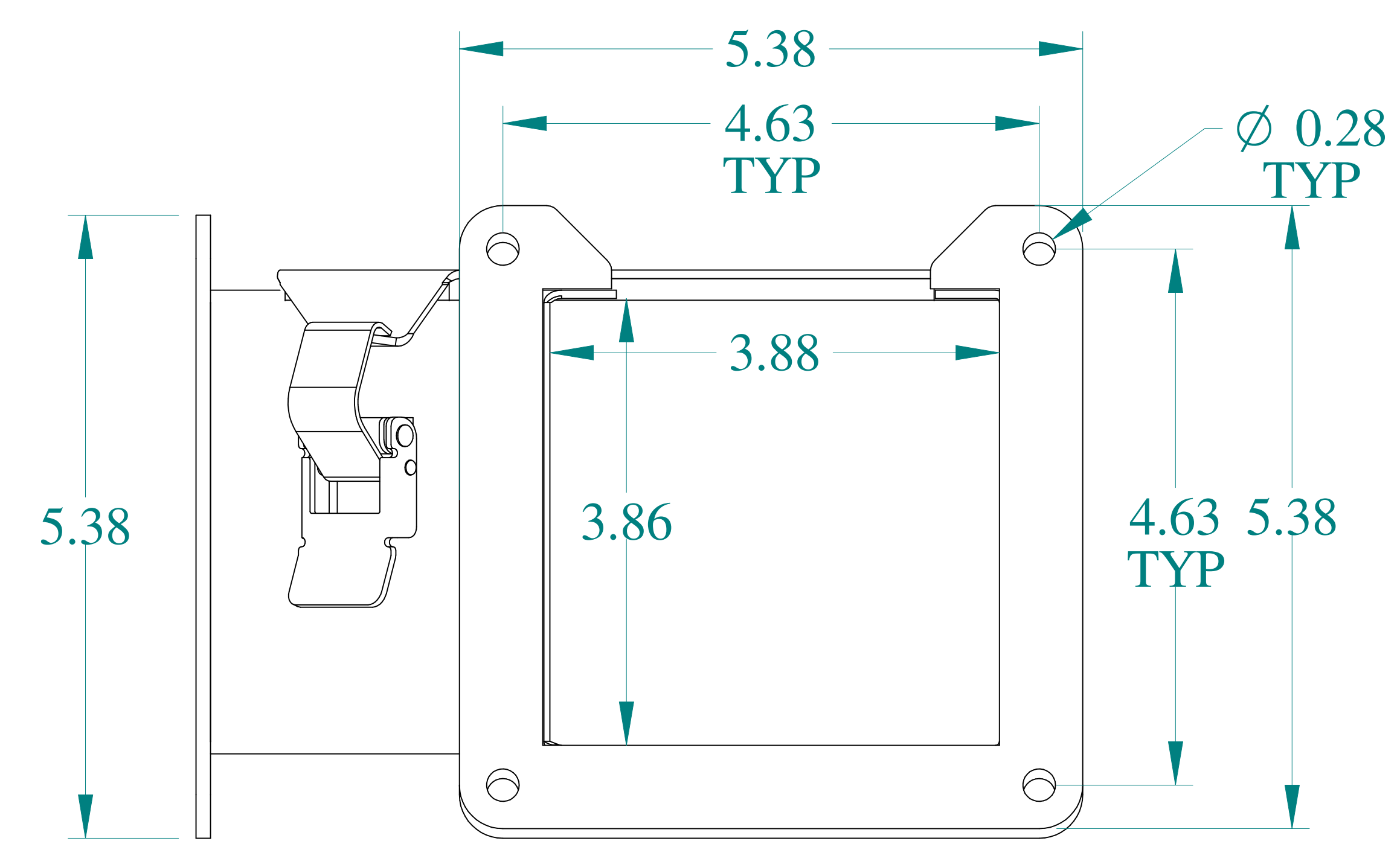
SIDE VIEW
