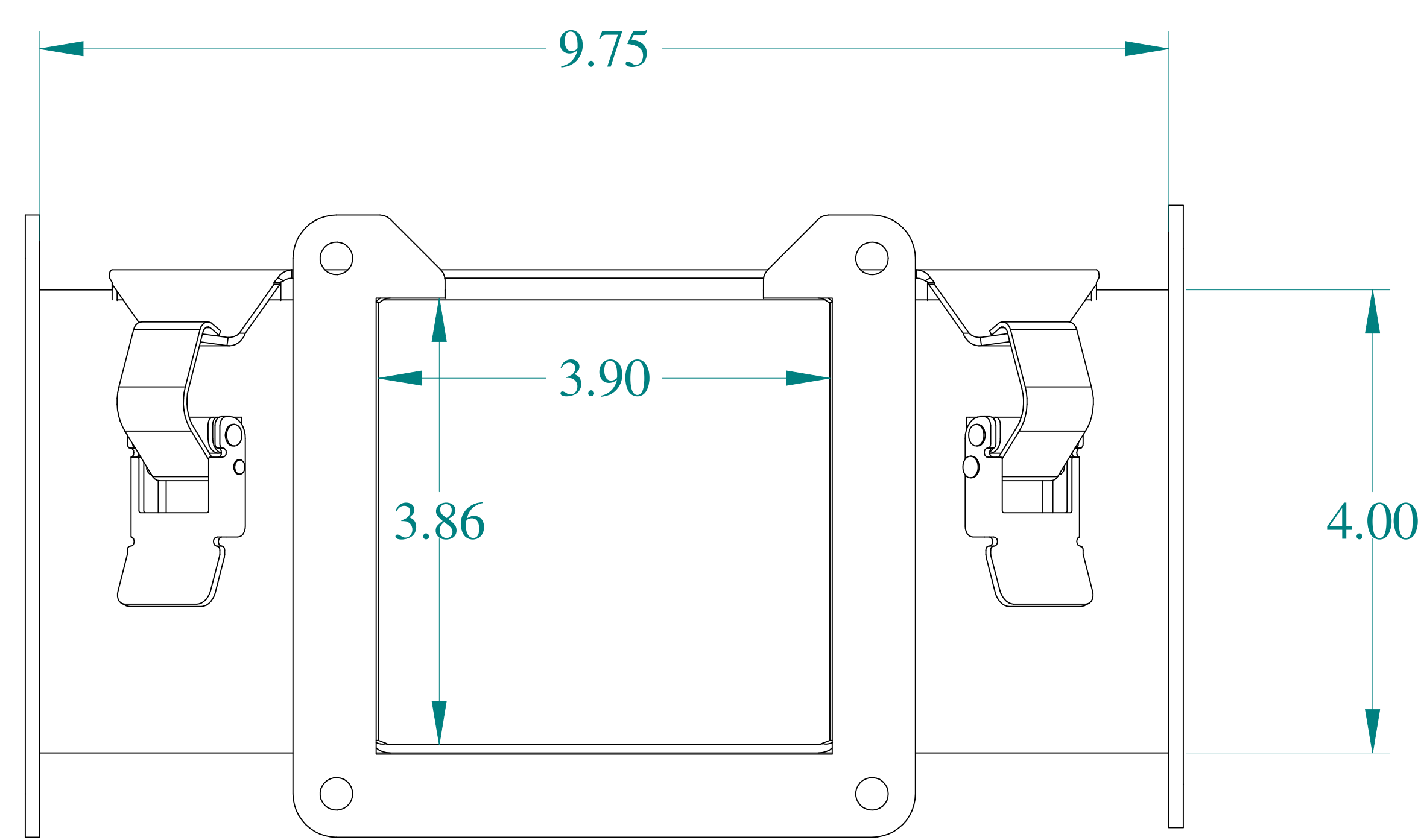
FRONT VIEW
