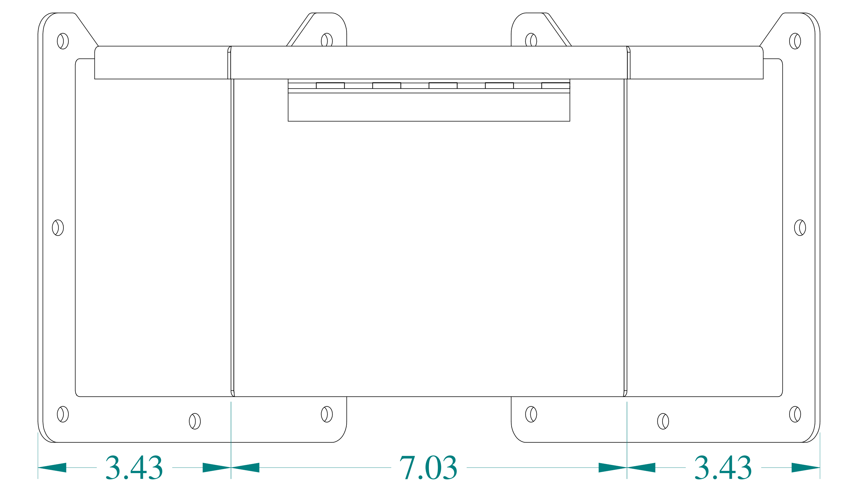
BACK VIEW
