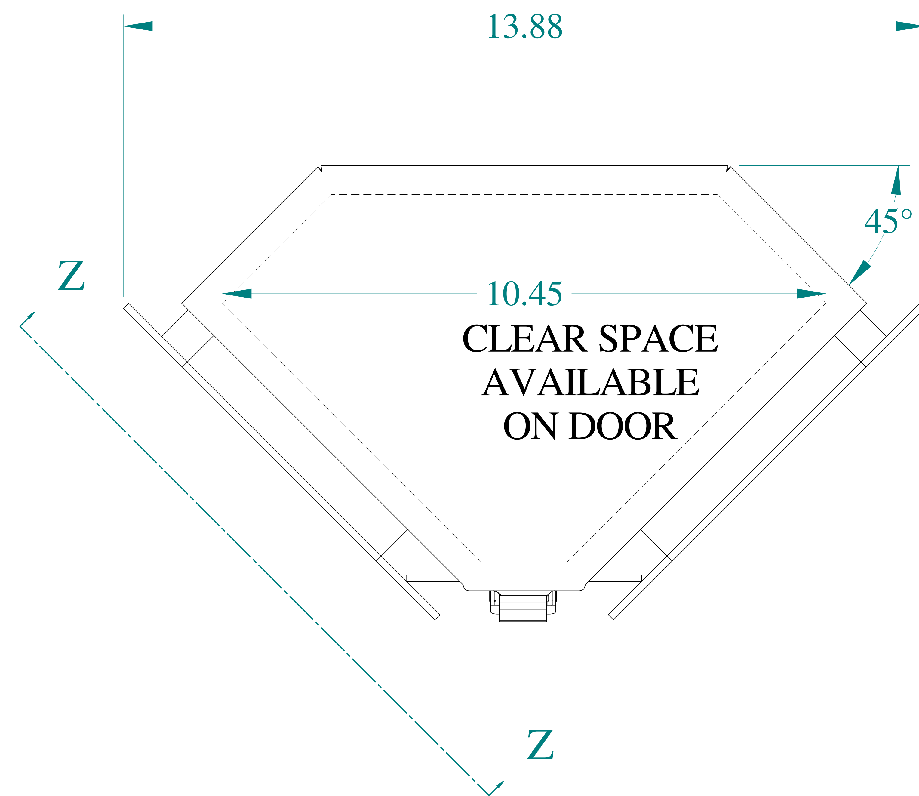
TOP VIEW
