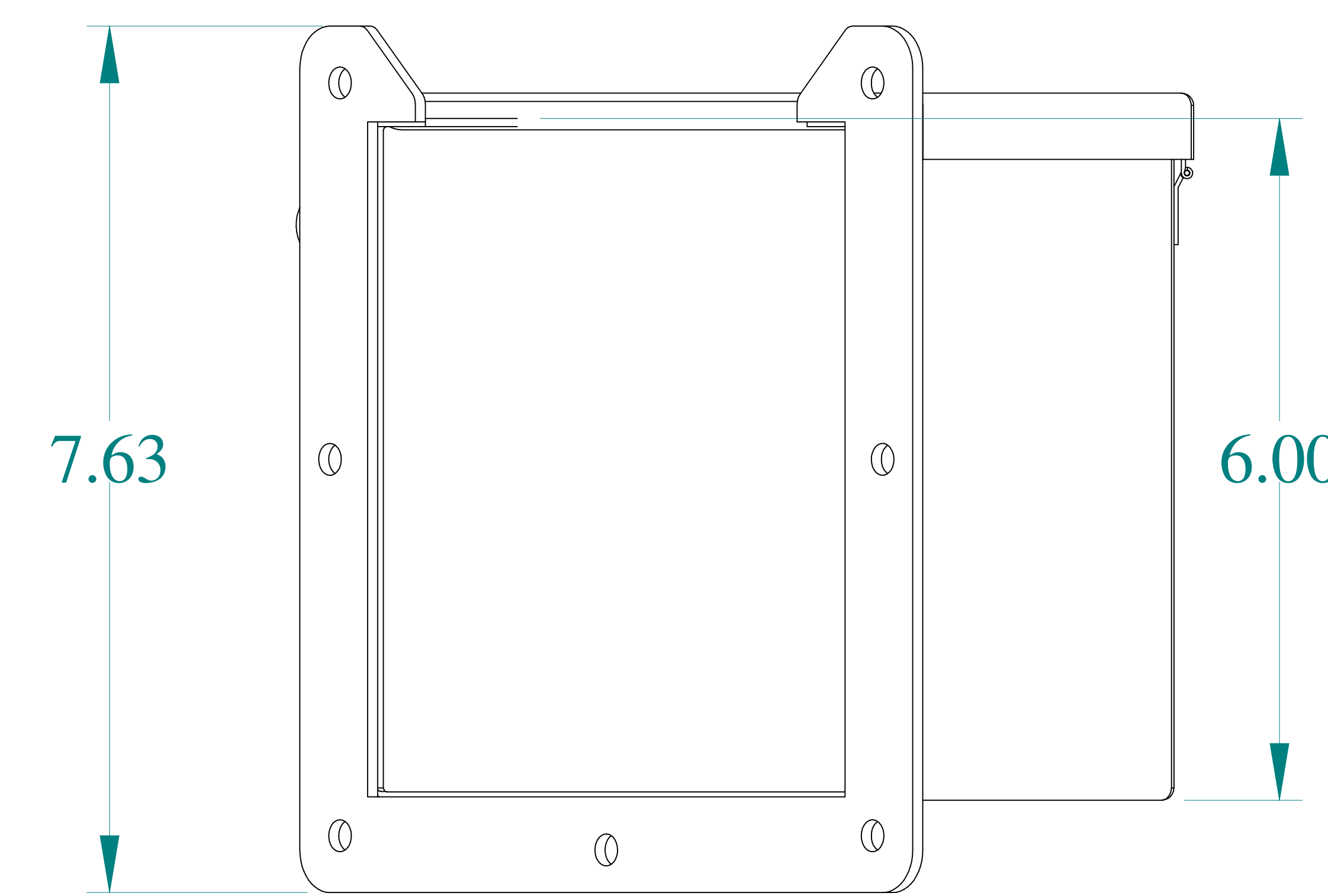
SIDE VIEW
